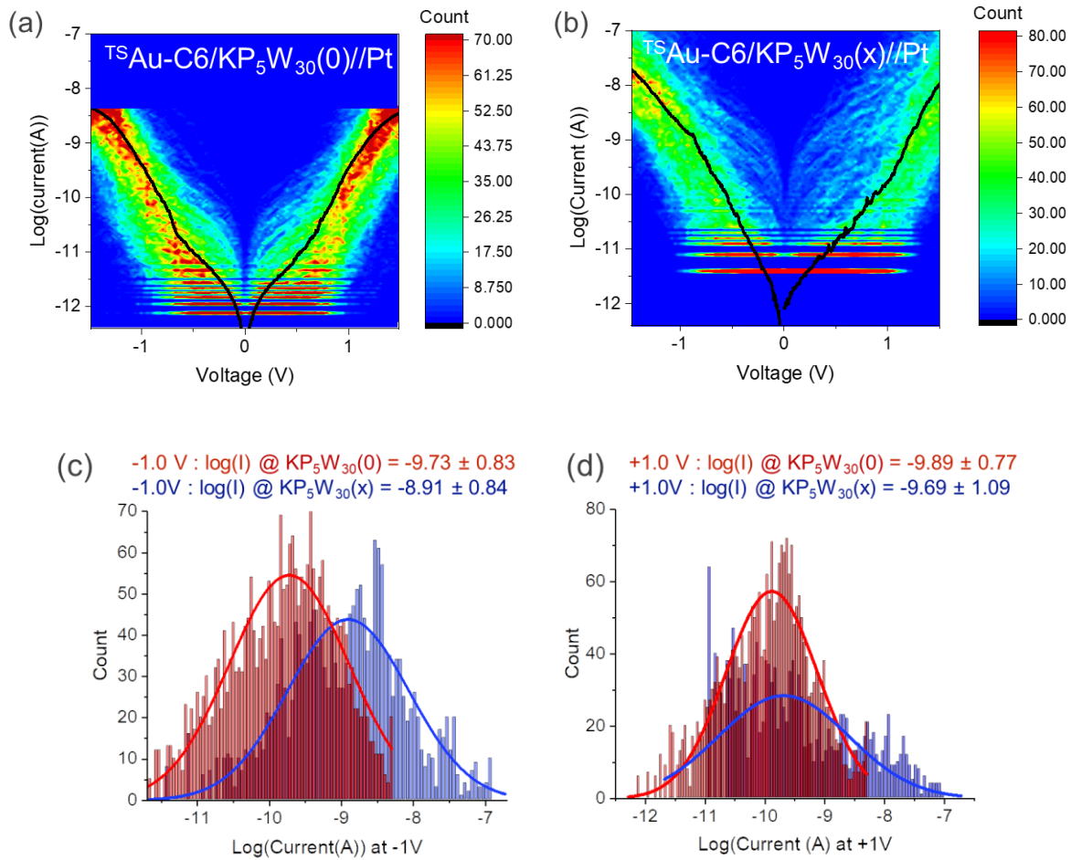
Figure 2.31. 2D histograms (heat maps) of I -Vs (loading force = 7.5 nN) in a semi- \log_{10} plot for (a) ^{TS}Au-C6/KP_5W_{30}(0)/Pt and (b) ^{TS}Au-C6/KP_5W_{30}(x)/Pt . The solid black lines are the mean \bar{I} -V curves. Histograms of the currents at (c) -1.0 V and (d) +1.0 V for the pristine (red bars) and reduced POM (blue bars) and fits by a log-normal distribution (the fitted log-mean value \pm log-standard deviation is indicated on the panels).
