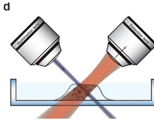
Fig. 1.4 Optical architecture of iSPIM. Figure modified from [27]
