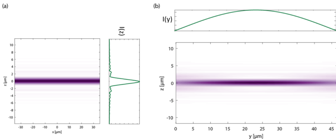
Fig. 2.7 LS generation using a square lattice. Cross-section of (a) the scanned beam intensity profile at the focus and (b) the excitation beam.
