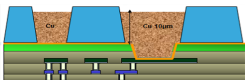
Figure 4.1: Scheme of a section of device after CuECD process.
