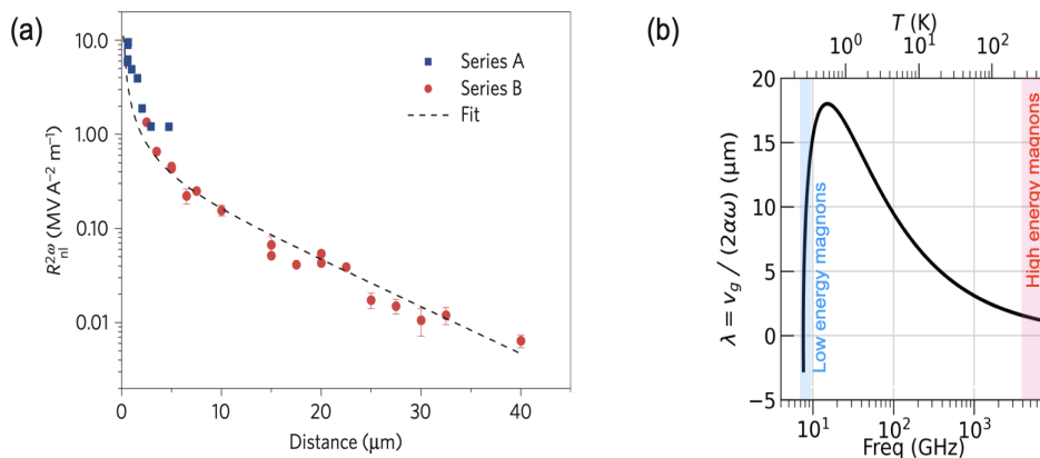
Figure 22: (a) Decay behavior of initially reported SSE signal. The solid line represents the exponential fit with 9 \mu decay length. The figure is taken from Ref. [52], the pioneer paper of this research field. (b) Calculated ballistic magnon relaxation length as a function of frequency. This shows the upper bound of characteristic decay of high-energy thermal magnons as 2 \mu\text{m} . \alpha = 4 \times 10^{-4} is used.
