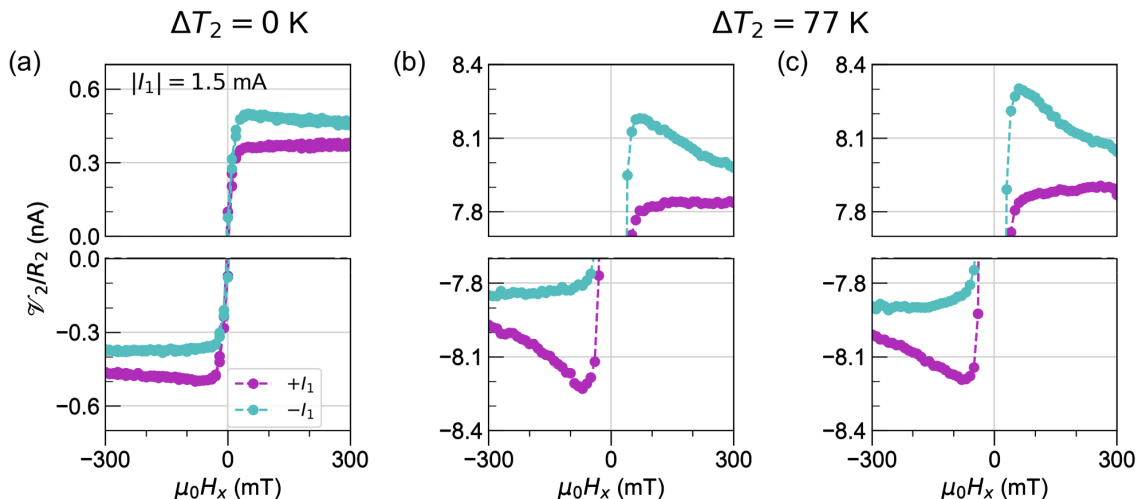
Figure 50: non-local magnon transport signal without and with local heating as a function of the external magnetic field. (a) Represents data without local heating \Delta T_2 = 0 K while (b) and (c) are data with local heating \Delta T_2 = 77 K, where the polarity of the current in the modulator I_3 is positive and negative, respectively. Note that the same range of vertical scale is maintained.
