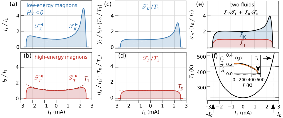
Figure 14: Dependence of the magnon transconductance on the spectral nature of propagating magnons. Panels (a) and (b) compare the predicted electrical variation of \mathcal{T}_s respectively for low-energy magnons (see Eq. (1.97), top panels), and for high-energy magnons (see Eq. (1.109), bottom panels), when H_x < 0 . Panel (f) displays the associated variation of T_1 = T_0 + \kappa R I_1^2 , the lattice temperature under the emitter. The current span exceeds I_c , the current bias that elevates T_1 to T_c , the Curie temperature. Panels (c) and (d) show the behavior when \mathcal{T}_s is renormalized by T_1 . Panel (e) shows the two-fluids fitting function: the independent sum of low-energy and high-energy magnon contributions with respective weight \Sigma_T and \Sigma_K . The insert (g) shows the temperature dependence of the magnetization M_T as measured by vibrating sample magnetometry (cf Fig. 31), and the solid line is a fit with the analytical expression M_T \approx M_0 \sqrt{1 - (T/T_c)^{3/2}} , with \mu_0 M_0 = 0.21 T and T_c = 550 K.
