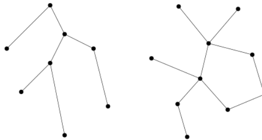
Figure 1.9: On the left-hand side, a tree with 4 leaves; on the right-hand side a graph which is not a tree as it contains a C_5 .
