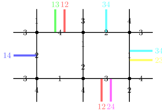
Figure 4.10: The border coloring does not extend, since inside the fragment there are no sources of swap lines, and the border is crossed by an odd number of swap lines of certain types.
