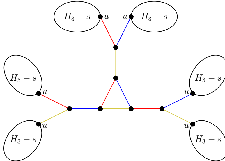
Figure 3.5: A graph G with maximum degree 3 and \chi_c(G)' > \chi'(G) . For any 3-edge coloring, there are two edges of type su colored 3 ‘entering’ a copy of H_3 .
