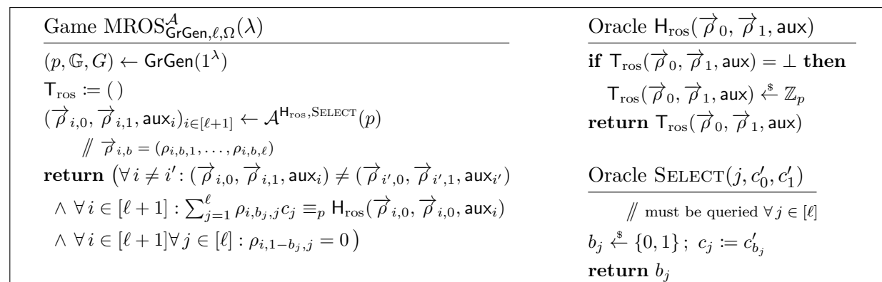
Figure 6.2: The modified ROS problem.
