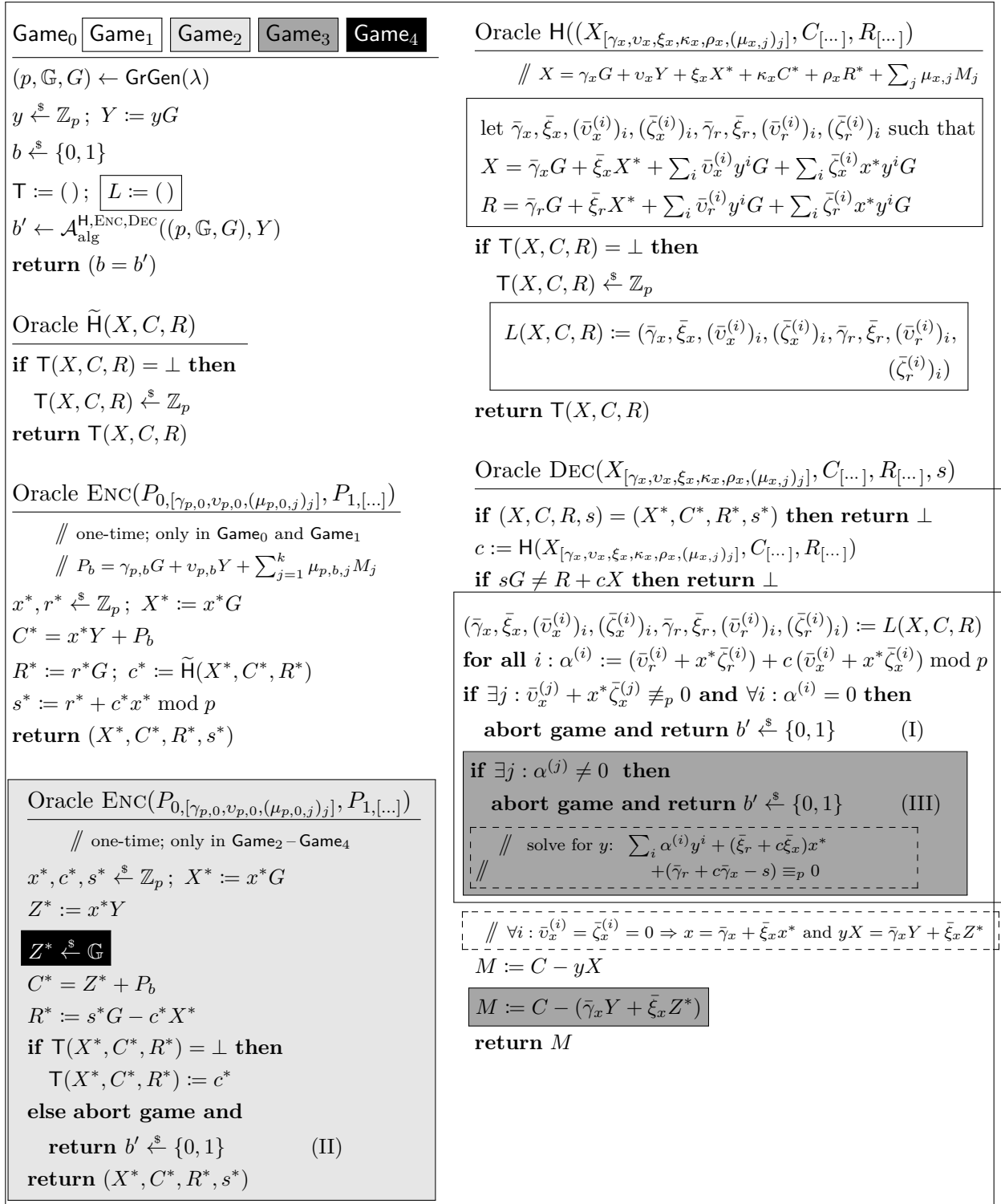
Figure 7.4: The IND-CCA2 game for the Schnorr-Signed ElGamal scheme (Game 0 ) and games Game 1 –Game 4 used in the proof. The comments in dashed boxes show how the DL reduction simulates Game 3 without knowledge of y .
