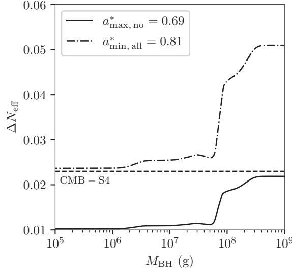
Figure 4.18: Low and high cut-off values for CMB-S4 exclusion (same limit as in Fig. 4.17), corresponding to a_{\text{max}, \text{no}}^* = 0.69 and a_{\text{min}, \text{all}}^* = 0.81 (solid and dot-dashed respectively). [taken from [584]]
