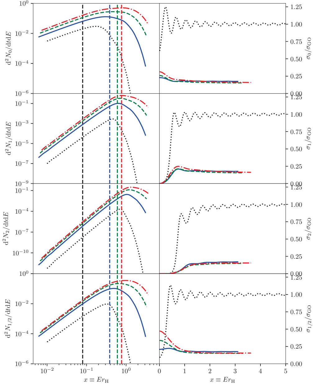
Figure 2.11: Primary spectra ( left ) and cross-sections ( right ) for spins 0, 1, 2 and 1/2 for a HDBH with n = \{2, 4, 6\} (resp. solid blue, dashed green, dot-dashed red) compared to the SBH (dotted black). The vertical lines represent T_{HD} . [taken from [150]]
