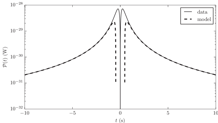
Figure B.6: Example of a light curve for a speed v = 0.001 c , impact parameter b = 10^3 m, sail area \mathcal{S} = 1 m 2 , and P9 parameters M = 5 M_{\oplus} and a^* = 0 (solid line). The approximation of Eq. (B.11) leads to the dashed line. [taken from [663]]
