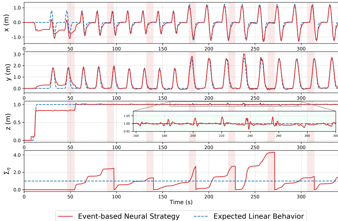
Figure IV.3: Simulation scenario (I): circles motions. This scenario illustrates the performance criterion. Red areas represent learning and re-learning processes.
