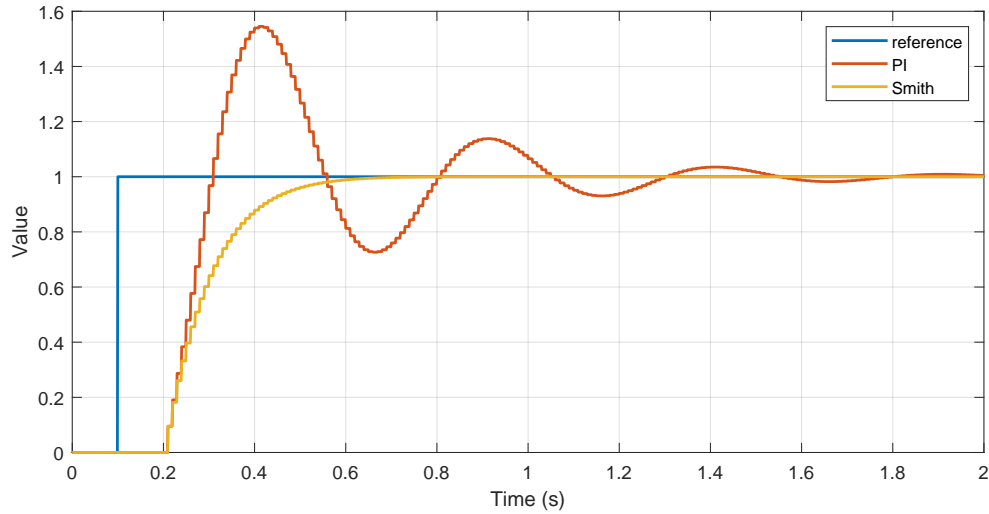
Figure II.11: Example of Smith predictor improvement.
