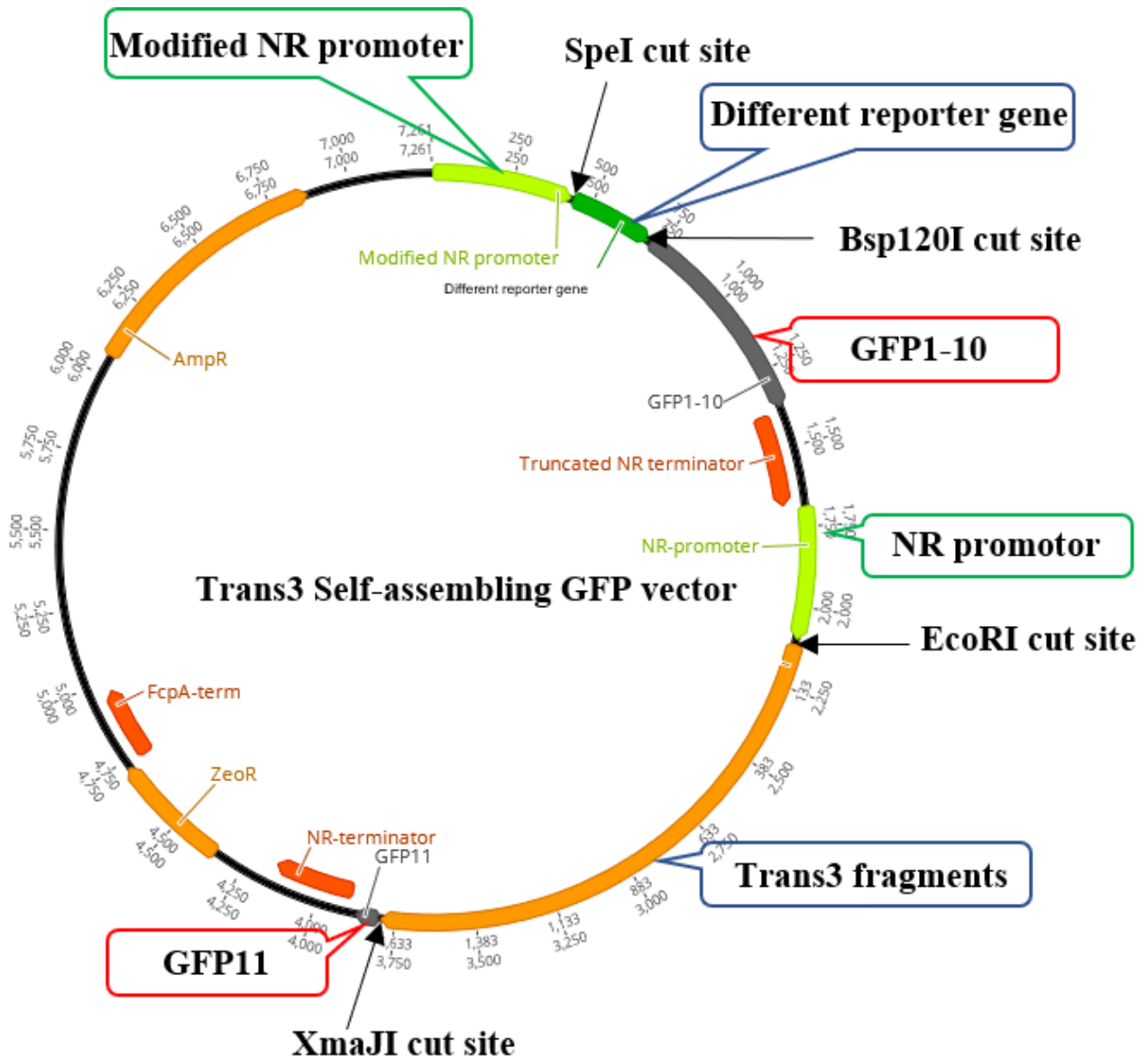
Figure 3.5 pPha 2x NR Trans3 self-assembling GFP vector structure. Reporter genes were incorporated upstream of the GFP1-GFP10 regions; and different Trans3 fragments were introduced upstream of GFP11. NR promoter and terminator sequences, resistance marker genes, and restriction cut sites used for cloning are shown.
