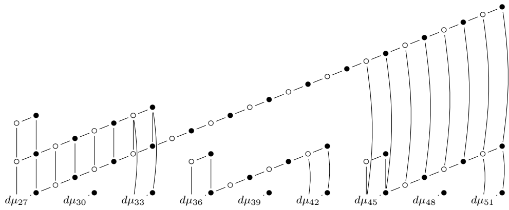
Figure 6.3: T_3^! for p = 3 .
