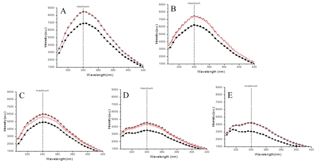
Figure S2. Intrinsic fluorescence. (A) pure CMs, (B) pure pea protein, (C) 80:20, (D) 50:50, (D) 80:20. Black symbols stand for gels before HIUS treatment, colored full symbols stand for samples treated with HIUS with route 1, and colored empty symbols stand for samples treated with HIUS with route 2.
