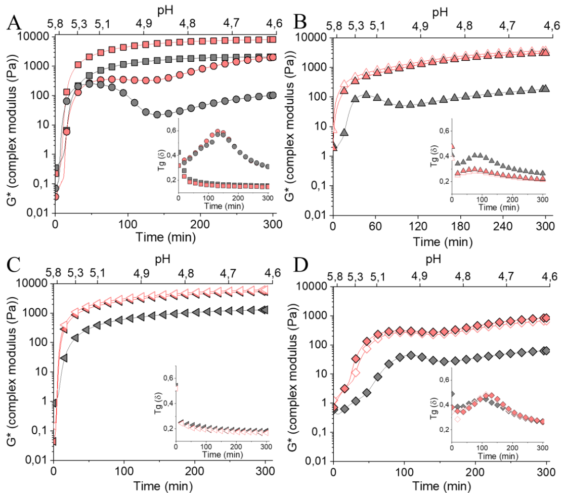
Figure 4. Complex modulus G^* in the function of time after addition of GDL. (A) pure CMs (● ●) and pure pea protein (■ ■). (B) 50:50, (C) 20:80, and (D) 80:20. The inserted graphs are the loss tangent plots in the function of time. Black symbols stand for suspensions before HIUS treatment. Colored full symbols stand for samples treated with HIUS with route 1 whereas colored empty symbols stand for samples treated with HIUS with route 2.
