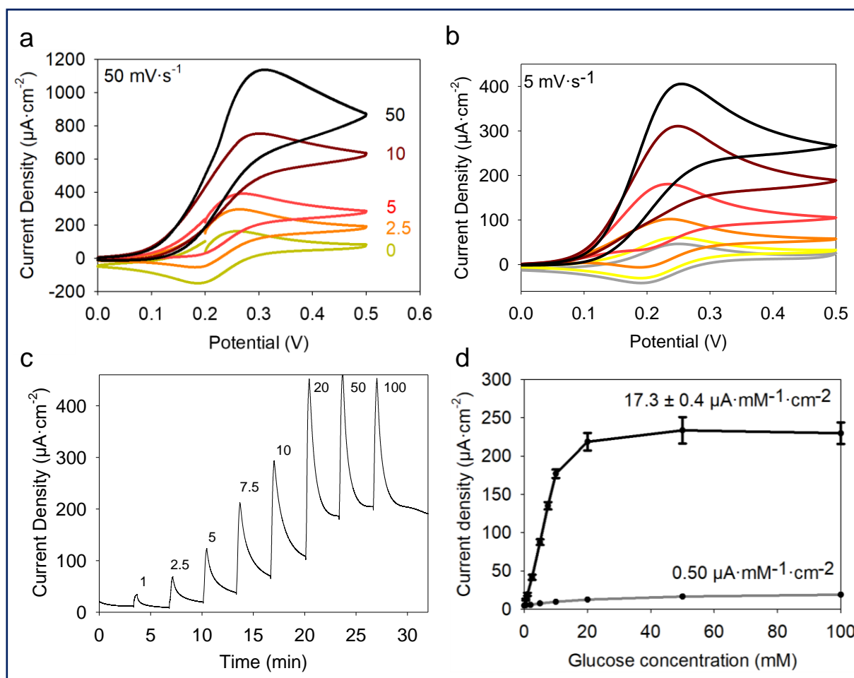
Figure 3.9: Cyclic voltammograms, performed at a scan rate of (a) 50 \text{mV}\cdot\text{s}^{-1} and (b) 5 \text{mV}\cdot\text{s}^{-1} of GOx/TA@AuNPs coating in contact with 0 to 100 mM of glucose solution prepared in 0.5 mM FcOH/10 mM PBS. (c) Chronoamperometric response at 0.25 V upon addition of different glucose concentration. (d) Average current density, measured at 0.25 V, as a function of the glucose concentration of GOx/TA@AuNPs (black curve) and GOx/TA (grey curve) coatings. The average and error bars of GOx/TA@AuNPs coatings were evaluated on six independent experiments.
