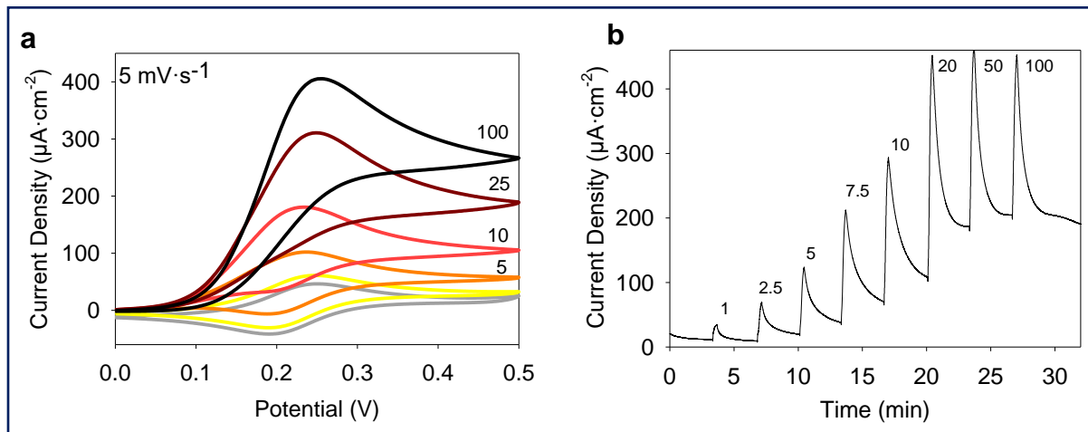
Figure 2.16: Illustration of the biocatalytic characterization of \text{GOx/NPs} coatings with (a) cyclic voltammetry and (b) chronoamperometry at 0.25V for different glucose concentration from 0 to 100 mM in presence of 0.5 mM FcOH.
