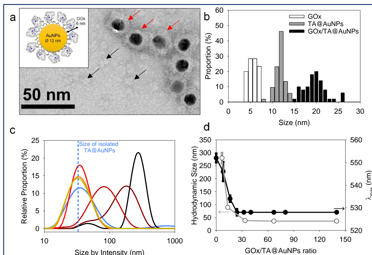
Figure 3.2. Characterization of GOx/TA@AuNPs complexes. (a) Typical TEM image, obtained after uranyl acetate staining at 2%. Red arrows show GOx/TA@AuNPs and black arrows some extra GOx in the supernatant. Inset is the illustration of GOx/TA@AuNPs complexes. (b) Size distribution of GOx, TA@AuNPs and GOx/TA@AuNPs determined from TEM images. (c) Hydrodynamic size in presence of NaCl 1M at GOx/TA@AuNPs molar ratio of 0 (black), 13.4 (dark red), 34 (red), 67 (orange), 140 (yellow) and in absence of NaCl (blue). (d) Flocculation test upon addition of 1 M NaCl in the GOx/TA@AuNPs suspension with the hydrodynamic size previously measured (white circle) and the maximum absorption wavelength of aggregates (black circle) as a function of GOx/NPs molar ratio.
