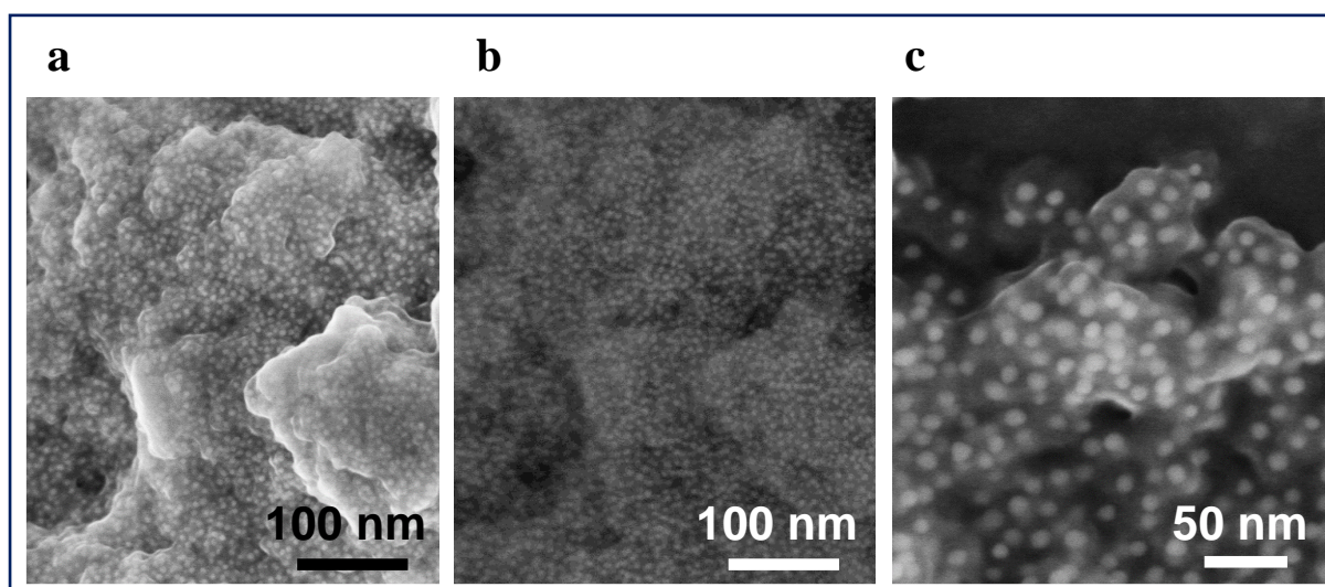
Figure 5.7: SEM micrographs of a typical HRP/NP12/GA coating on PU-FLG, obtained at a working distance of 3 mm using an electron beam of 5 kV and 10 \mu A, with the secondary electrons at different magnification (a,c) and the same area was then observed with back-scattered electron (b).
