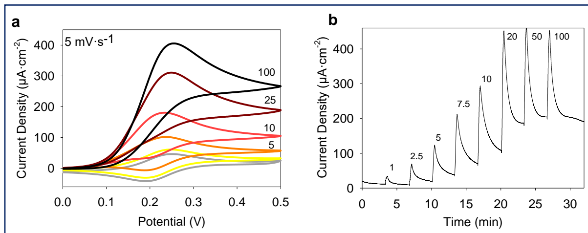
Figure 2.16: Illustration of the biocatalytic characterization of \text{GOx/NPs} coatings with (a) cyclic voltammetry and (b) chronoamperometry at 0.25V for different glucose concentration from 0 to 100 mM in presence of 0.5 mM FcOH.
