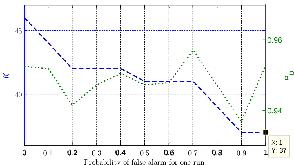
Figure 6.5 Required number of non-coherent summations for Approach 3
