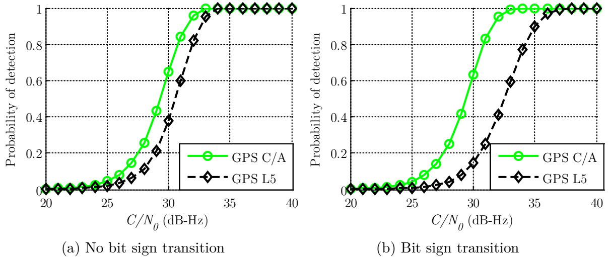
Figure 4.32 Probabilities of detection when considering or not bit sign transitions on T_I = 20 ms and T_C = 1 ms for GPS L1 C/A and GPS L5
