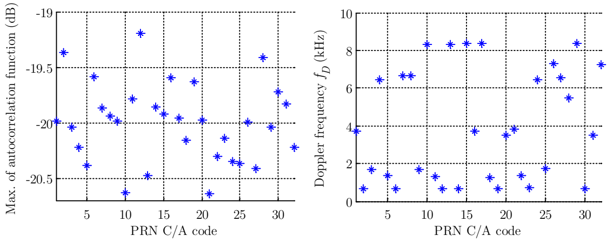
(a) Maximum of the autocorrelation function per PRN C/A code
