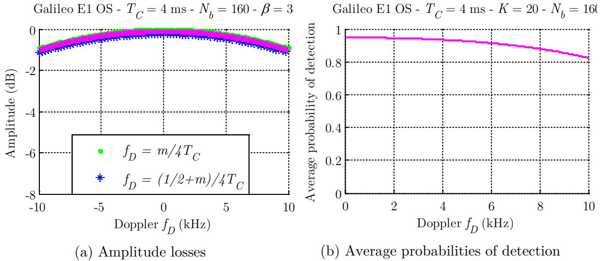
Figure 5.15 Losses due to the incoming Doppler frequency after improvements
