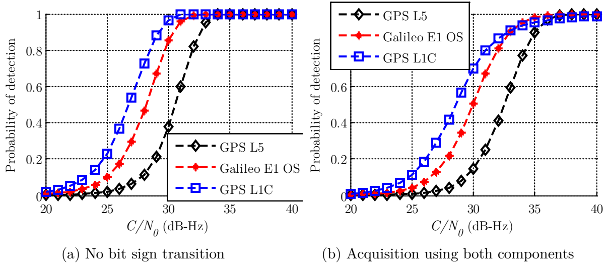
Figure 4.31 Probabilities of detection for T_I = 20 ms when considering or not bit sign transitions (modernized GNSS signals)
