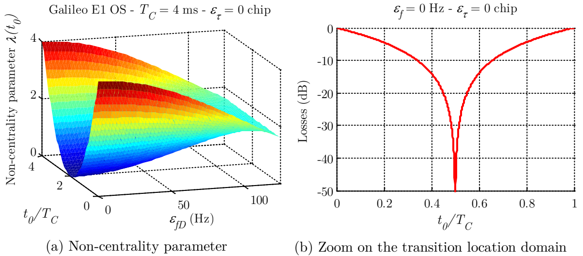
Figure 4.17 Non-centrality parameter in presence of a bit sign transition
