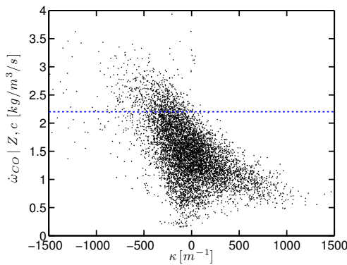
(b) CO source term.
