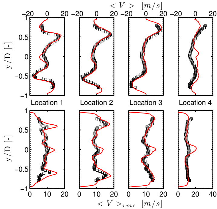
Figure 9.6: SGT-100/Case A: Transverse profiles of mean (top) and rms (bottom) transverse velocity at the four measurement locations. Comparison between LES (-) and experiments ( \square ).
