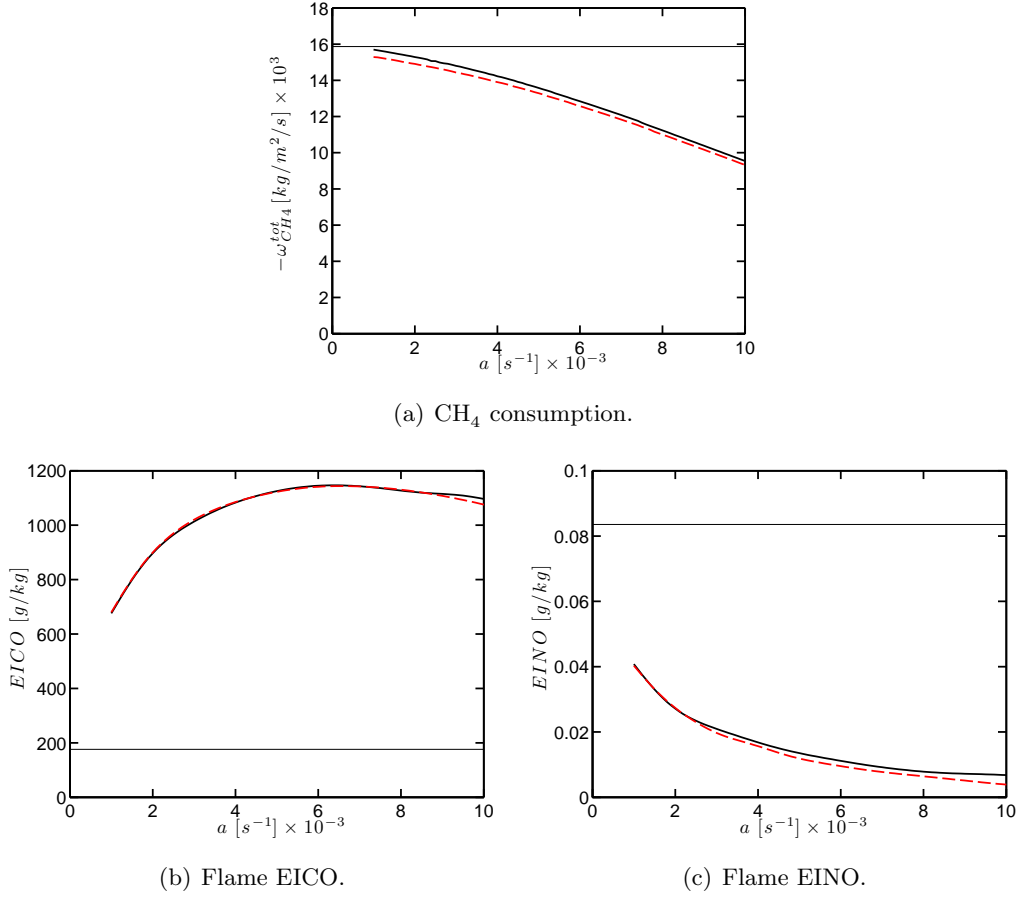
Figure 9.15: One-dimensional strained premixed flames in SGT-100/Case A conditions at \phi = \phi_{glob} . Comparison of the response to strain of global quantities between GRI 2.11 (—), ARC_22_GRI211 (---). The horizontal lines correspond to the unstrained values for GRI 2.11.
