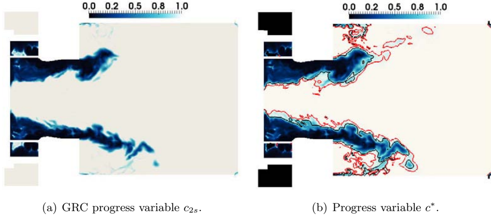
Figure 9.28: SGT-100/Case A - NOMAGT: Instantaneous fields of a) progress variable from 2-step chemistry c_{2s} and b) progress variable c^* with c_{2s} = 0.98 isocontour (black) and c^* = 0.98 isocontour (red).
