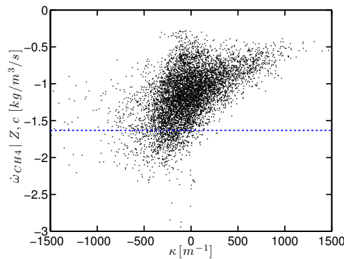
(a) CH_4 source term.
