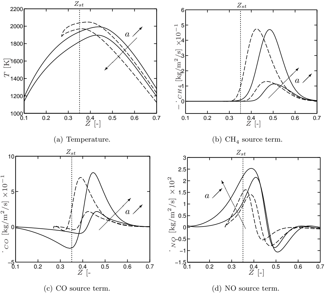
Figure 8.14: Laminar counterflow flames with ARC_22_GRI211. a) Temperature, b) CH 4 source term, c) CO source term and d) NO source term vs mixture fraction. Comparison of coflow (—) and pilot (---) counterflow flames at strain rates a = 60 \text{ s}^{-1} and 270 \text{ s}^{-1} .
