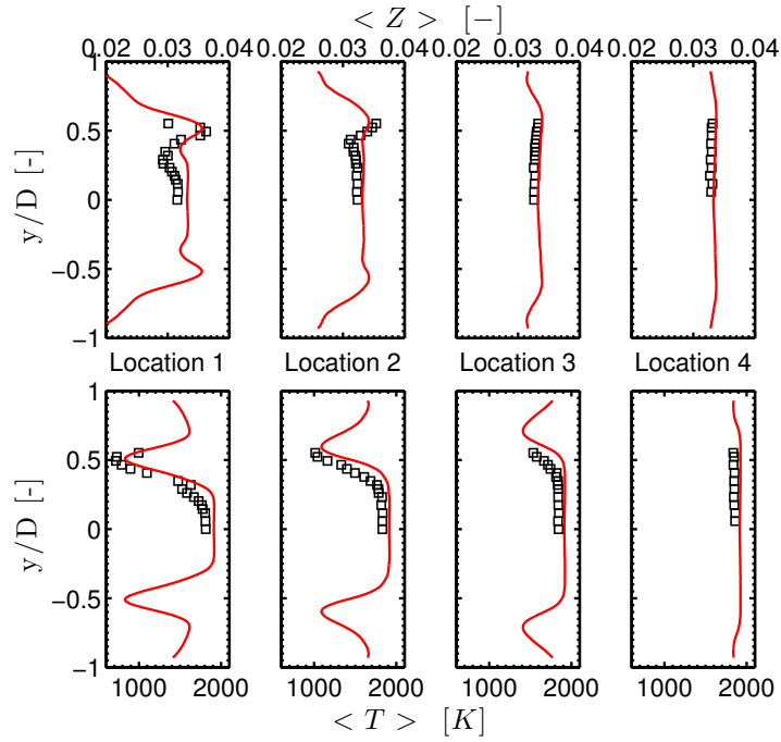
Figure 9.32: SGT-100/Case B: Transverse profiles of mean mixture fraction (top) and temperature (bottom). Comparison between LES (—) and experiments (□).
