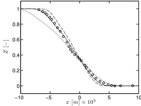
Figure 7.12: Measured profiles of mixture fraction ( \circ ) from Barlow et al. [11]. Comparison with counterflow flames at global strain rate a = 5\text{s}^{-1} ( \cdots ), 10\text{s}^{-1} ( \text{—} ) and 15\text{s}^{-1} ( \text{--} ).
