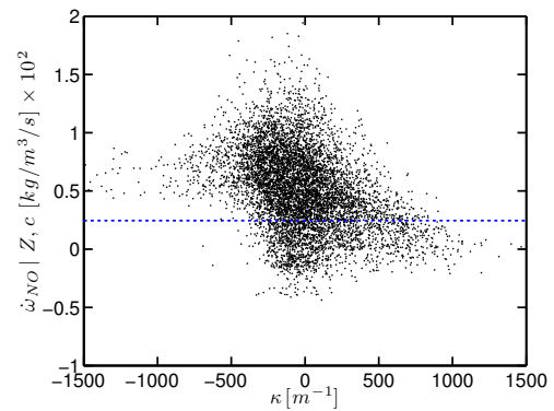
(c) NO source term.
