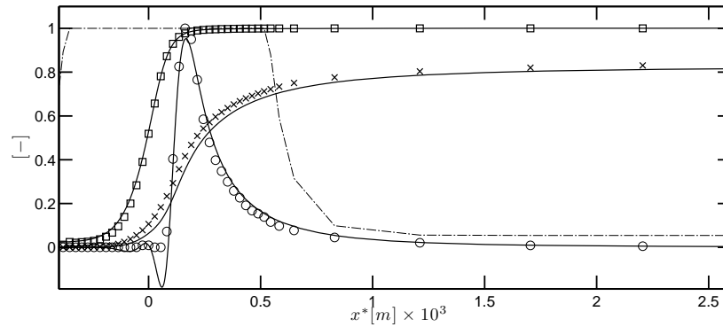
Figure 5.11: Comparison of the NOMAGT model with detailed chemistry on a one-dimensional premixed methane-air flame at \phi = 1.4 with adjusted flame speed: thickening factor ( -\cdot- ), progress variable c^* ( \square ), NO mass fraction from NOMAGT ( \times ) and NO source term from NOMAGT ( \circ ). The continuous lines corresponds to the results obtained for the detailed mechanism with Cantera.
