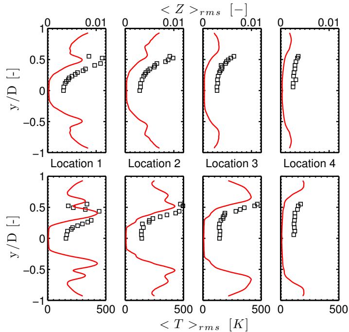
Figure 9.33: SGT-100/Case B: Transverse profiles of rms mixture fraction (top) and rms temperature (bottom). Comparison between LES (—) and experiments (□).
