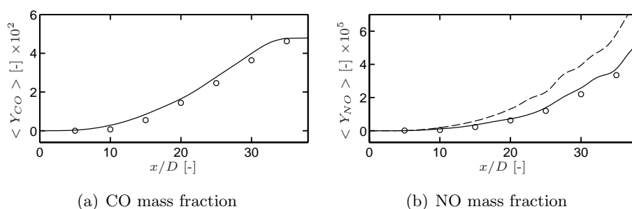
Figure 8.10: Sandia flame D: Axial profiles along the centerline of a) mean CO mass fraction for ARC_22s (—) and b) NO mass fraction for ARC_22_GRI211 (---) and ARC_22_GRI30 (- -). Experimental data \circ .
