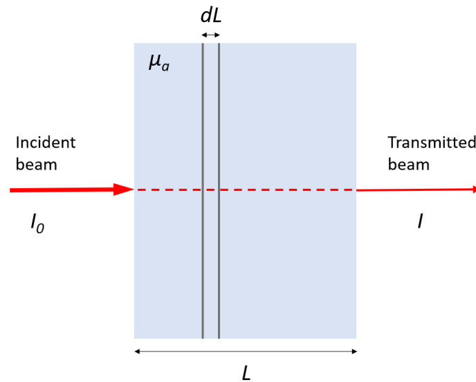
Figure II.2 – Light propagation through an absorbing medium.
