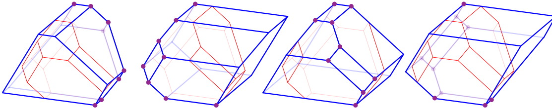
Figure 6: Four realizations of the 3-dimensional permutahedron \Pi_3 sitting inside an associahedron. The left-most associahedron is the Loday's associahedron \text{Asso}_3 . Illustration from [PSZ23, Figure 7(Top)].
