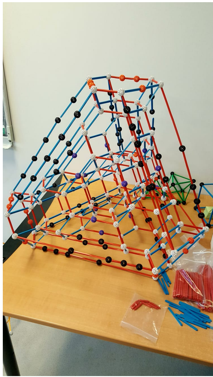
Figure 5: The permutahedra for dimensions d = 0, 1, 2, 3 and 4 . Up to dimension 3 , the vertices are labelled by the permutations, and each edge is colored according to its class of parallelism (for example, going through a blue edge amounts to exchanging the values 1 and 2 ). The 4 -dimensional permutahedron have been made with Zometool, the vertices correspond to the white nodes.
