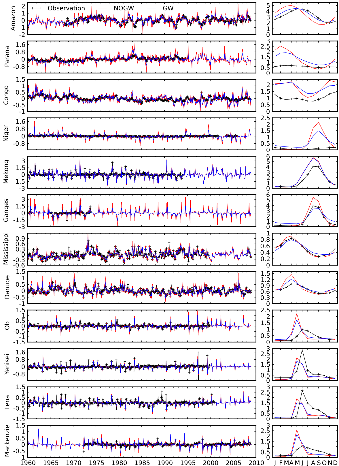
FIG. 5.5: Basin-scale comparison (mm day -1 ) between the (right) annual cycle and (left) monthly-mean anomalies of simulated and observed discharges. Statistics for each station are shown in Table 5.3
