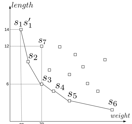
Figure 3: Pareto Front
