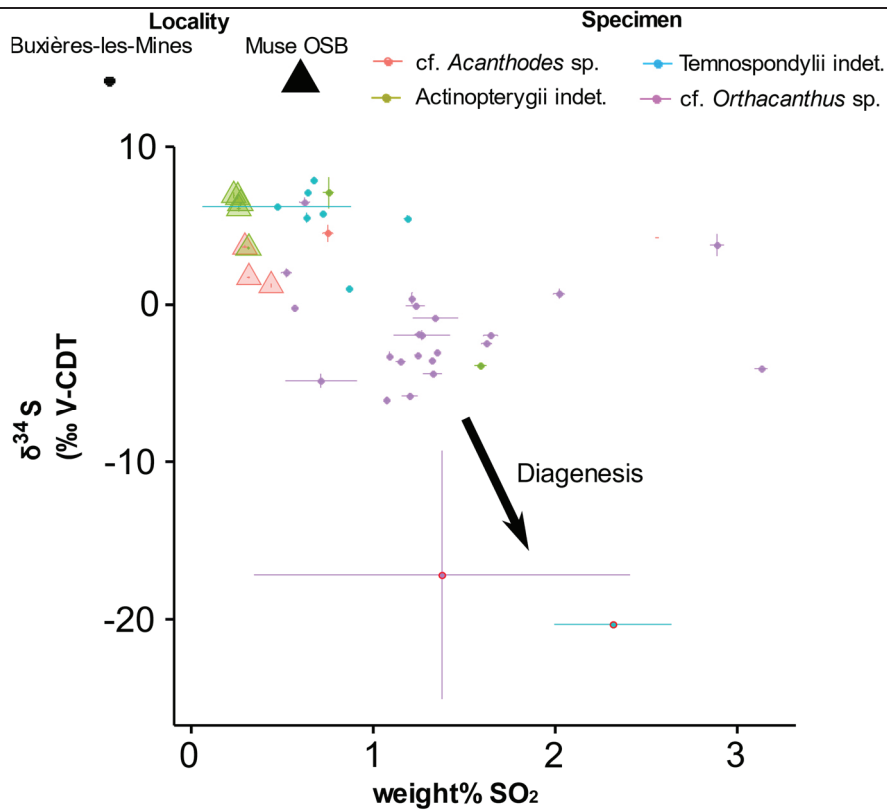
Figure 88. The sulfur isotope composition ( \delta^{34}S ) plotted against the sulfur content (weight% SO_2 ).
