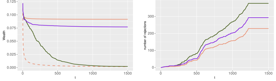
Figure A.1: Comparison with DS. Left: nominal wealth for OB (dashed orange curve), effective wealth for OB (solid orange curve), effective wealth for \rho OB (solid green curve) and effective wealth for DS (solid purple curve), plot similar to Figure 2.1. Right: rejection numbers, cumulated over time, for the same procedures (same color code). Both plots are computed from the male IMPC data.
