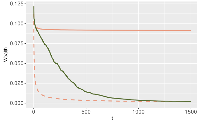
Figure 2.1: Nominal wealth for OB (dashed orange curve), effective wealth for OB (solid orange curve) and effective wealth for \rho OB (solid green curve) for the male mice from the IMPC data (see Section 2.5.3 for more details).
