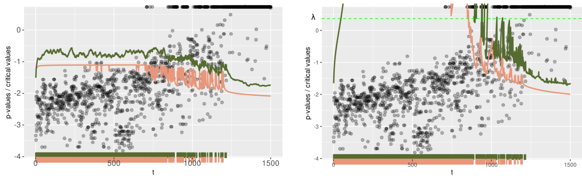
Figure A.12: Same as Figure 2.8 for female mice of IMPC data (see Section 2.5.3).
