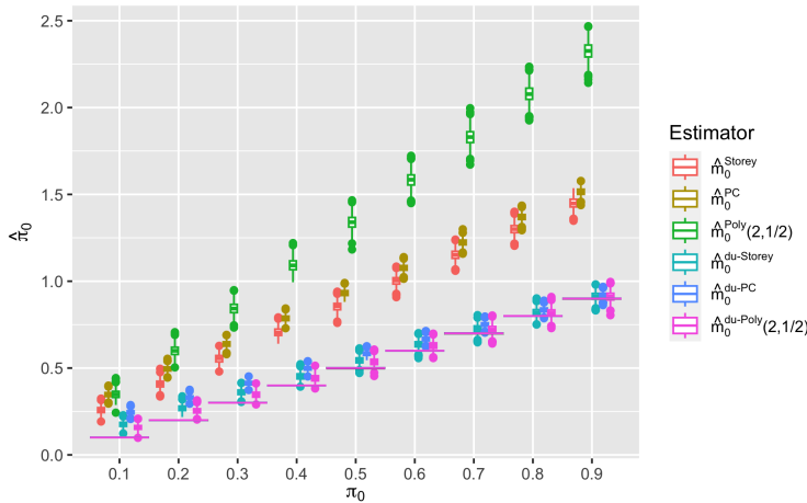
Figure 4.3: Comparison between base estimators \hat{m}_0^{\text{Storey}} , \hat{m}_0^{\text{PC,new}} and \hat{m}_0^{\text{Poly}}(2, 1/2) and their standard discrete rescaled versions on simulated data.
