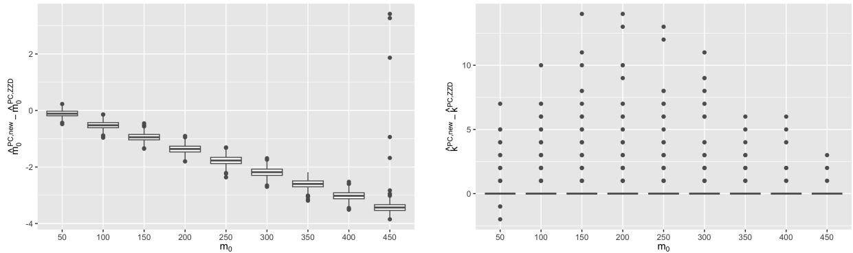
Figure C.1: Box plots for the difference between \hat{m}_0^{\text{PC,new}} and \hat{m}_0^{\text{PC,ZDD}} for point estimation (left) and rejection numbers for the plug-in BH procedures (right) against a range of true m_0 = 50, 100, \dots, 450 .
