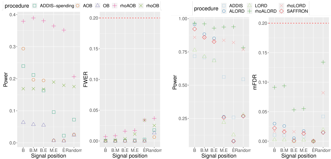
Figure 2.5: Power and type I error rates of the different considered OMT procedures versus positions of the signal: at the beginning (B), the end (E), half at the beginning and half in the middle of the stream (BM), half at the beginning and half at the end of the stream (BE), half in the middle and half at the end of the stream (ME), and taken uniformly at random (Random).
