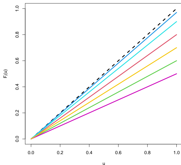
Figure 1.3: Examples of F_i functions in the constrained weighting setting (colored solid lines) and standard Uniform c.d.f (black dashed line).
