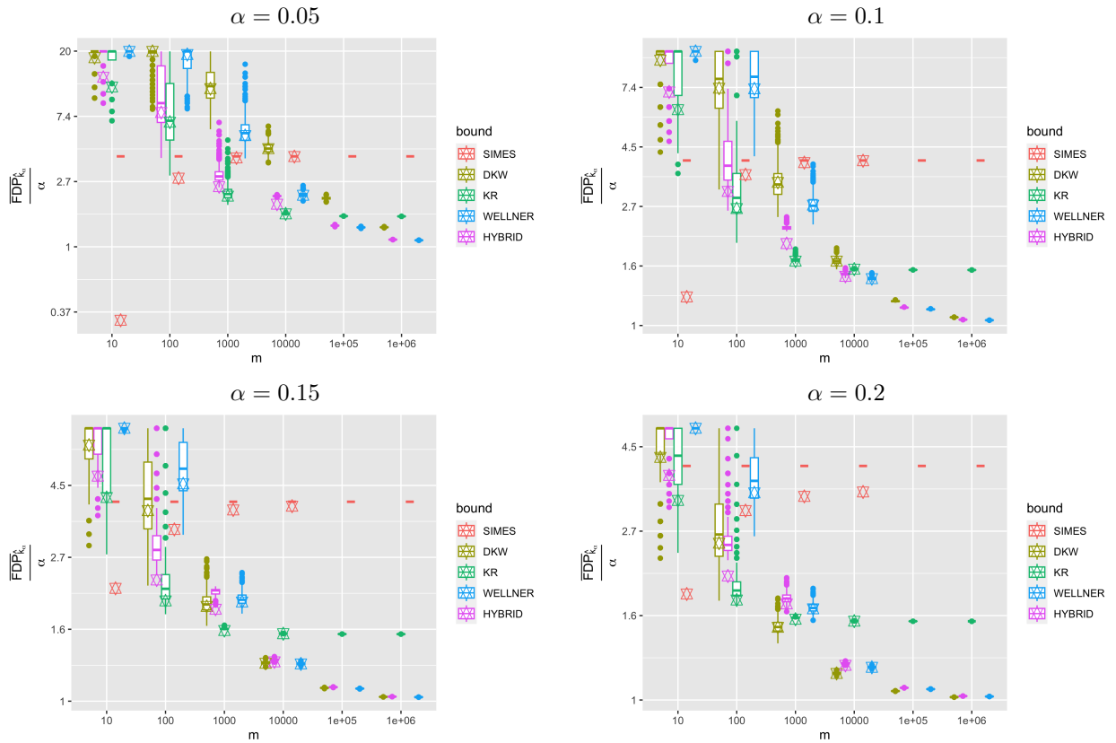
Figure B.2: Figure 3.1 where we have superposed in each case the (median of the) interpolated bounds (star symbols). Top- k dense case ( \pi_0 = 0.5, \mu = 1.5 ).
