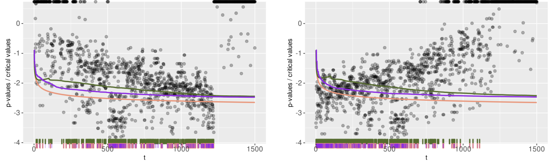
Figure A.2: Critical values of OB (orange), \rho OB (green) and DS (purple) for the IMPC data (left panel is for male, right panel is for female).
