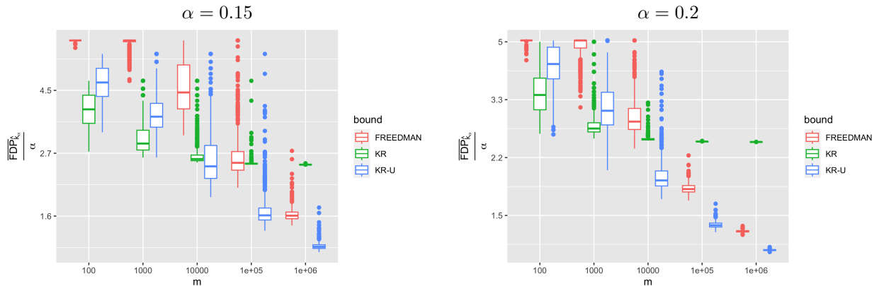
Figure 3.8: Pre-ordered sparse ( \beta = 0.25 ) knockoff setting with BC procedure (i.e., LF procedure with s = \lambda = 0.5 ).
