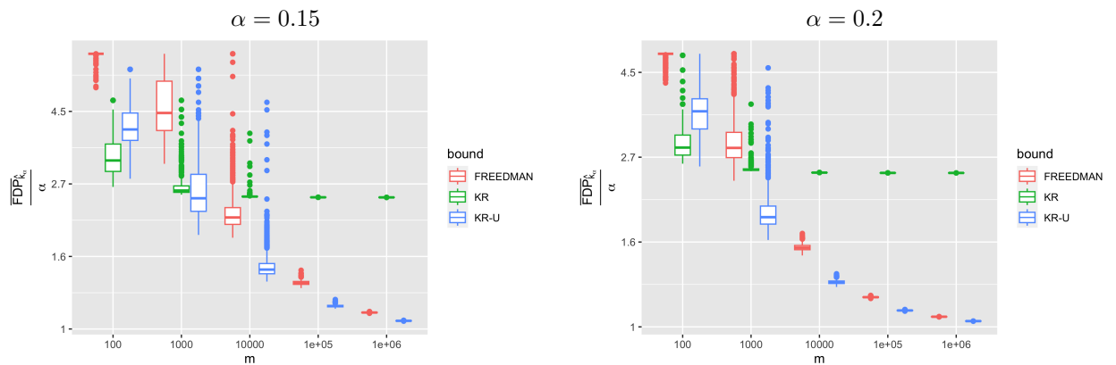
Figure 3.7: Pre-ordered dense ( \beta = 0 ) knockoff setting with BC procedure (i.e., LF procedure with s = \lambda = 0.5 ).
