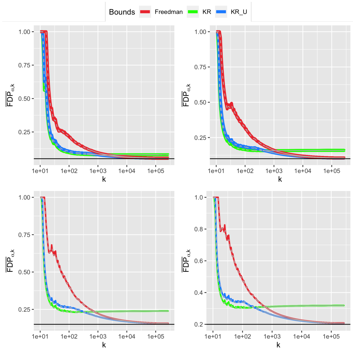
Figure 3.9: Online FDP envelopes for LORD applied on IMPC data for four values of \alpha \in \{0.05, 0.1, 0.15, 0.2\} (horizontal black bars). The interpolated bounds are displayed for each procedure as a gray dashed line.
