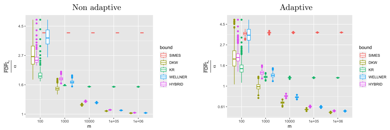
Figure 3.3: Top- k dense case with nonadaptive bounds (left) and adaptive bounds (right) ( \pi_0 = 0.5 , \alpha = 0.2 ).
