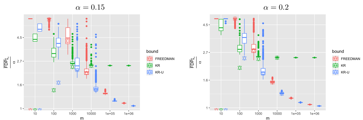
Figure B.7: Figure 3.7 where we have superposed in each case the (median of the) interpolated bounds (star symbols). Pre-ordered dense ( \beta = 0 ) knockoff setting with BC procedure (i.e., LF procedure with s = \lambda = 0.5 ).
