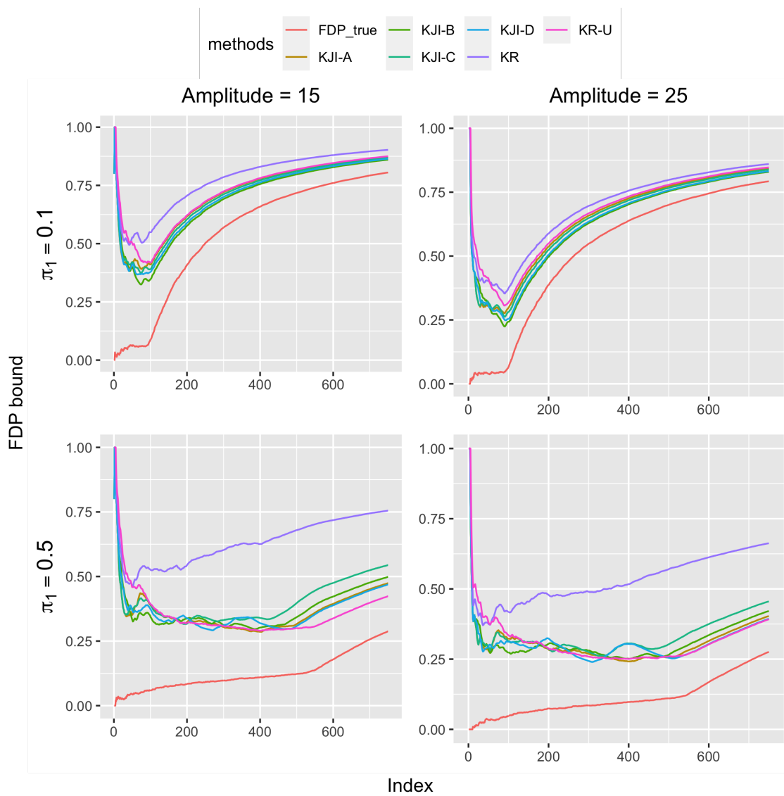
Figure 3.10: Comparing the envelope \widetilde{\text{FDP}}_k^{\text{KR-U}} , k \geq 1 given by (3.2)-(3.35) ( s = \lambda = 0.5 ) to those of Li et al. (2022) in the Gaussian linear regression setting of Section 3.5.4 for m = 1000 (see text for more details).
