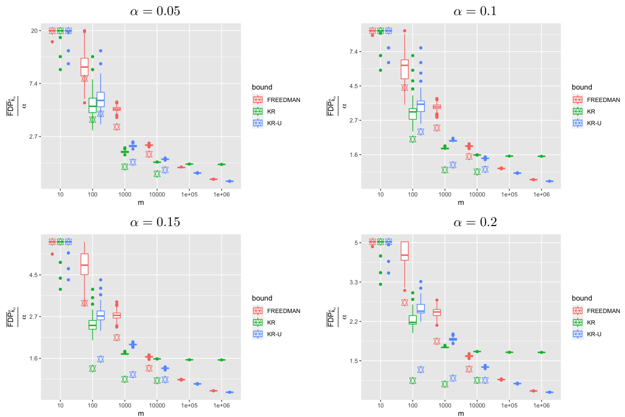
Figure B.6: Figure 3.6 where we have superposed in each case the (median of the) interpolated bounds (star symbols). Preordered sparse ( \beta = 0.25 ) LF setting with LF procedure ( s = 0.1\alpha , \lambda = 0.5 ).
