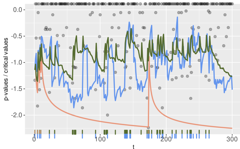
Figure 2.4: Sequences of critical values of LORD procedure with different rewards over time 1 \leq t \leq T = 300 (simulated data): base LORD critical values (B.13) (orange line), rewarded with the greedy approach (2.24) (blue line), and with the rectangular kernel SUR spending sequence (2.25) ( h = 10 , green line). The rug plots display the time of discoveries for each procedure with the corresponding color. The y -axis has been transformed by y \mapsto -\log(-\log(y)) . The grey dots denote the p -value sequence (those equal to 1 are displayed at the top of the picture). The spending sequence is \gamma_t \propto t^{-1.6} .
