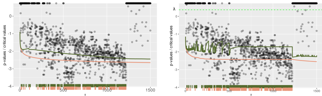
Figure 2.7: Applying online FWER controlling procedures to the male mice IMPC data set. Left panel: p -values and critical values for OB (orange curve) and \rho OB (green curve). Right panel: AOB (orange curve) and \rho AOB (green curve). Representation similar to Figure 2.3 ( Y -axis transformed by y \mapsto -\log(-\log(y)) ; p -values equal to 1 displayed at the top of the picture).
