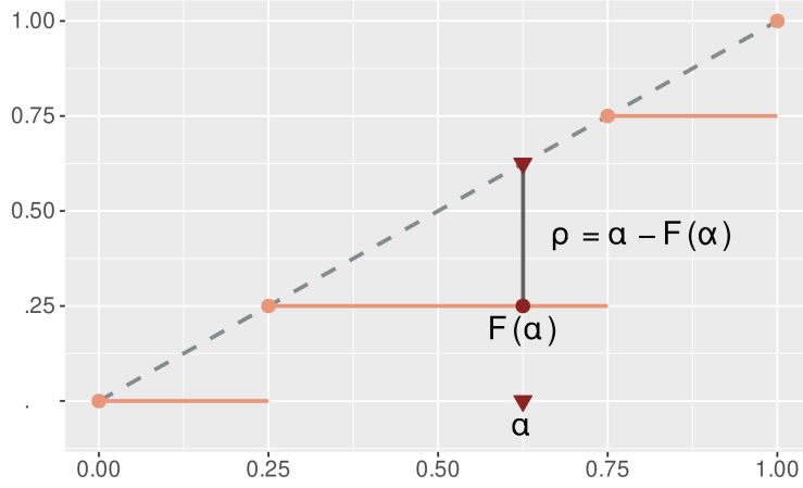
Figure 2.2: Super-uniformity reward \rho_t at time t (length of the vertical line) as defined by (2.8) for a given function F_t (orange step function) and a critical value \alpha_t (triangle). The dashed line is the identity function x \in [0, 1] \mapsto x .
