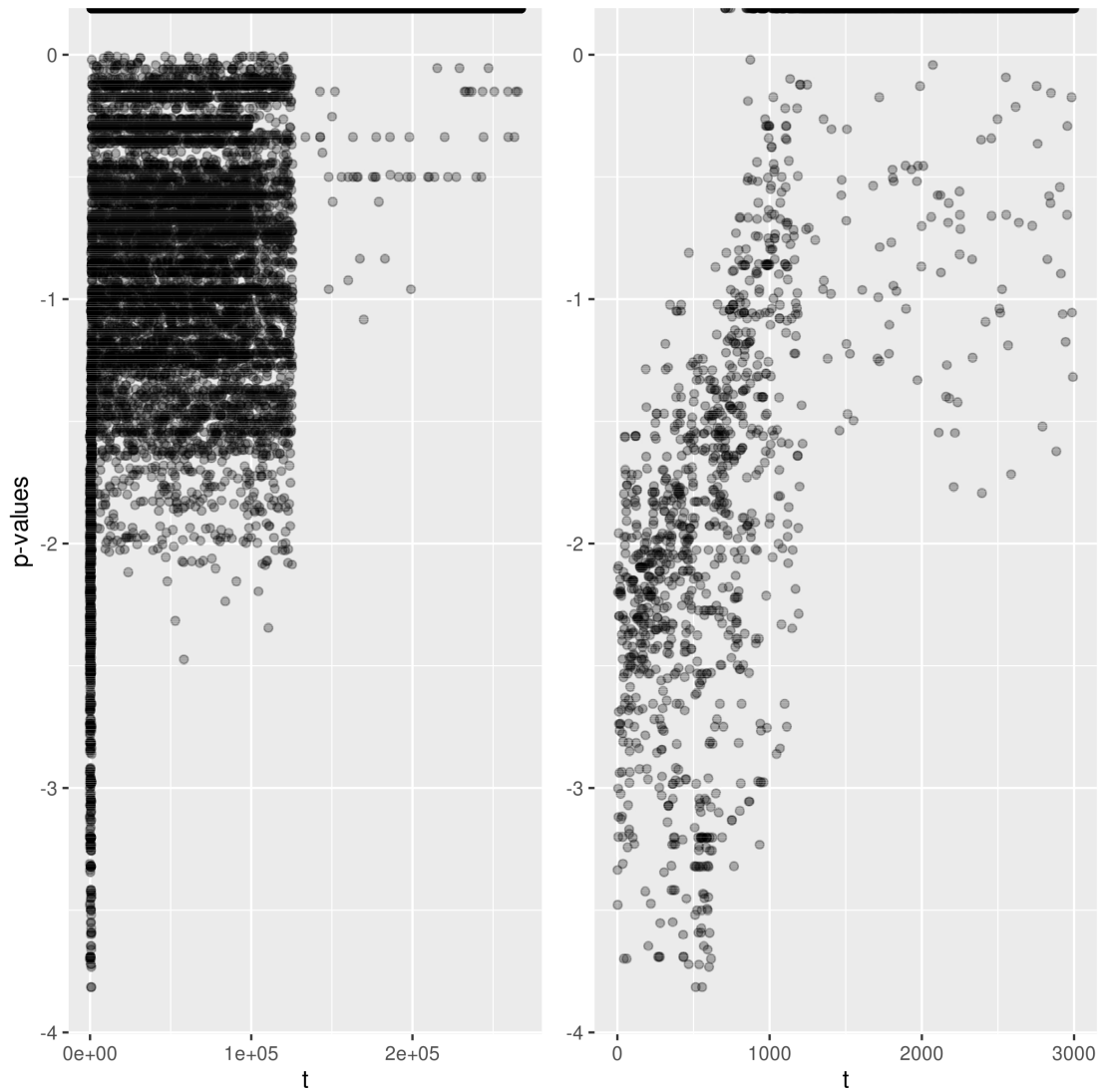
Figure A.10: p -values for female mice in the IMPC data of Section 2.5.3. The left panel presents all p -values, the right panel the first 3000 p -values. The p -values have been transformed as in Figure 2.3.
