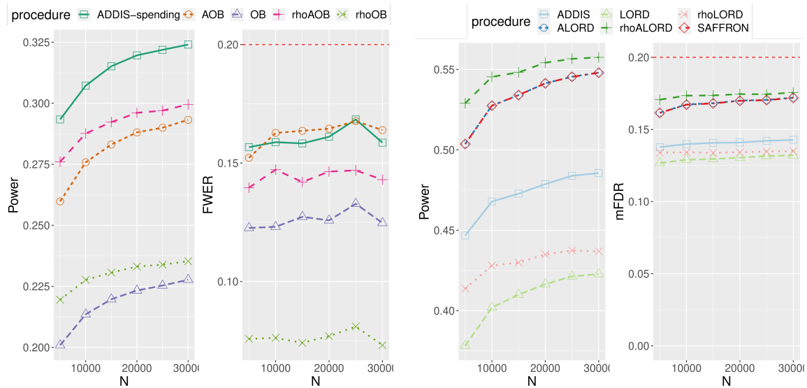
Figure A.6: Power and type I error rates of the considered procedures versus N \in \{5, 10, \dots, 30\} \times 1000 , with local alternatives.
