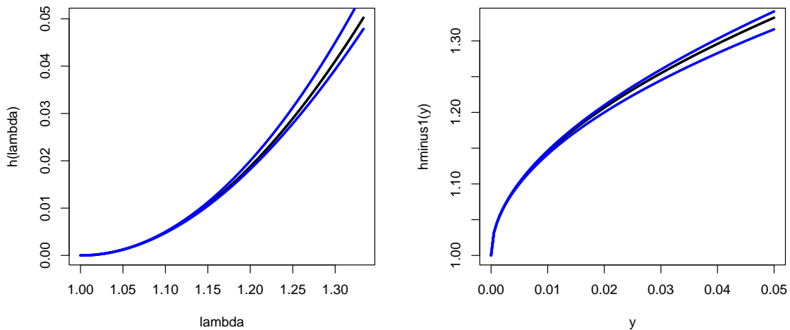
Figure B.1: Displaying h (left) and h^{-1} (right). Bounds of Lemma B.4.1 are displayed in blue.
