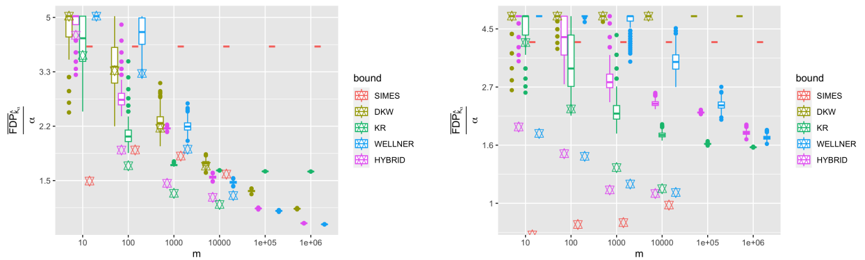
Figure B.3: Figure 3.2 where we have superposed in each case the (median of the) interpolated bounds (star symbols). Top- k sparse case \pi_0 = 1 - 0.5m^{-0.25}, \mu = \sqrt{2 \log m} (left) \pi_0 = 1 - 0.5m^{-0.55}, \mu = 10 (right), \alpha = 0.2 .
