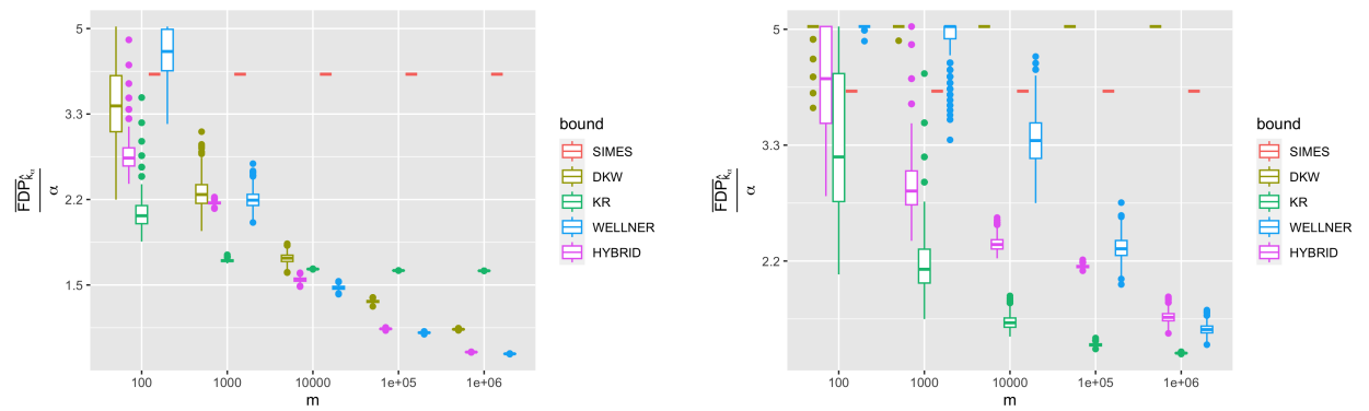
Figure 3.2: Top- k sparse case \pi_0 = 1 - 0.5m^{-0.25} , \mu = \sqrt{2 \log(m)} (left) \pi_0 = 1 - 0.5m^{-0.55} , \mu = 10 (right), \alpha = 0.2 .
