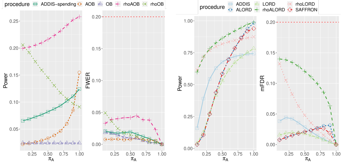
Figure 2.6: Power and type I error rates of the considered procedures for \pi_A \in \{0.1, 0.2, \dots, 0.9, 1\} .
