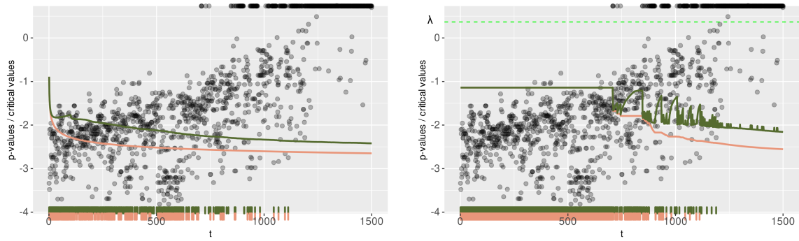
Figure A.11: Same as Figure 2.7 but for female mice of IMPC data (see Section 2.5.3).
