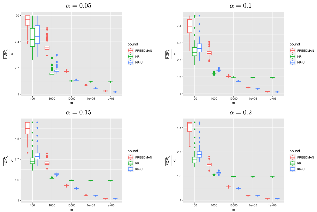
Figure 3.5: Preordered dense ( \beta = 0 ) LF setting with LF procedure ( s = 0.1\alpha , \lambda = 0.5 ).
