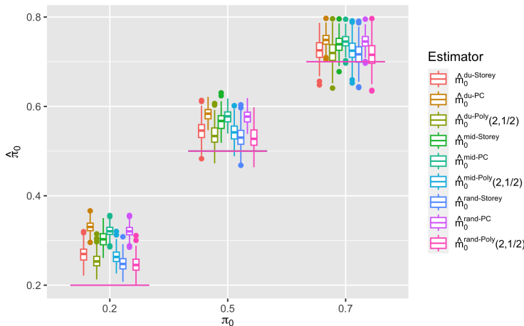
Figure 4.4: Comparison between discrete adjustments \hat{m}_0^{\text{du}} , \hat{m}_0^{\text{mid}} and \hat{m}_0^{\text{rand}} on simulated data.
