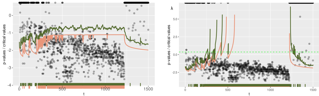
Figure 2.8: Applying online mFDR controlling procedures to the male mice IMPC data set. Left panel: p -values and critical values for LORD (orange curve) and \rho LORD (green curve). Right panel: ALORD (orange curve) and \rho ALORD (green curve). Representation similar to Figure 2.4 ( Y -axis transformed by y \mapsto -\log(-\log(y)) ; p -values equal to 1 are displayed at the top of the picture).
