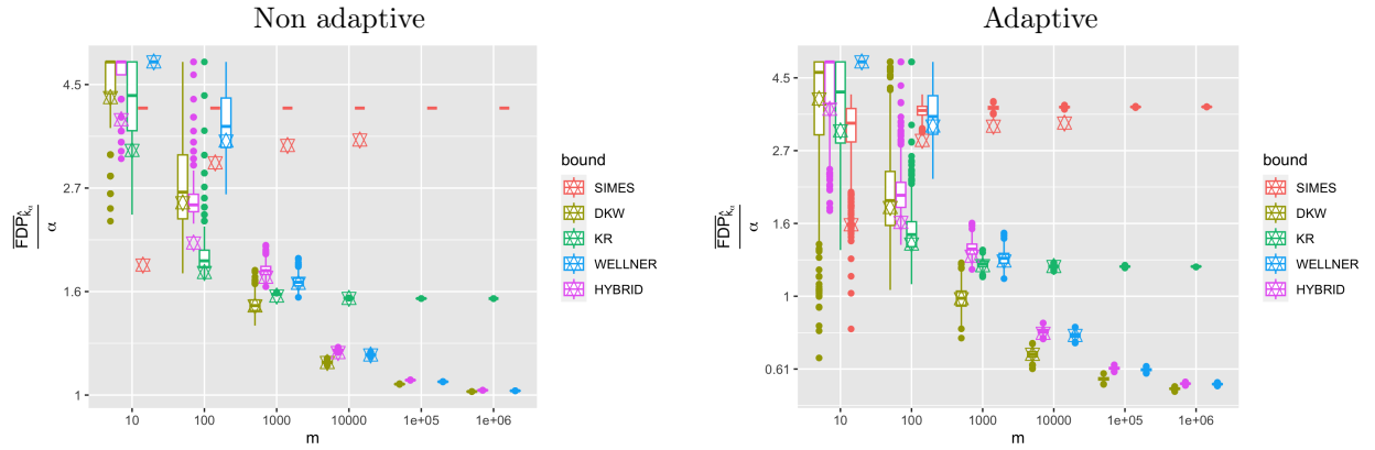
Figure B.4: Figure 3.3 where we have superposed in each case the (median of the) interpolated bounds (star symbols). Top- k dense case with nonadaptive bounds (left) and adaptive bounds (right) ( \pi_0 = 0.5 , \alpha = 0.2 ).
