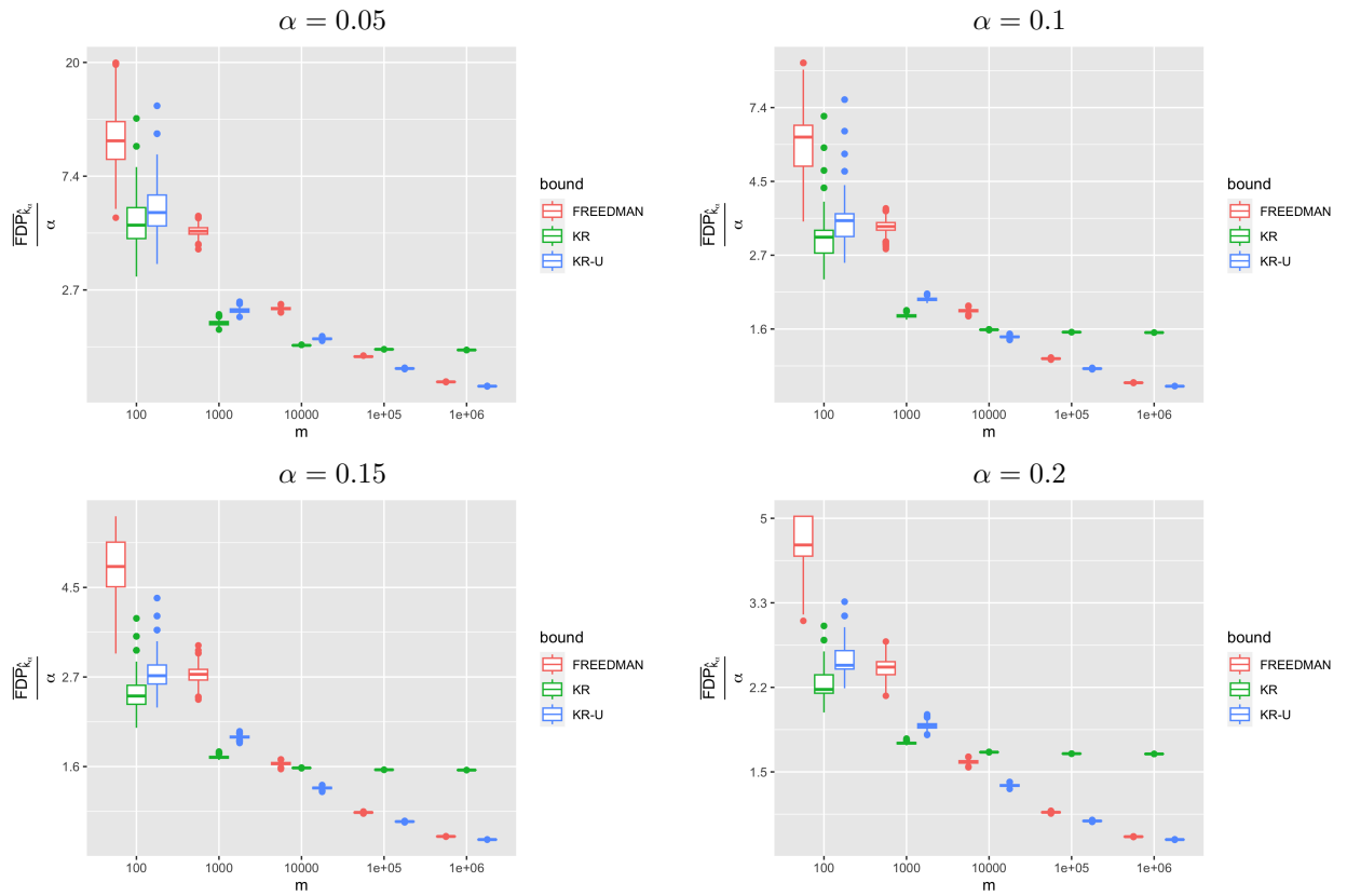
Figure 3.6: Preordered sparse ( \beta = 0.25 ) LF setting with LF procedure ( s = 0.1\alpha , \lambda = 0.5 ).
