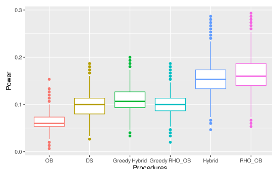
Figure A.3: Power of several online FWER controlling approaches for simulated data (see text): online Bonferroni (OB), Delayed spending (DS), greedy hybrid, greedy \rho OB, hybrid, \rho OB.
