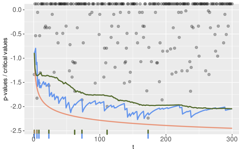
Figure 2.3: Sequences of critical values for Bonferroni procedures with different rewards over time 1 \leq t \leq T = 300 (simulated data): base Bonferroni critical values (2.10) (orange line), rewarded with the greedy approach (2.14) (blue line), and with the rectangular kernel SUR spending sequence (2.15) ( h = 100 , green line). The rug plots display the time of discoveries for each procedure with the corresponding color. The Y-axis has been transformed by y \mapsto -\log(-\log(y)) . The grey dots denote the p -value sequence (those equal to 1 are displayed at the top of the picture). The spending sequence is \gamma_t \propto t^{-1.6} .
