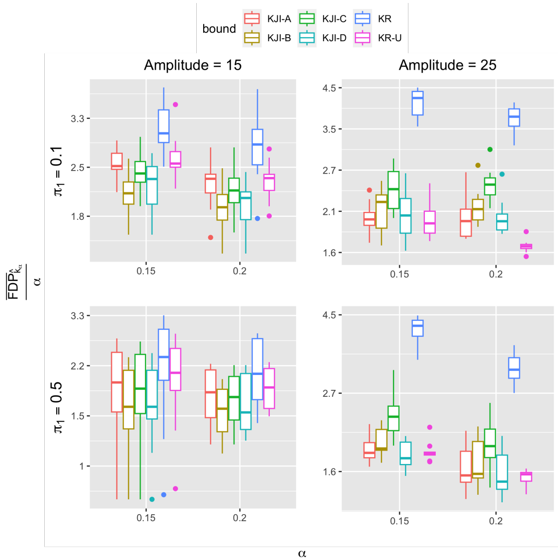
Figure 3.11: Comparing the FDP bound \widehat{\text{FDP}}_{\hat{k}_\alpha}^{\text{KR-U}} for \hat{k}_\alpha the BC procedure (3.32) ( s = \lambda = 0.5 ) to those of Li et al. (2022) with respect to \alpha \in \{0.15, 0.2\} in the Gaussian linear regression setting of Section 3.5.4 for m = 1000 (see text for more details).
