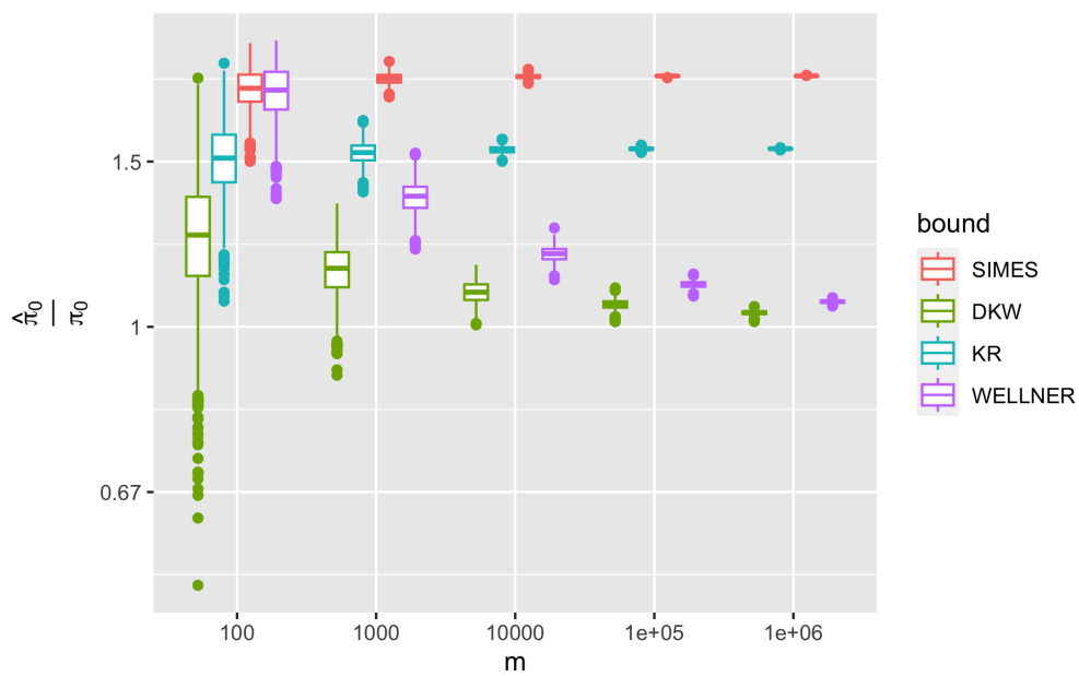
Figure 3.4: Boxplots of the estimators \hat{\pi}_0 in the top- k dense case ( \pi_0 = 0.5 , \alpha = 0.2 ).
