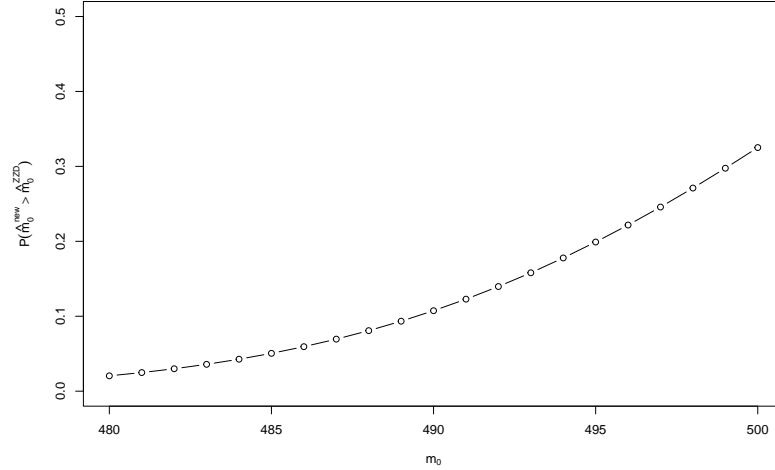
Figure C.2: Approximate probabilities \mathbf{P}(\hat{m}_0^{\text{PC,new}} > \hat{m}_0^{\text{PC,ZZD}}) for various values of true m_0 , with fixed m = 500 .
