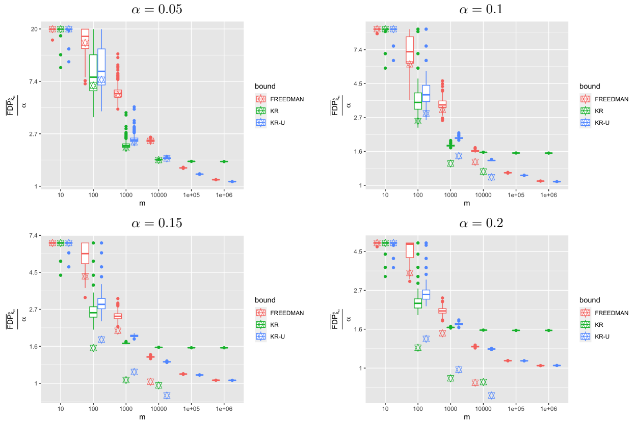
Figure B.5: Figure 3.5 where we have superposed in each case the (median of the) interpolated bounds (star symbols). Preordered dense ( \beta = 0 ) LF setting with LF procedure ( s = 0.1\alpha , \lambda = 0.5 ).
