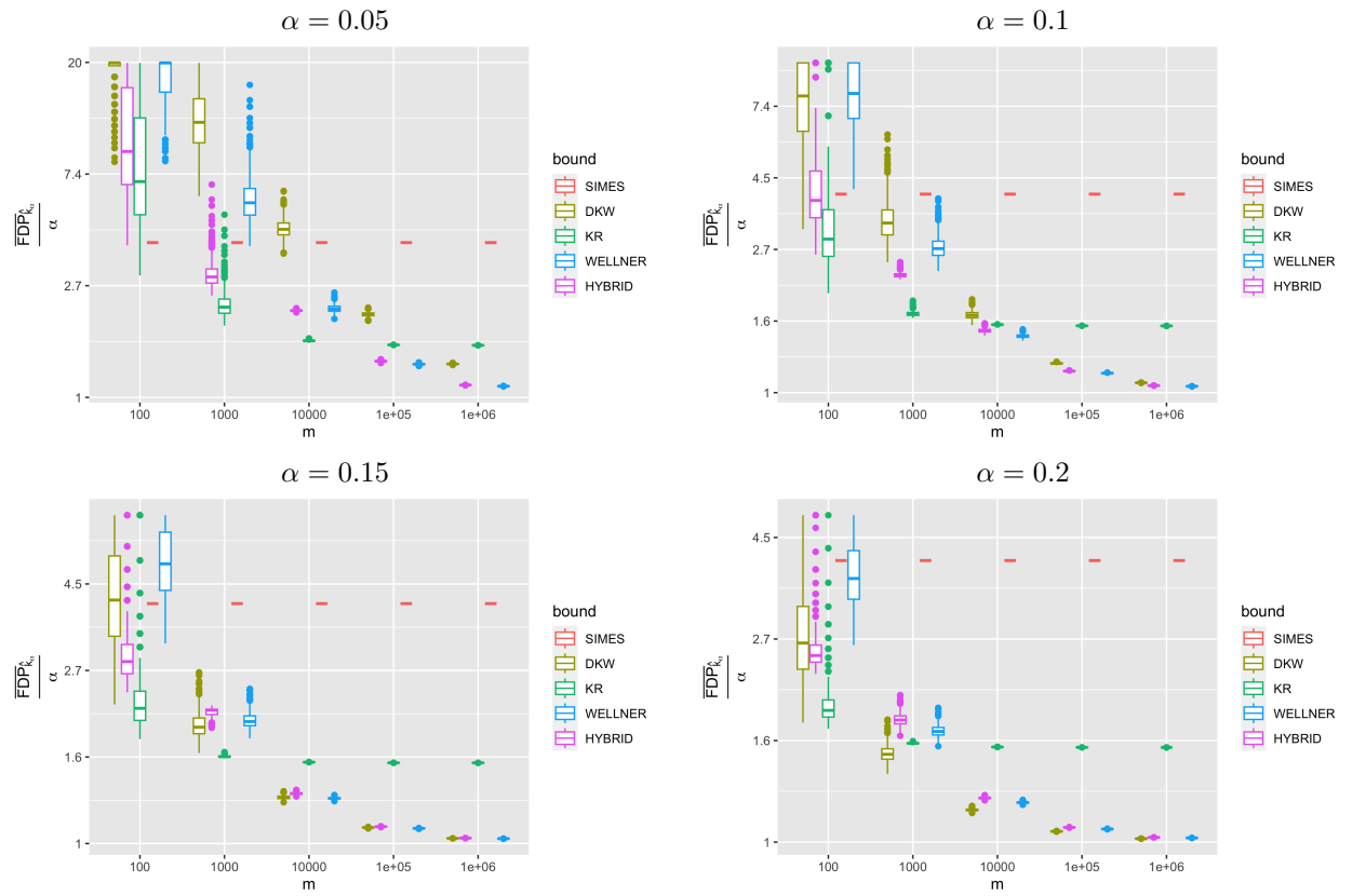
Figure 3.1: Top- k dense case ( \pi_0 = 0.5 , \mu = 1.5 ).
