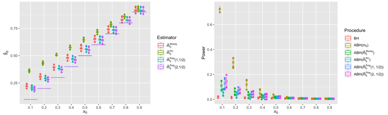
Figure C.3: Estimation results (left panel) for \hat{m}_0^{\text{Storey}} , \hat{m}_0^{\text{PC,new}} , \hat{m}_0^{\text{Poly}}(1, 1/2) , and \hat{m}_0^{\text{Poly}}(2, 1/2) , and power results (right panel) for the associated plug-in BH procedures on simulated data.
