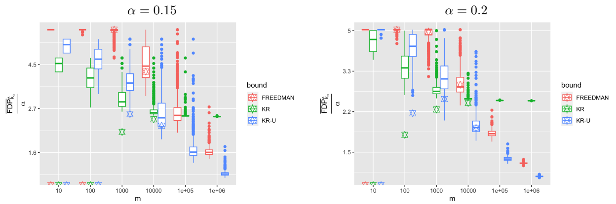
Figure B.8: Figure 3.8 where we have superposed in each case the (median of the) interpolated bounds (star symbols). Pre-ordered sparse ( \beta = 0.25 ) knockoff setting with BC procedure (i.e., LF procedure with s = \lambda = 0.5 ).
