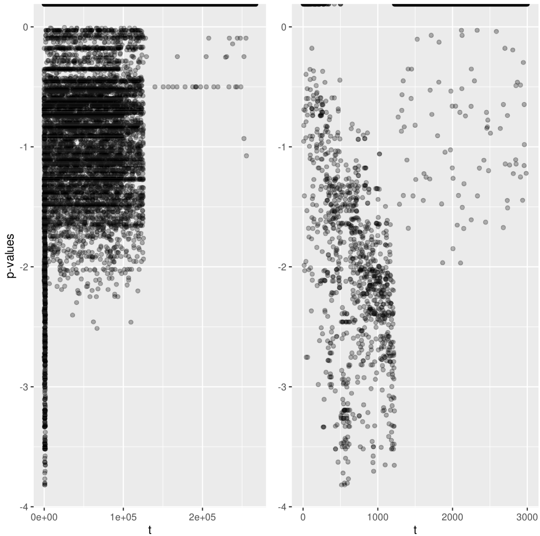
Figure A.9: p -values for male mice in the IMPC data of Section 2.5.3. The left panel presents all p -values, the right panel the first 3000 p -values. The p -values have been transformed as in Figure 2.3.
