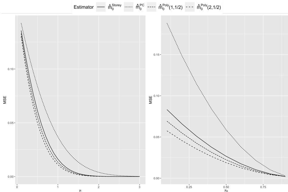
Figure 4.1: MSE against signal strength \mu \in [0, 3] with \pi_0 = 0.6 (left) and MSE against \pi_0 \in [0.1, 0.9] with \mu = 1.5 (right)
