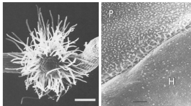
Figure 1.2. 48H-old haustorium (x150, bar represents 100 µm) and interface between haustorial hair (P) and host root surface (H) where secreted compounds (likely exopolysaccharides) have coalesced at the contact region (x10,000). Adapted from Baird and Riopel (1983).
