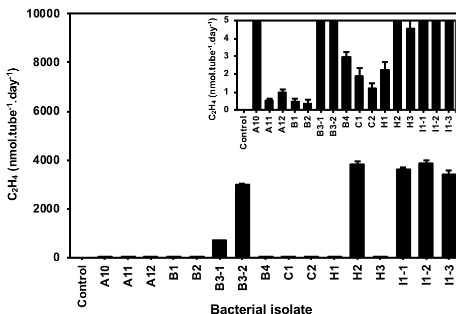
Figure 3.3. Nitrogenase activity of the 16 bacterial strains at the end of the 6 th purification round. Insert: scale enlargement. Nitrogenase activity was assessed by the acetylene reduction assay (ARA). Acetylene (10%) was provided to the bacteria after 3 days of growth at the sub-surface of N free semi-solid NFb medium, and ARA was measured 24h later. Means \pm SE, n = 3. Purification rounds and protocol: see Chapter 2, Figure 2.7.
