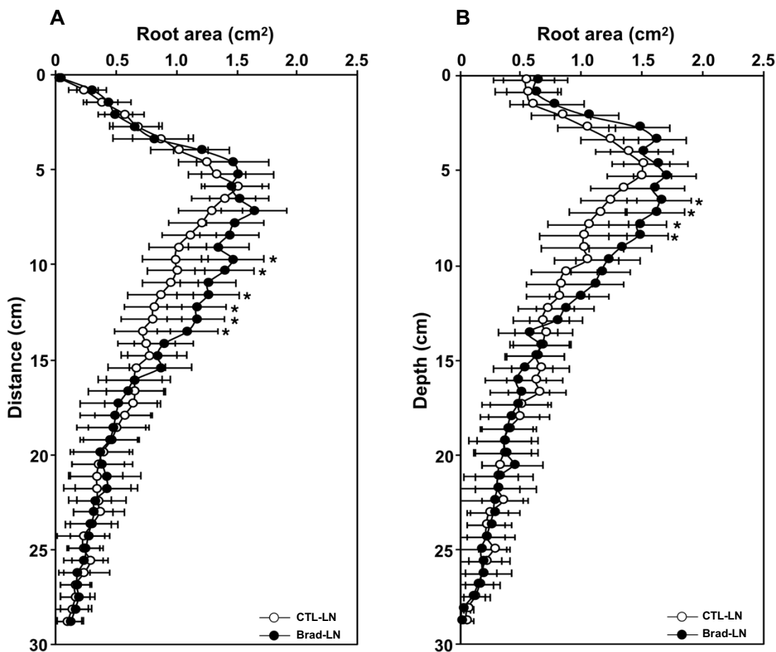
Figure 5.10. Effect of B. japonicum strain ORS285 on root system development. Plants were either inoculated with B. japonicum strain ORS285 (black symbols) or non-inoculated (open symbols) and grown in rhizobox devices for 12 days in LN solution. Images (scans) of 10 root systems at the end of the 12-d growth period are provided by Figure 5.7 for non-inoculated plants and 5.8 for inoculated plants. Root development was analyzed using the ACRT program, allowing to plot root surface area (derived from the number of root pixels on the 2-D image) as a function of either the distance to the seed (panel A) or the depth "in the soil" (panel B), i.e. , the distance to the horizontal line at the top of the rhizobox that would correspond to the "soil surface where germination would have occurred". ACRT program: see Chapter 4, Figure 4.17 and 4.18, and § 4.3.2.
