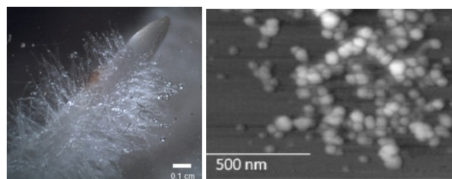
Figure 1.2. 48H-old haustorium (x150, bar represents 100 µm) and interface between haustorial hair (P) and host root surface (H) where secreted compounds (likely exopolysaccharides) have coalesced at the contact region (x10,000). Adapted from Baird and Riopel (1983).
