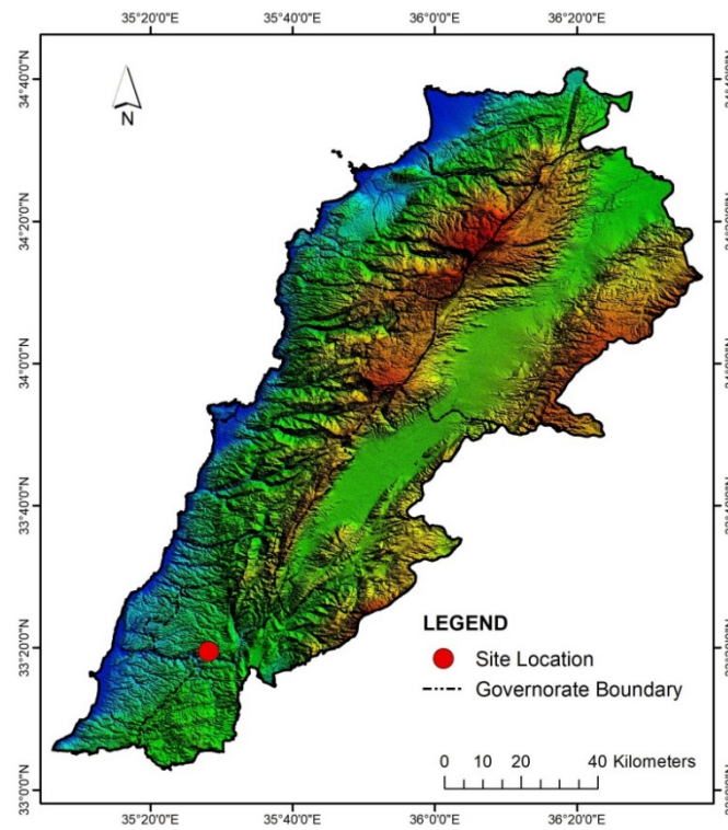
Figure 2.6. Bacterial strain collection site in Zawtar Al-sharkiya village, Nabatiyeh city, Labanon. Soil samples prepared from wheat root rhizosphere were collected by Houssein Zhour, PhD student in our group.
