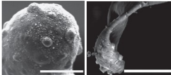
Figure 1.4. Developmental stages of ivy root hairs. Protuberances are present at the tip of root hairs and may represent the location of adhesive excretion. Later, root hairs dessicate, squeeze and lignify looking as curled ribbon (left panel scale bar, 5 mm, right panel scale bar, 10 mm). (Adapted from Melzer et al. , 2010).
