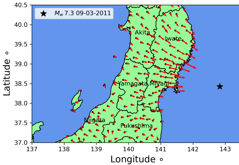
Figure 3.1: Ground deformation (red arrows) due to the magnitude 7.3 earthquake occurred in offshore Japan (black star) the 9th March 2011. It is evident how the deformation direction and magnitude is strongly correlated with the location of the earthquake. GPS data extracted from the Nevada Geodetic Laboratory repository.
