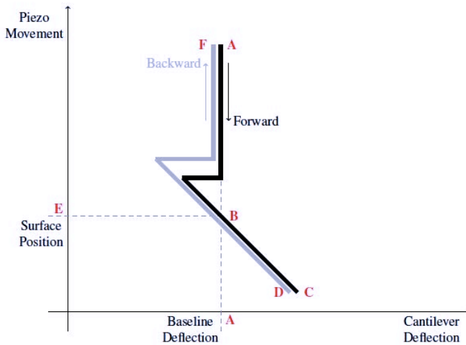
Fig. 2.9 The force-plot of an AFM. Source: AD
