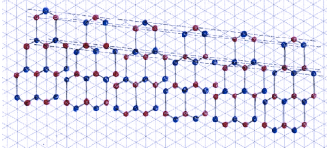
Fig 4.29 A schematic representation of hexagonal boron nitride structure, with the alternate layers of the two elements. Source: AD
