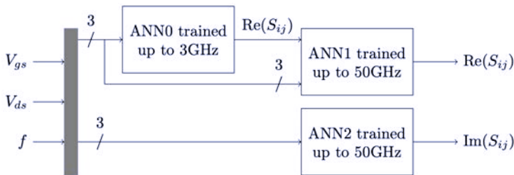
Fig 5.71 The small-signal bias-dependent hierarchical Prior Knowledge Input neural model. Source: adapted from Marinković et al. (2011)
