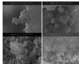
Figure 4: Top left: \alpha -Fe 2 O 3 spherulic structure. Top right: NiO cubic geometry, according to fcc crystallographic unit cell. Bottom pictures: SEM details of the reacted samples where the collars are visible and nanodimensioned. Source: AD (2002) Magnetic and Structural Properties of NiFe 2 O 4 Nanoferrites. Unpublished Master's Thesis, University of Ferrara, Italy.
