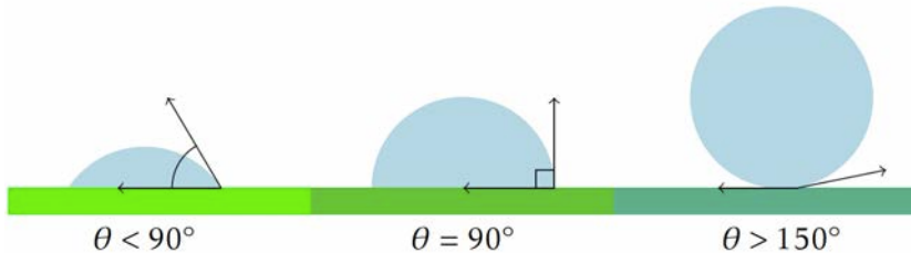
Fig. I.5 On the left, a non-hydrophobic situation, with a contact angle lesser than 90^\circ ; in the centre the limit situation, above which we speak of a water-repellent (hydrophobic) surface; on the right, the super-hydrophobic surface situation. In the latter case, the drop of water is practically supported, almost entirely, by the surface. Source: AD
