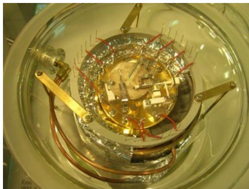
Fig. I.23 The first Scanning Tunneling Microscope, Bonn, Deutsches Museum. Source: J. Brew. https://www.flickr.com/photos/brewbooks/176058521/in/photostream/ CC BY-SA 2.0
