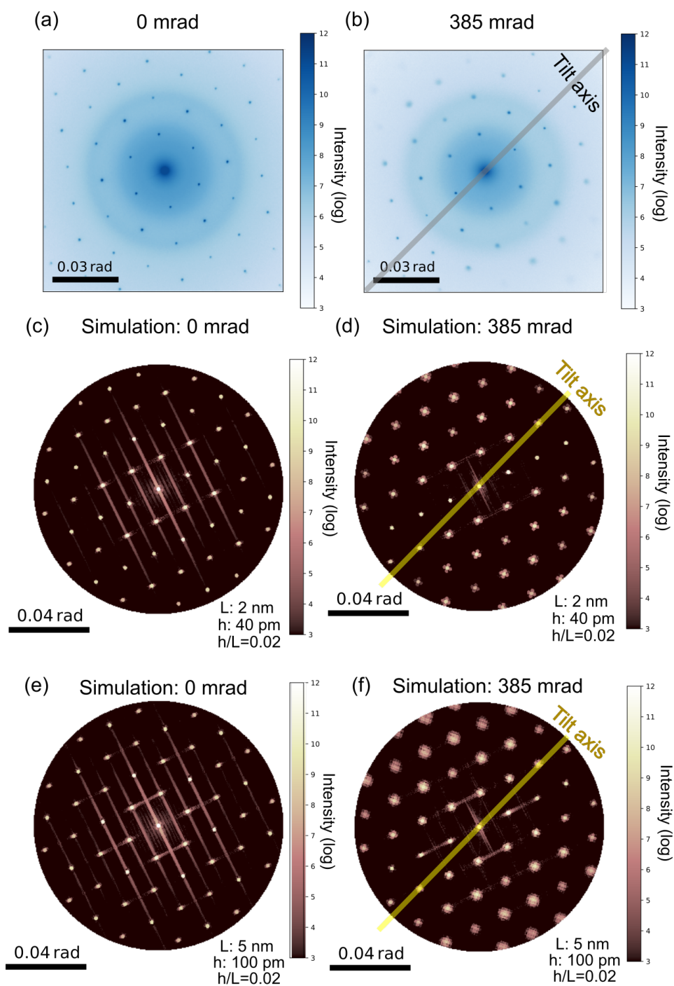
Figure A.4: Roughness of \text{Si}_3\text{N}_4 supported \text{WS}_2 monolayer: (a) and (b) are experimental results of diffraction patterns at 0 and 385 mrad tilt angles; (c) and (d) are the simulation results of h/L = 0.02 with period of L = 2 nm; (e) and (f) are the simulation results of h/L = 0.02 with period of L = 5 nm.
