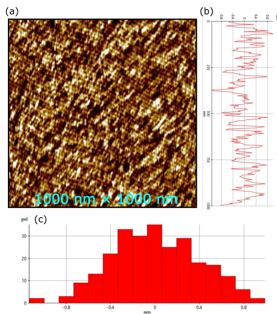
Figure A.5: AFM measurement the roughness of S_3N_4 membrane: (a) AFM mapping of 1000 nm \times 1000 nm area of 15 nm- S_3N_4 TEM support windows; (b) the height of 1000 nm line profile; (c) histogram of (a), the amplitude is in the range of -0.8 nm to 0.8 nm
