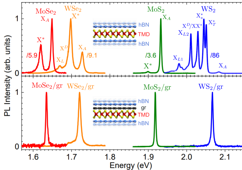
Figure 8.11: PL spectra of hBN/TMDs/hBN and hBN/graphene/TMDs at around 20 K. The scaling factors indicate a direct PL intensity comparison between TMD and TMD/graphene encapsulated between hBN flakes. Normalizing all spectra to unity is done by taking the most intense feature as the reference. Reproduced from ref. [18].
