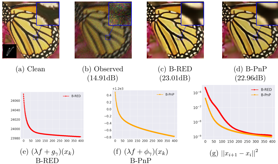
Figure 6.3: Deblurring from the indicated motion kernel and Poisson noise with \alpha = 40 .
