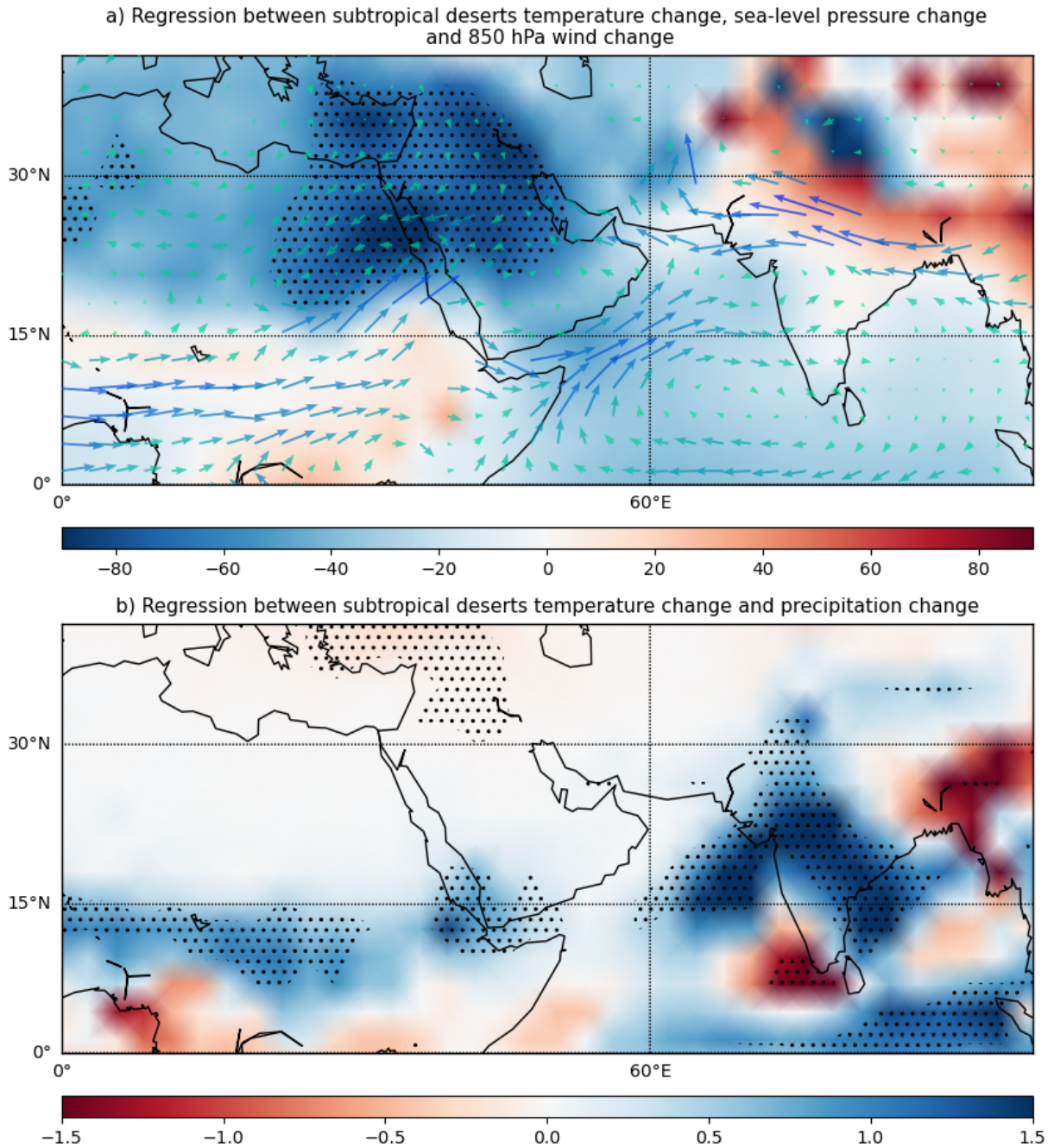
Figure 4.4: Inter-model regressions against the subtropical deserts temperature change of (a): changes in SLP (color shaded, \text{Pa.K}^{-2} ) and wind at 850 hPa (vectors, \text{m.s}^{-1}.\text{K}^{-2} ); (b) precipitation change (color shaded : 0.1 \text{ mm.d}^{-1}.\text{K}^{-2} ). The colors of the arrows vary from blue to green according to the intensity of the wind speed for readability. On panel (a) dotted points indicate grid-points where the regression with SLP change is significant at the 95% confidence level. On panel (b), dotted points indicate grid-points where the regression with precipitation change is significant at the 95% confidence level.
