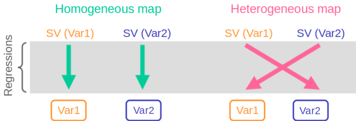
Figure 2.1: Homogeneous and heterogeneous maps from MCA.
