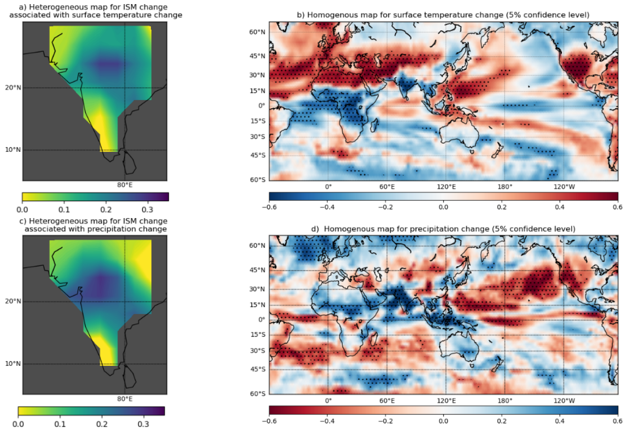
Figure 4.1: Heterogeneous (a) and homogeneous (b) maps obtained from the MCA analysis performed between the scaled surface temperature change ( K.K^{-1} ) of the 32 climate models and the scaled ISM precipitation changes ( mm.d^{-1}.K^{-1} ) in the same 32 models. (c) and (d): same as (a) and (b) for the MCA between the precipitation change ( mm.d^{-1}.K^{-1} ) and the ISM precipitation change ( mm.d^{-1}.K^{-1} ). Dotted points indicate pointwise correlations significant at the 95% confidence level between the respective Singular Variable (SV) and grid-point model series using a Student test with 31 degrees of freedom.
