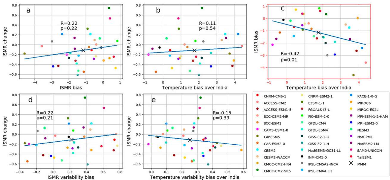
FIG. 3. Scatterplots of ISMR change ( \text{mm day}^{-1} ), respectively, with (a) mean ISMR bias ( \text{mm day}^{-1} ), (b) mean temperature bias over India ( \text{K} ), (d) ISMR standard deviation bias ( \text{mm day}^{-1} ), and (e) temperature standard deviation bias over India ( \text{K} ). Temperature biases are calculated over India, which corresponds to the same domain as the one used for ISMR. Temporal standard deviation in (d) and (e) is computed for each individual historical member and averaged for each model in case of several members. (c) Scatterplot of mean ISMR bias and mean surface temperature bias over India to illustrate local interaction between temperature and precipitation bias over India. The correlation and its associated p value for each pair of model series are indicated in each panel. The red outline means that the correlation is significant at the 95% confidence level ( p < 0.05 ). Crosses indicate the MMM position in each scatterplot.
