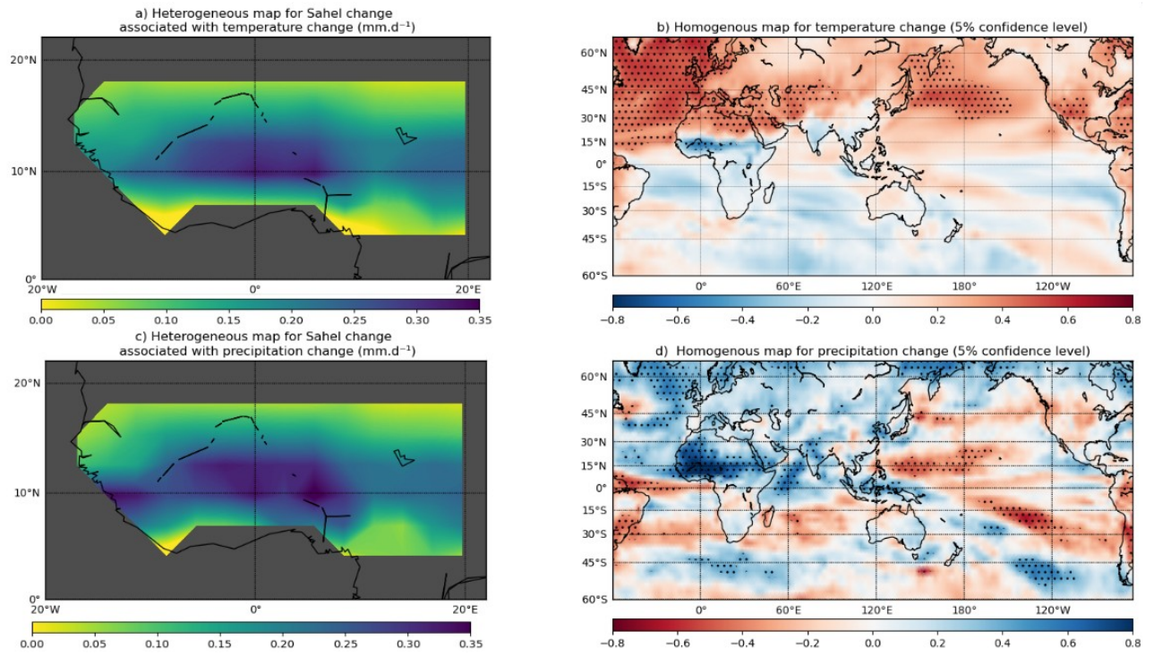
Fig.S4: same as Fig.3 but with unscaled temperature and precipitation fields.
