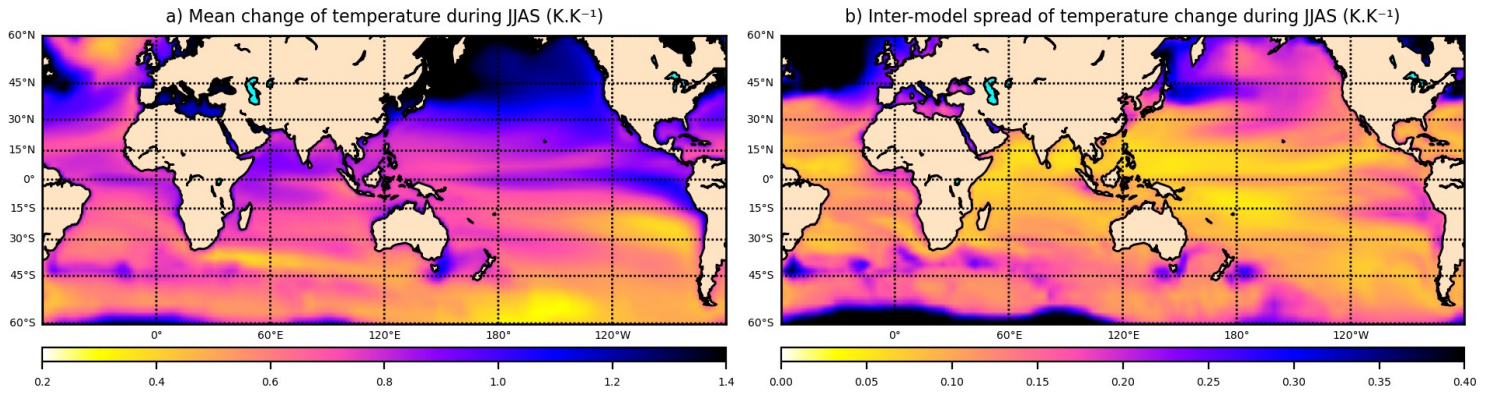
Fig. S1. (a) MMM temperature change ( \text{K.K}^{-1} ), (b) inter-model spread of temperature change ( \text{K.K}^{-1} ), during JJAS and ocean-only. Computed for the 32 CMIP6 models.
