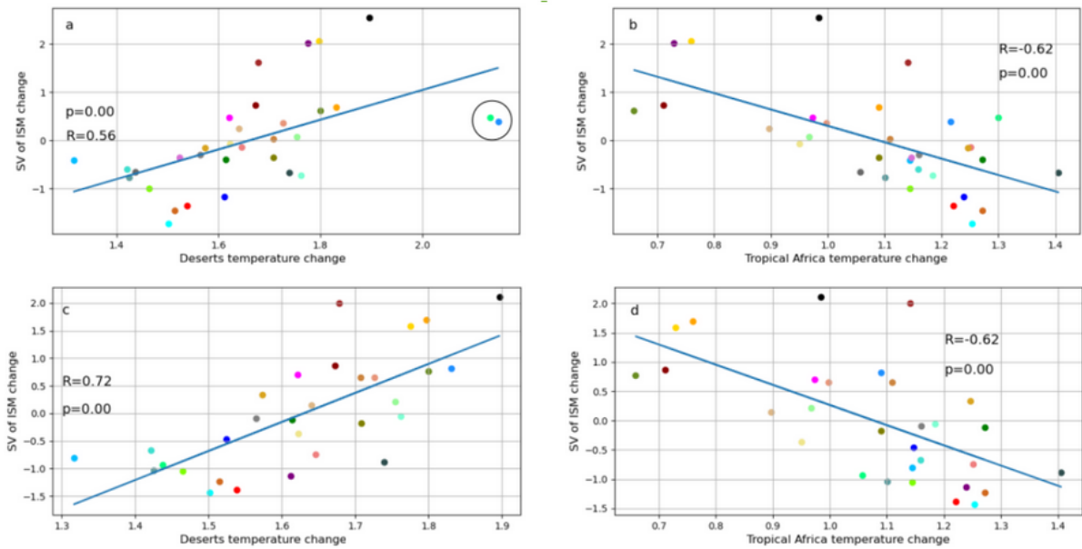
Figure 4.3: Scatterplots of SV of ISM change ( mm.d^{-1}.K^{-1} , from Figure.4.1a), respectively, with (a) deserts temperature change ( K.K^{-1} ), (b) tropical Africa temperature change ( K.K^{-1} ). (c) and (d), same as (a) and (b) but without the outliers. The definition of each index can be found in Table 2. All model series are scaled by the global temperature change in each model. The correlation and its associated P-value for each pair of model series are indicated in each panel.
