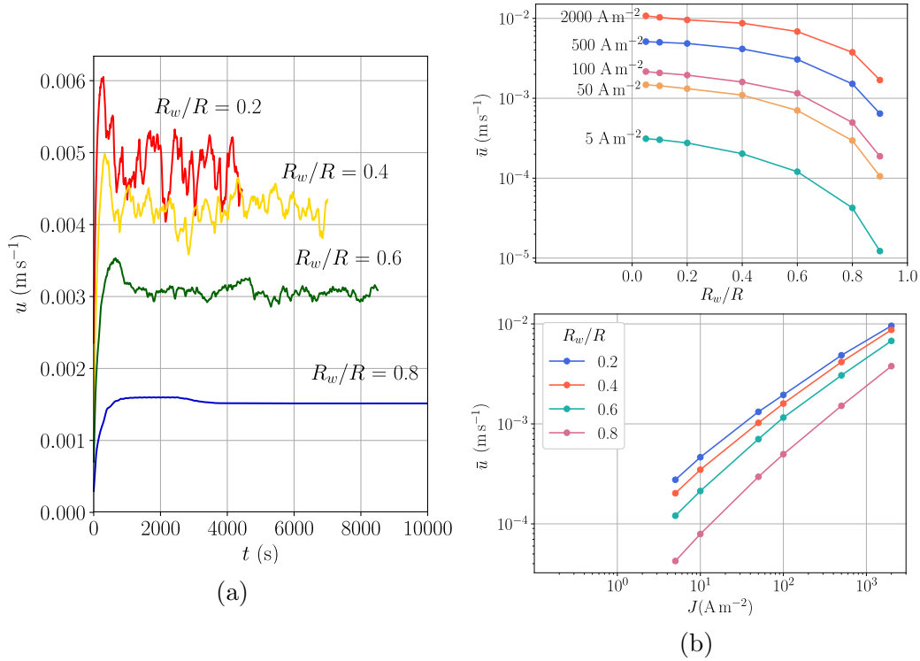
Figure 3.17 – (a) Evolution of the velocity \mathbf{u} with time for different R_w/R and J = 500 \text{ A m}^{-2} . (b) Time- and volume-averaged velocity \bar{\mathbf{u}} as a function of R_w/R for different J (top), as a function of J for different R_w/R (bottom).
