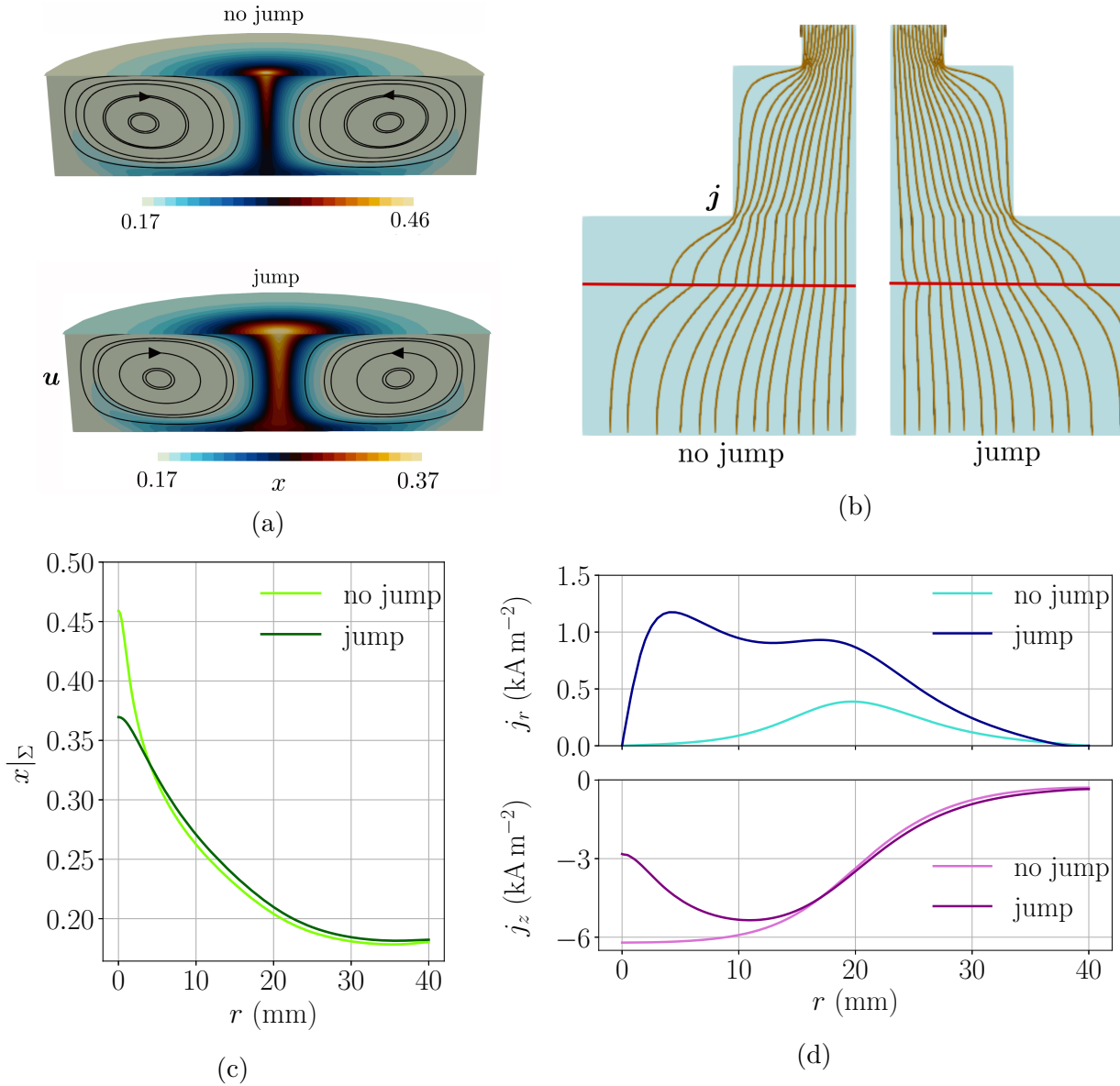
Figure 5.14 – I=10 A. Molar fraction in the alloy and current density in the case with EVF and no buoyancy, at t=500 s, with or without jump coupling. (a) Snapshots of the molar fraction of lithium in the alloy x . (b) Streamlines of the current density in the cell. (c) Molar fraction x|_{\Sigma} at the alloy-electrolyte interface as a function of radius r . (d) Current density j_r (top) and j_z (bottom) at the alloy-electrolyte interface as a function of radius r .
