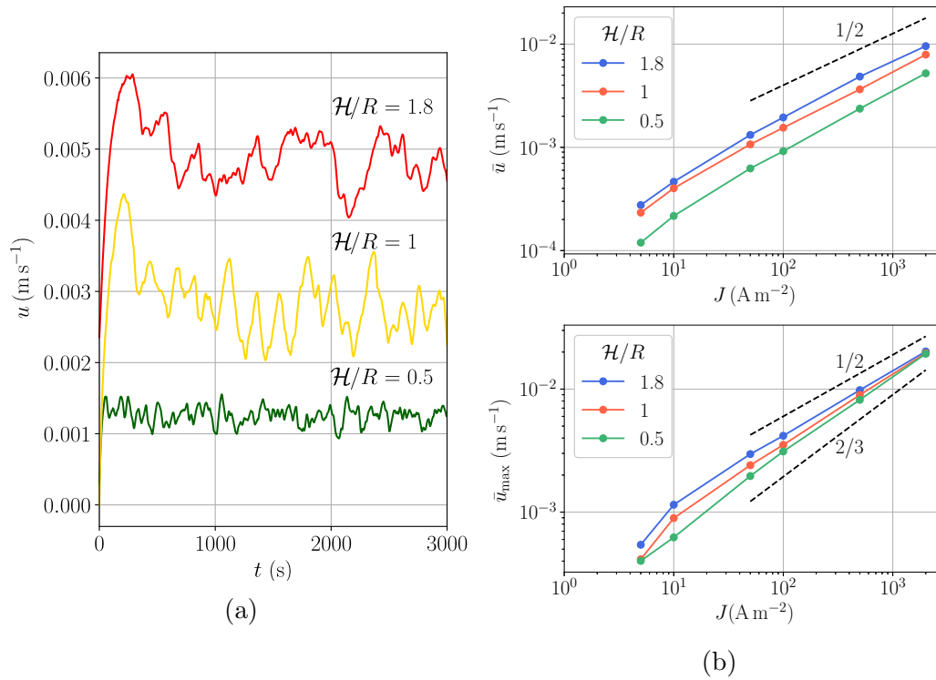
Figure 3.20 – (a) Volume-averaged velocity u for different aspect ratios and J = 500 \text{ A m}^{-2} . (b) \bar{u} (top) and \bar{u}_{\max} (bottom) as a function of J .
