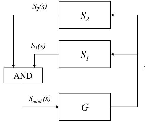
Figure 3.3 – Modular control architecture [Cas08]
