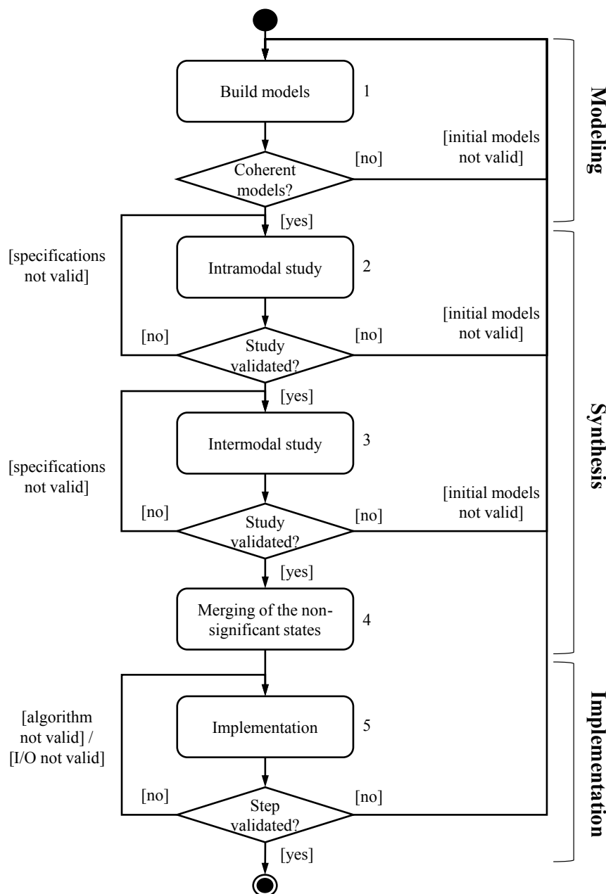
Figure 5.1 – Proposed approach for mode-switching control design
