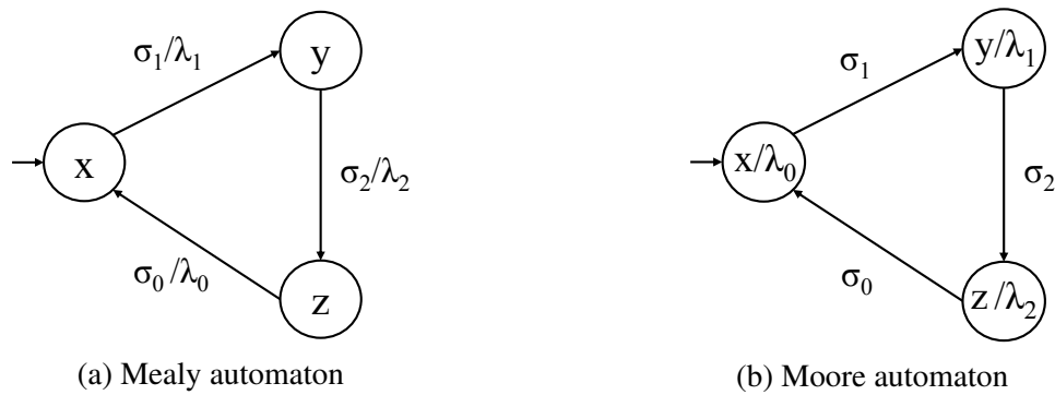
Figure 3.10 – State-transition diagrams of Mealy and Moore automata
