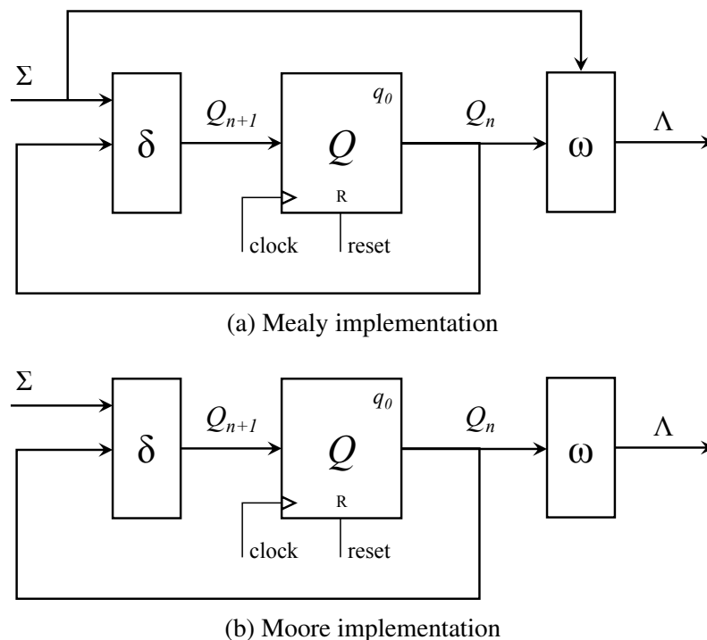
Figure 3.11 – Sequential logic circuits of Mealy and Moore automata
