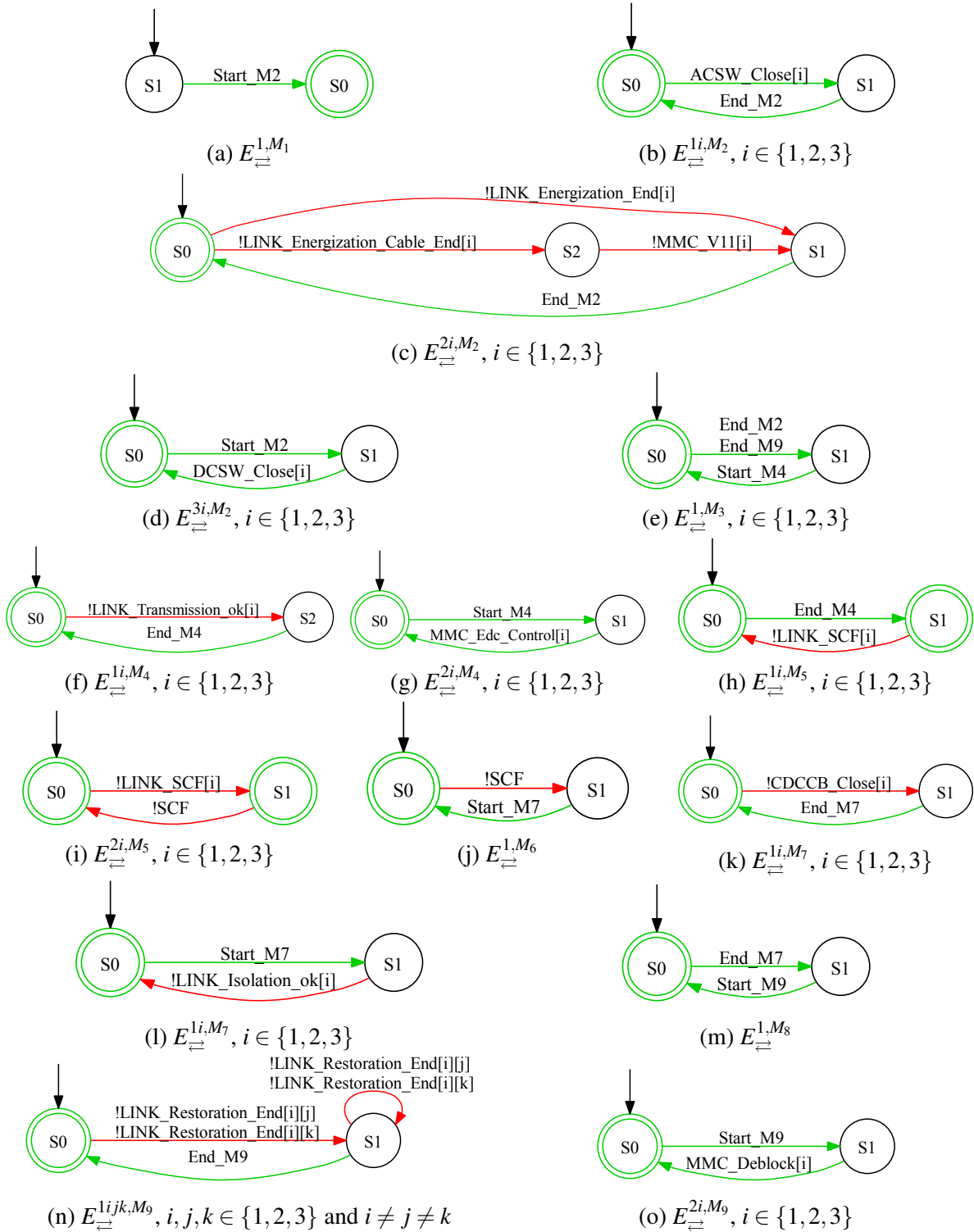
Figure 6.8 – Intermodal specification and plant models
