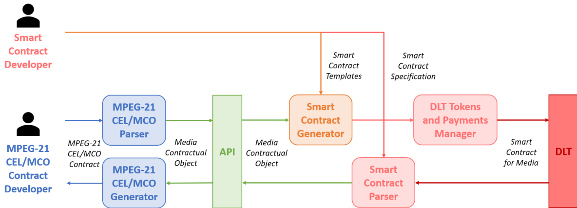
Figure 45: MPEG-21 Contract Expression Language (CEL)/Media Contractual Object (MCO) contracts to and from Smart Contracts conversion workflow.
