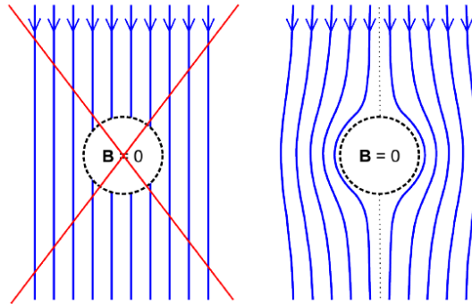
Figure 1.6: The configuration with field lines ending on the surface of the inclusion is excluded when \text{div } \mathbf{B} = 0 . Source: [31]
