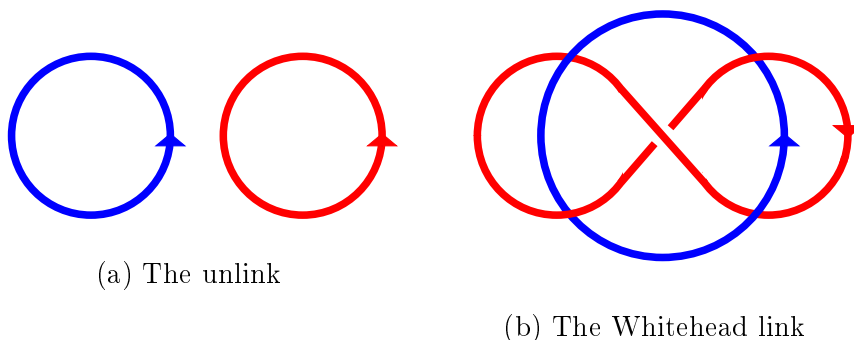
Figure 1.6 – The unlink and the Whitehead link are both of linking number 0 but the Whitehead link is topologically linked.
