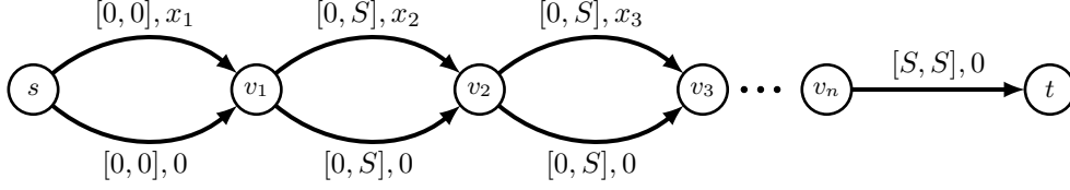
Figure 1.8: Representation of the reduction from the partition problem to the computation of earliest arrival time in piecewise constant temporal graphs with forbidden waiting.
