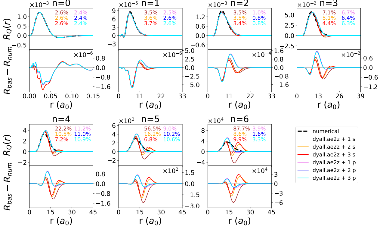
Figure D.3: Scheme I. Radial distributions of electric transition multipole moments in the generalized length representation for the 1s_{1/2} \rightarrow 7p_{1/2} transition. The basis sets for these calculations were generated by augmenting the dyall.ae2z basis set with diffuse functions in an even-tempered fashion. The percentages in the upper right corner of each box are the relative errors of the transition moments, i.e. \left| \frac{T_{bas} - T_{num}}{T_{num}} \right| \times 100\% .
