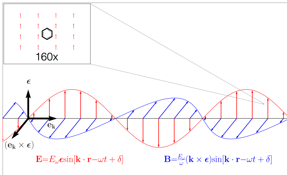
Figure 1.1: schematic representation of a benzene molecule interacting with linearly polarized red light ( \lambda = 700 nm) consisting of an electric (red) and magnetic (blue) component. To make the magnetic field amplitude visible in this picture, it is not depicted at its true relative scale with respect to the electric field. The benzene molecule is only visible after zooming into a small region of space and in this region, the molecule effectively experiences a uniform field, which is dominated by its electric component. The mathematical expressions describing the electromagnetic fields are given at the bottom of the box. The propagation- and polarization direction are described by the unit vectors \mathbf{e}_k and \boldsymbol{\epsilon} , respectively, with the latter being defined by the relation \mathbf{e}_k = \frac{c}{\omega} \mathbf{k} .
