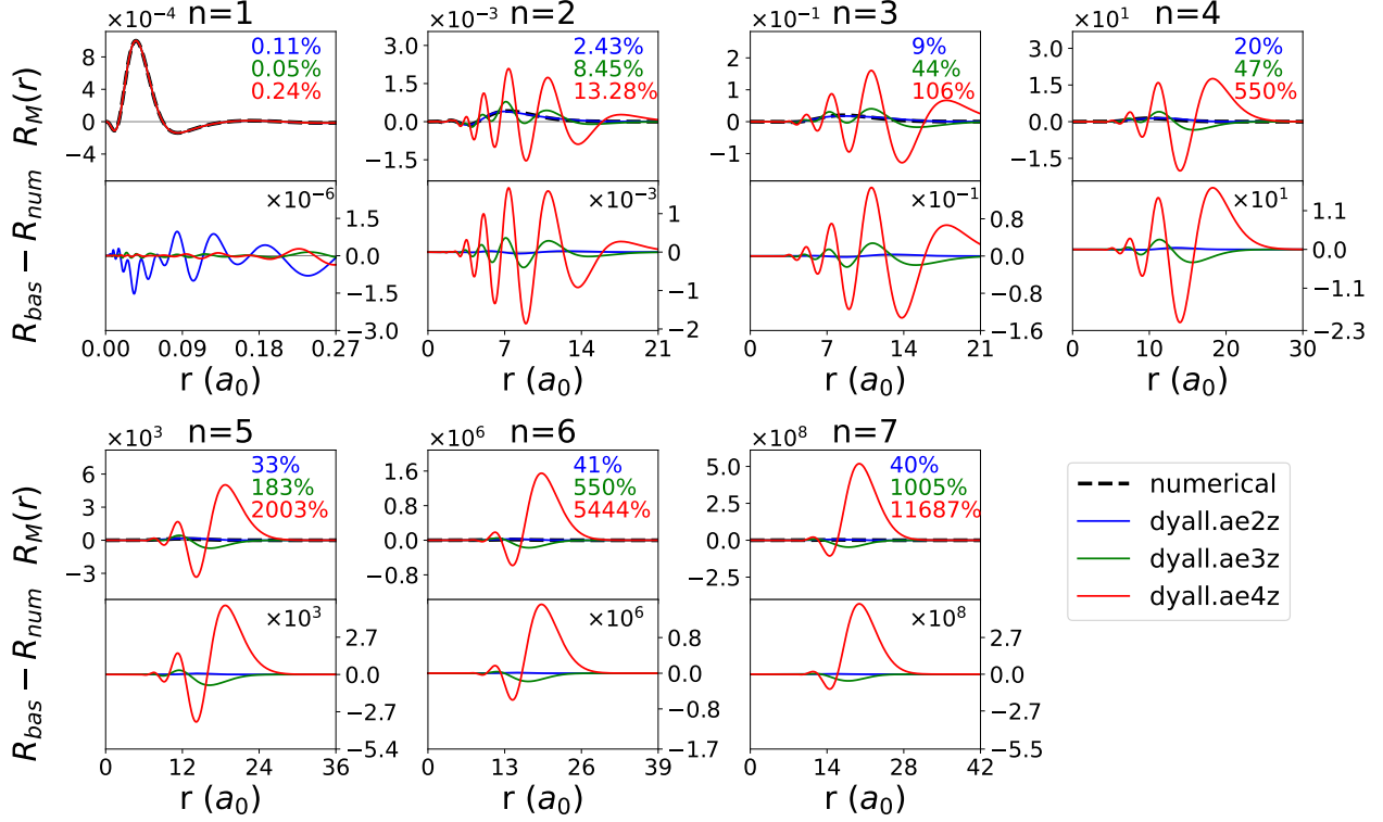
Figure D.1: Core transition ( 1s_{1/2} \rightarrow 7p_{1/2} ): radial distributions of magnetic multipole moments \hat{m}^{[2n]}, n \in [1, 7] . These distributions are calculated with the default linear dependence thresholds: 10^{-6} and 10^{-8} for the large and small component space. In each box, the upper panel contains the radial distribution, while the lower panel contains error relative to the numerical reference. Note that each box has different scales. The percentages in the upper right corner of each box are the relative errors of the transition moments, i.e. |\frac{T_{bas}-T_{num}}{T_{num}}| \times 100\% .
