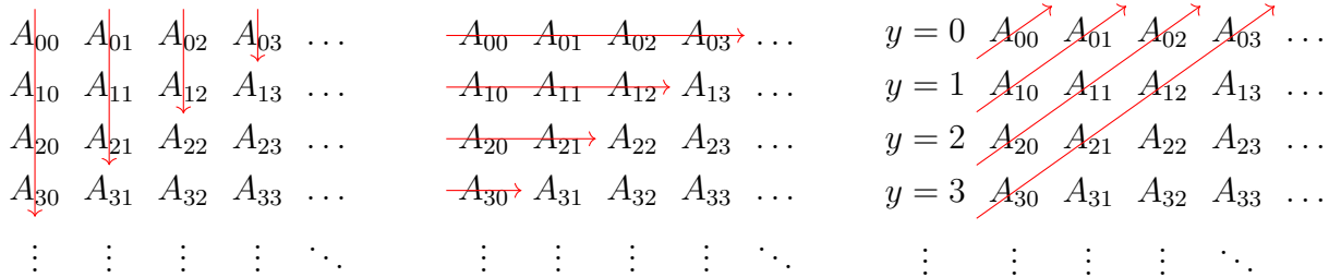
Figure C.4: diagrammatic representation of the column-wise (left), row-wise (middle) and diagonal (right) summation of the sub anti-diagonals and anti-diagonal of a matrix. For the summation on the right, the index y = n + m is given for each (sub) anti-diagonal.
