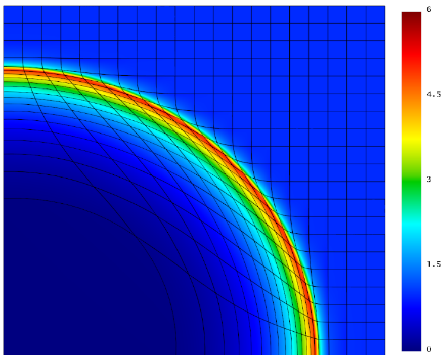
Figure 1.2: Simple Sedov Blast wave problem 2d modelization. LULESH represents this problem on a 3d cartesian mesh
