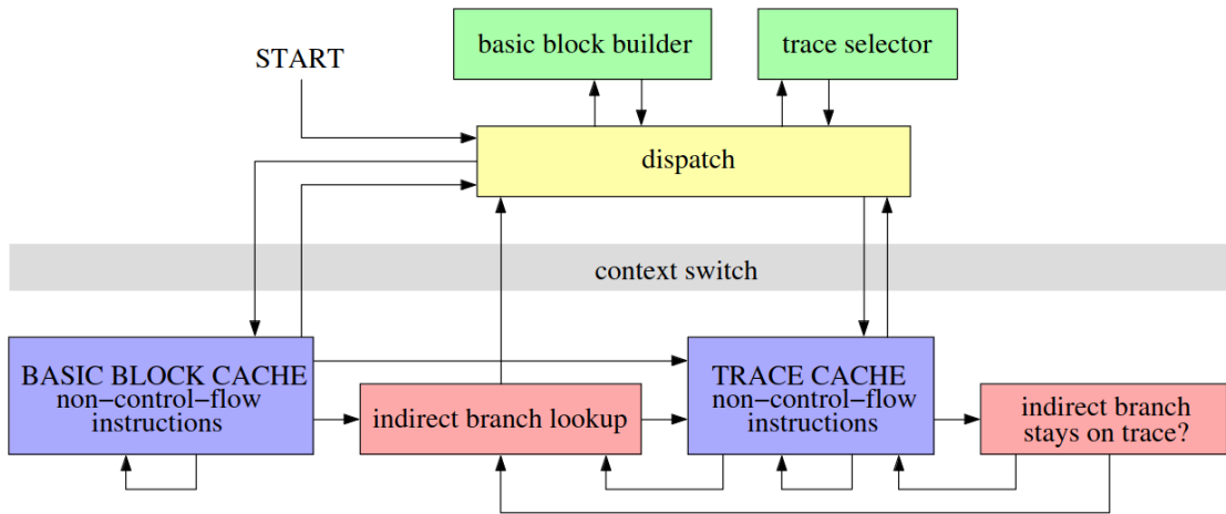
Figure 6.7: DynamoRIO flow chart. The application code is stored in the two caches separated from the DynamoRIO code by a context switch. Source: [33]
