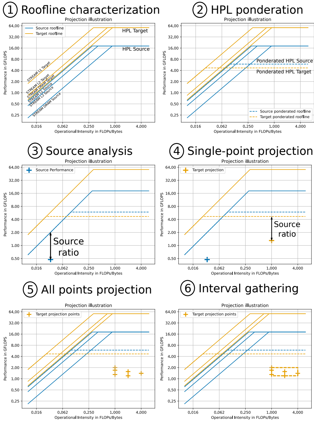
Figure 6.6: Illustration of the performance projection approach with the different steps of the projection. All the figures present the OI (FLOP/Bytes) on the x-axis and the Performance (GFLOPS) on the y-axis.
