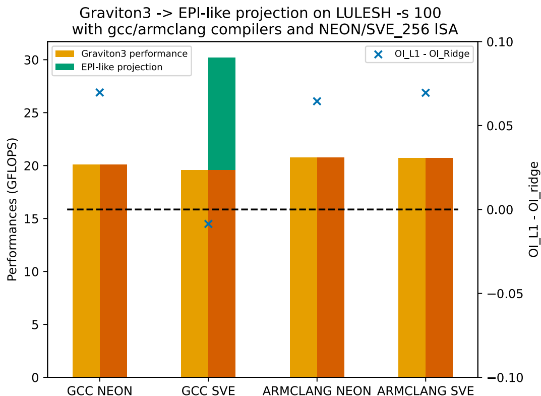
Figure 7.5: Observed performance, projections, and OIs of LULESH with different compilers and ISA on two node architectures: Graviton3 and EPI-like. The OI_{L1} - OI_{Ridge} value is represented with blue crosses.
