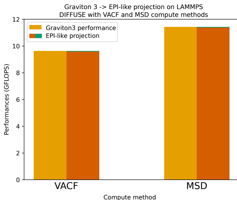
Figure 7.4: Projections of two compute methods of LAMMPS DIFFUSE small benchmark from Graviton 3 to our EPI-like machine
