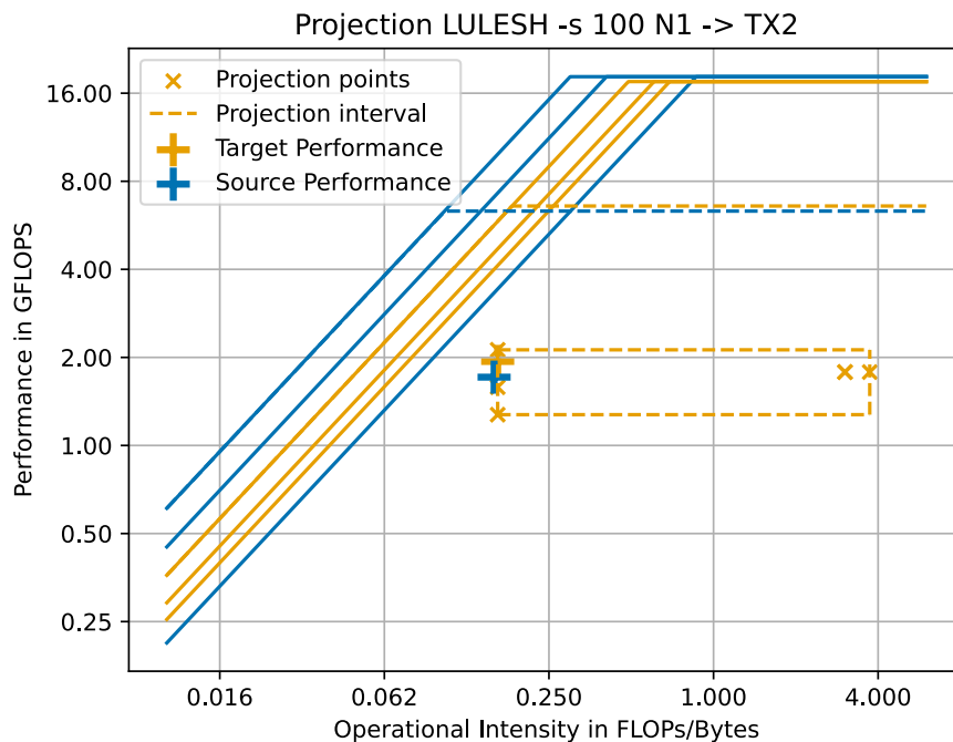
Figure 6.10: LULESH -s 100 N1 \rightarrow TX2 projection results.
