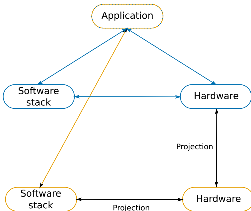
Figure 5.3: Projection approach between an accessible source and a future target triplet.
