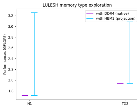
Figure 6.20: Exploration of introduction of HBM2 on LULESH
