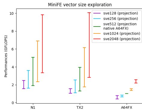
Figure 6.18: Exploration of different SVE vector sizes on MiniFE
