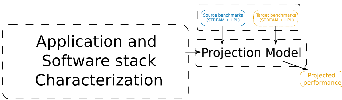
Figure 6.2: Hardware characterization through STREAM and HPL benchmarking. Source machine is in plain blue and target machine is in dotted yellow.
