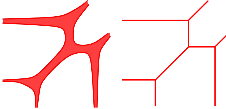
Figure 4.1: An amoeba in \mathbb{R}^2 , and the associated tropical limit.
