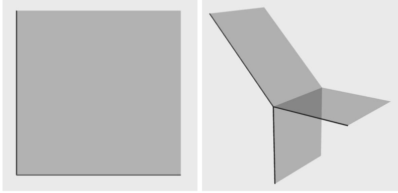
Figure 7.5: A depiction of the polyhedral complexes \gamma^\circ for two faces \gamma from Example 7.3.3.
