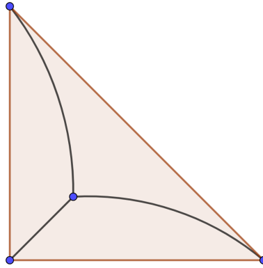
Figure 7.1: The tropical curve induced by the tropical polynomial " x + y + xy " in \mathbb{TP}^2 .
