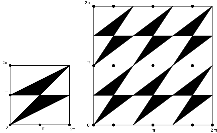
Figure 8.2: On the left, G \cdot \widetilde{\mathcal{C}_{X_{P_L}}} . On the right: the coamoeba \mathcal{C}_X in black and the zonotopes in white.
