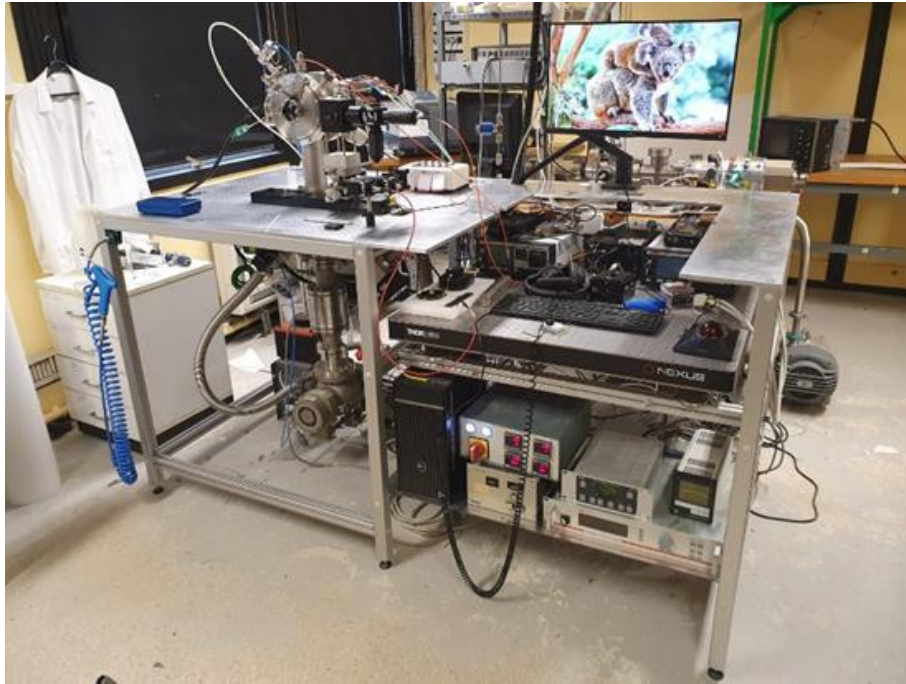
Figure 2-26: Retrofitted PECVD Reactor (left) with in-situ MPL & PL workstation (right).
