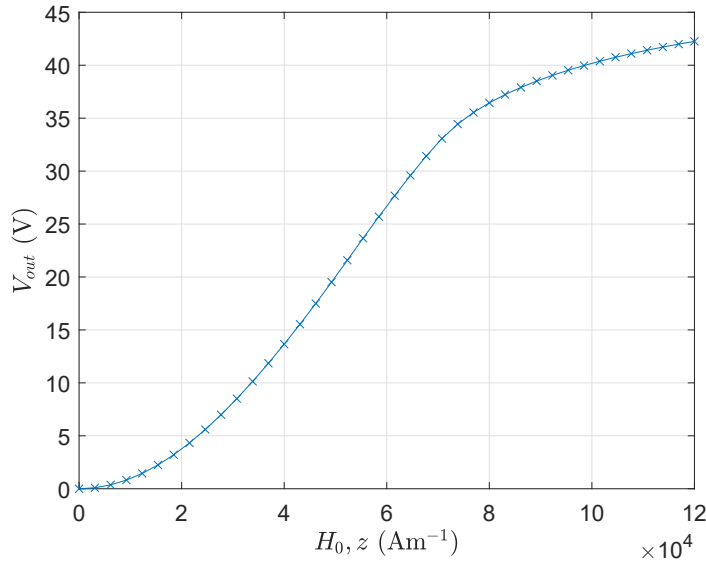
Figure 4.21: Output voltage of the three-layer ME composite with the invariants approach to magneto-mechanical coupled behavior
