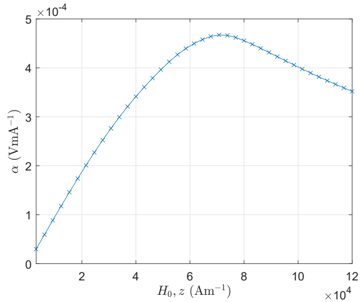
Figure 4.22: Output voltage of the three-layer ME composite with the invariants approach to magneto-mechanical coupled behavior
