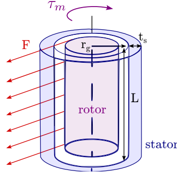
Figure 18: Motor geometric sketch
