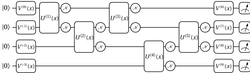
Figure 5.1: Example of a noisy quantum circuit on n = 4 qubits with two-qubit and single-qubit gates, parametrized by the input vector x \in \mathcal{X} . A pair of single-qubit noise channels \mathcal{N} follow each two-qubit gate. The circuit begins and ends with a layer of noiseless single-qubit gates. This model contains minimal assumptions on the circuit architecture, and it coincides with the one adopted in [DHJB21].
