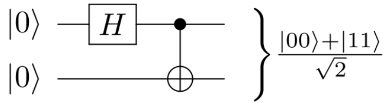
Figure 2.2: Quantum circuit to create the EPR pair.
