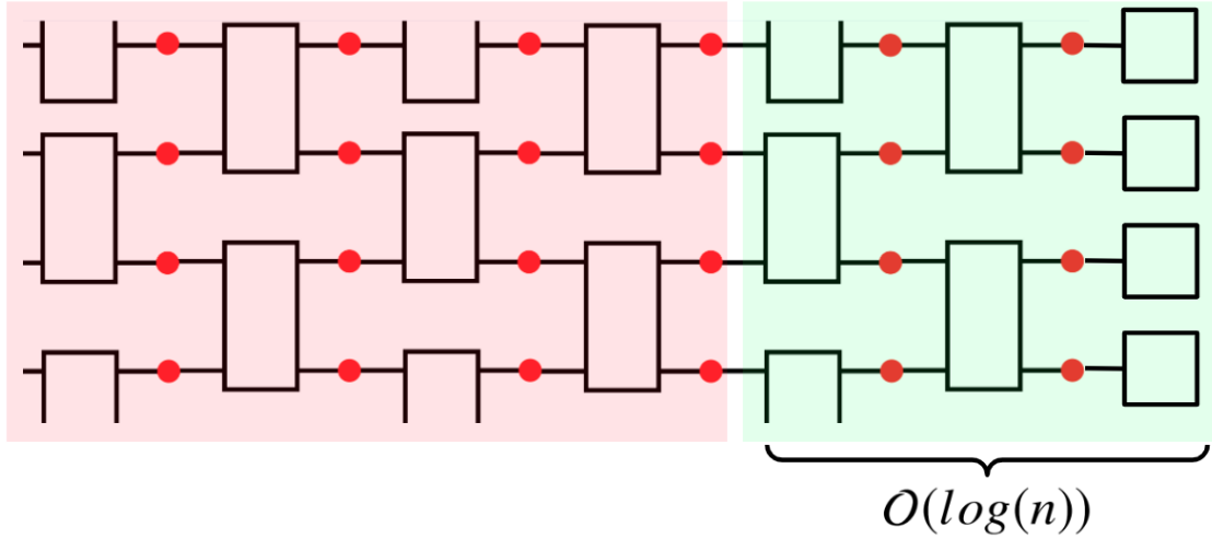
Figure 5.2: Here we provide a pictorial representation of the “effective depth” noisy circuit. We conjecture that the final state \rho(x) = \Phi_x(\rho_0) bears little information about the initial portion of the circuit. In the context of cost function-based variational machine learning, this also implies that the parameters encoded in this initial portion are not trainable.
