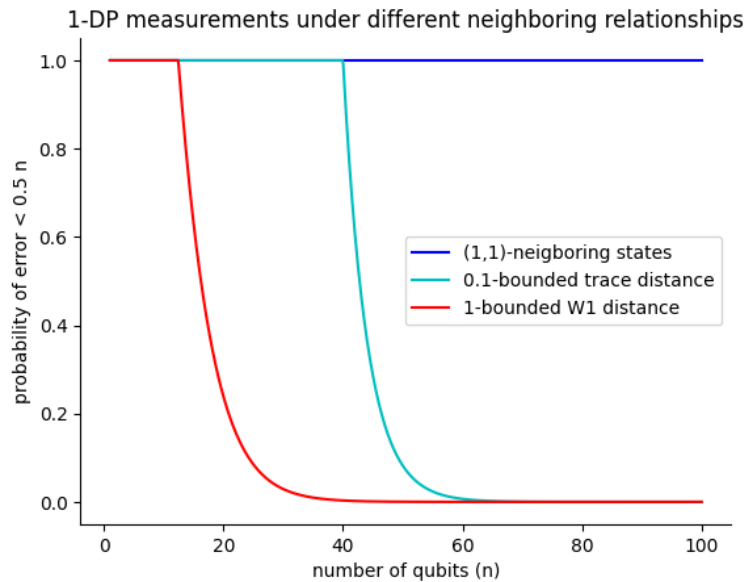
Figure 8.3: Upper bounds on the probability of achieving error lower than 0.5n for a measurement of \frac{1}{n} \sum_{i=1}^n Z_i on the state |1^n\rangle , for several neighboring relationships and various values of n . We assumed the input state undergoes a 1-DP channel.
