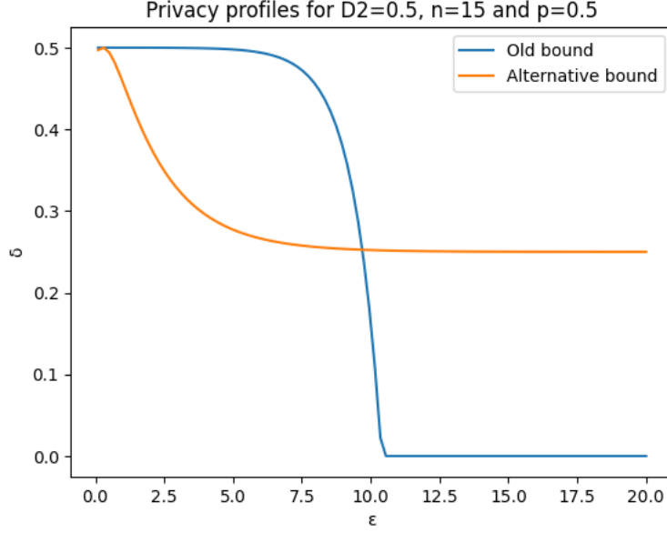
Figure 8.1: In this figure we compare the former upper bound from [HRF23] (Equation 8.30) with the novel upper bound provided in this section (Equation 8.31). We emphasise that each bound outperforms the other for some values of \epsilon . We assumed that the input state satisfy D_2(\rho \| I/2^n) \leq 0.5 , n = 15 and p = 0.5 . The upper bound on \tau is derived from \|\rho - \sigma\|_1 \leq \|\rho - I/2^n\|_1 + \|\sigma - I/2^n\|_1 \leq 2\sqrt{2D_2(\rho \| I/2^n)} , i.e. combining the triangle inequality and the Pinsker's inequality.
