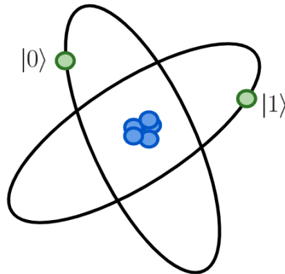
Figure 2.1: An atom with 2 electronic orbits, denoted as the states |0\rangle and |1\rangle . This 2-level system is a physical realization of the qubit.
