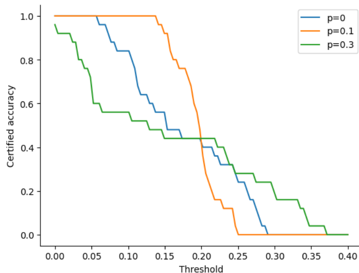
Figure 8.5: This plot contains the values of the certified accuracy estimated for various noise levels p and various attack thresholds \tau .
