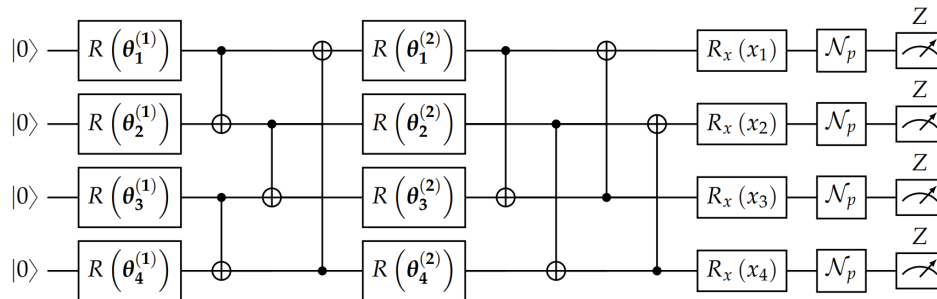
Figure 8.4: The parametric quantum circuit used in the simulation. We placed the encoding gates after the trainable gates in order to produce a (1, \tau) -neighboring-preserving encoding. The output state is measured according to the observable O = \frac{1}{8} \sum_{i=1}^4 (Z_i + 1) .
