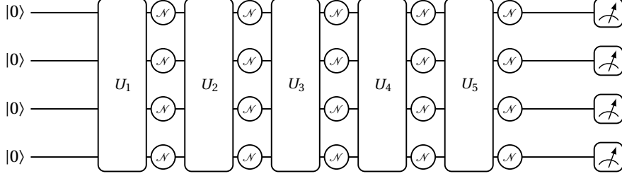
Figure 4.1: Example of a noisy quantum circuit on n = 4 qubits
