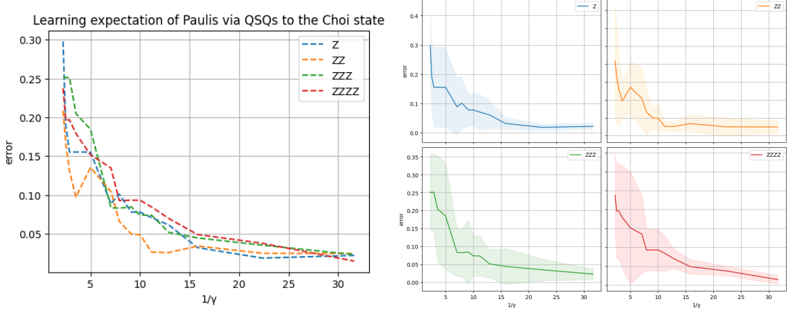
Figure 6.1: Average performance of the Goldreich-Levin algorithm implemented with quantum statistical queries to the Choi-Jamiolkowski state. We tested the algorithm on 10 random 4-qubit random unitaries, in predicting the absolute value of the outcome of Z observables on the unitary evolution of computational basis states. Each random unitary consists in 2 layers of Haar-random gates. We plotted the average error as a function of 1/\gamma , i.e. the inverse of the threshold of Algorithm 2. We set the tolerance of the quantum statistical queries as \gamma^2/4 .
