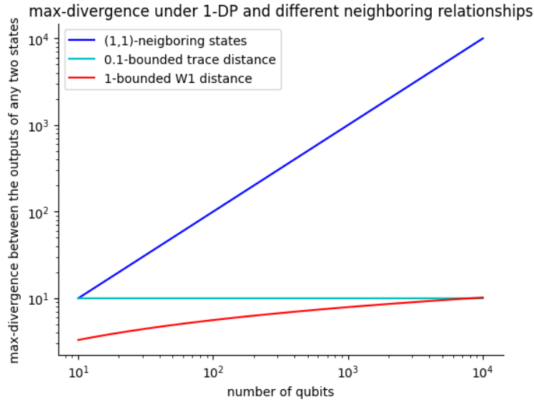
Figure 8.2: Upper bounds on the quantum max-relative entropy between any two states under 1-DP for several neighboring relationships and various values of n .
