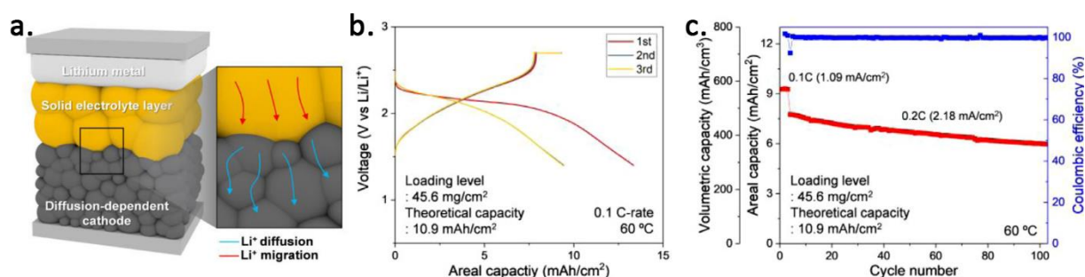
Figure 1.34. (a) Cell schematic, (b) galvanostatic cycling and (c) capacity retention of the \text{TiS}_2/\text{LPSCI}/\text{Li}^0 cell. Adapted from reference 118 .
