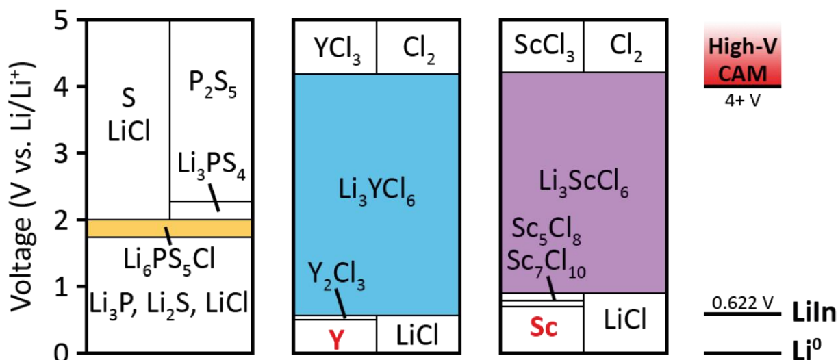
Figure 1.15. Calculated phase equilibria for (left to right) \text{Li}_6\text{PS}_5\text{Cl} , \text{Li}_3\text{YCl}_6 and \text{Li}_3\text{ScCl}_6 and potential of Li metal, LiIn alloy and high potential CAMs. Calculations based on first-principle calculations (DFT). Stable potential window of SEs are coloured and electronically conductive species are in red. Adapted from references 48,56,72 .
