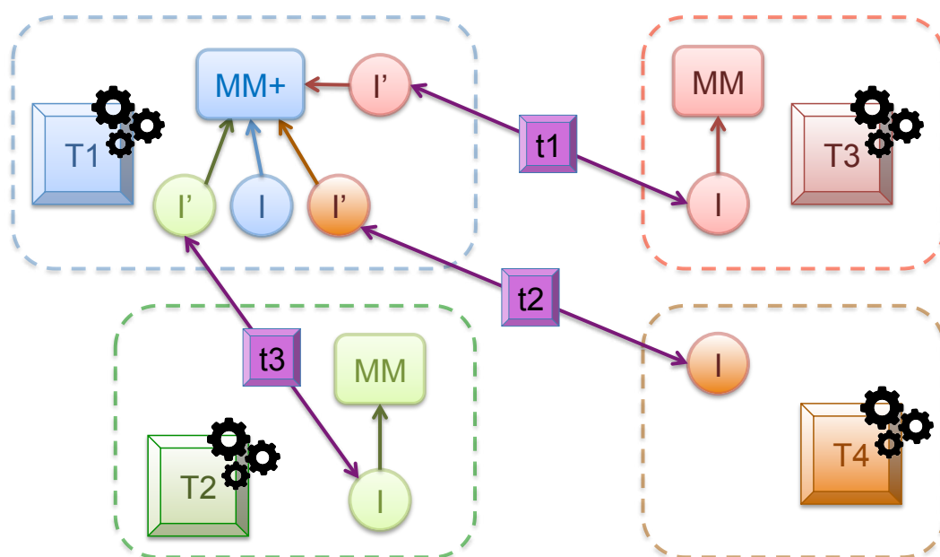
FIGURE 2.11 – L'approche "Unification"
