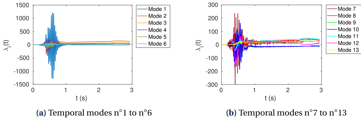
Figure 3.20 • Temporal PGD modes for the beam solicted with load 3 - a complex load
