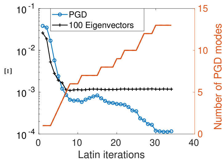
Figure 3.21 • Evolution of the error with LATIN iteration using an adaptive PGD basis or a fixed basis comprising the first 100 eigenmodes for the beam solicted with load 3 - a complex load
