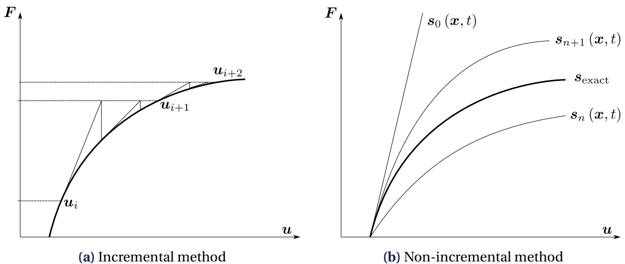
Figure 1.8 • Comparison between incremental and non-incremental schemes
