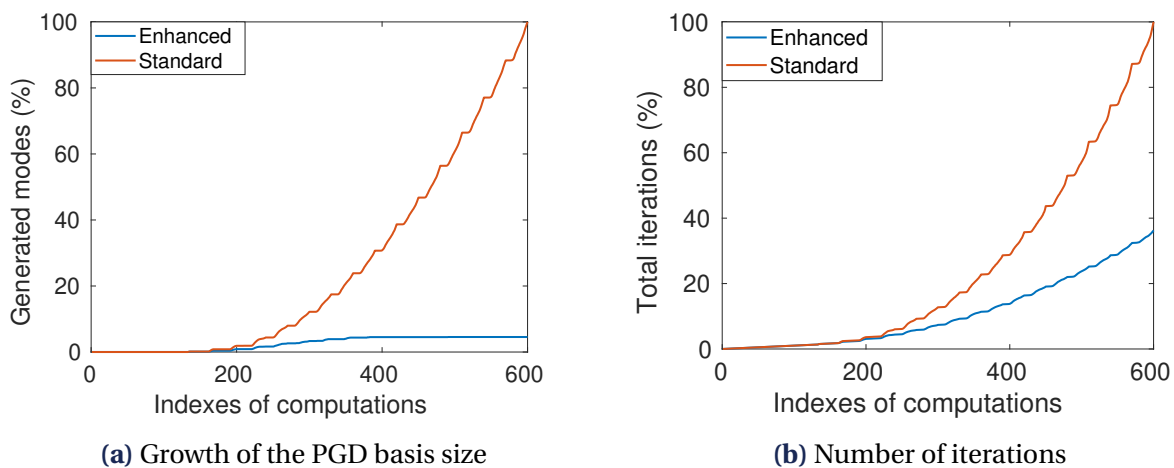
Figure 4.8 • Comparison of the standard method with the enhanced strategy.
