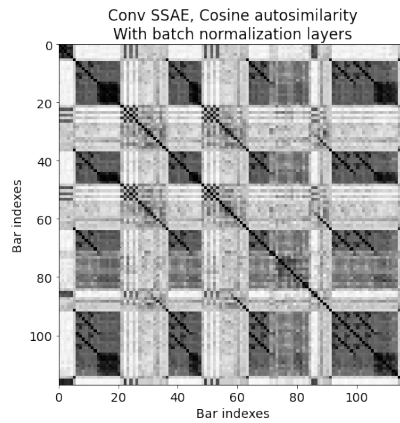
(d) Conv SSAE, with batch normalization layers.
