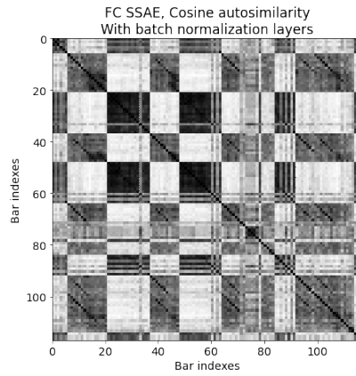
(b) FC SSAE, with batch normalization layers.
