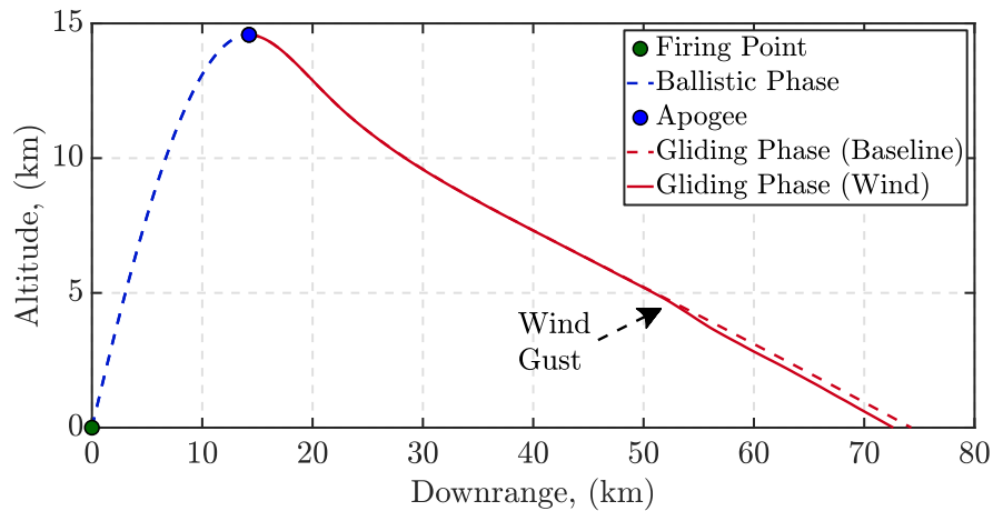
Figure 4.22: Polytopic simulations: trajectory performance.
