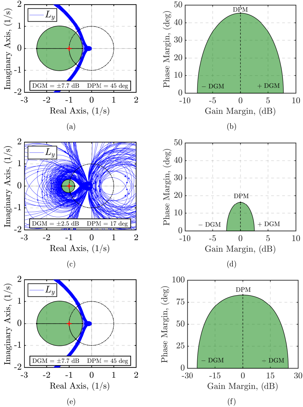
Figure 4.10: Grid-based output DKM Nyquist exclusion region and mutual GM/PM variation related to the: (a)-(b) \alpha channel, respectively; (c)-(d) q_{\text{dev}} channel, respectively; (e)-(f) \eta_{z,\text{dev}} channel, respectively.
