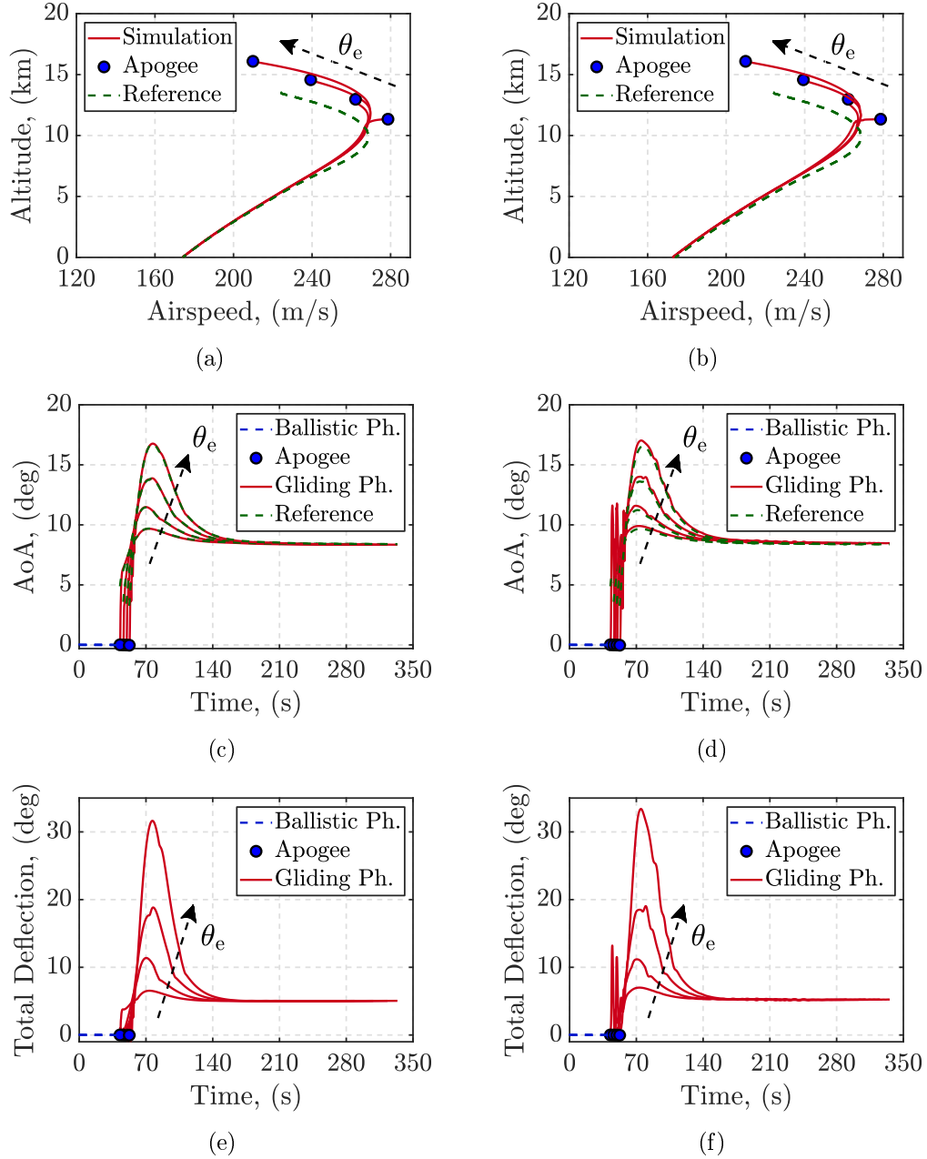
Figure 4.18: K_{PY} and K_{GR} baseline simulations: (a)-(b) V - h relation trajectories, respectively; (c)-(d) AoA trajectories, respectively; (e)-(f) canards total pitch deflection trajectories, respectively.
