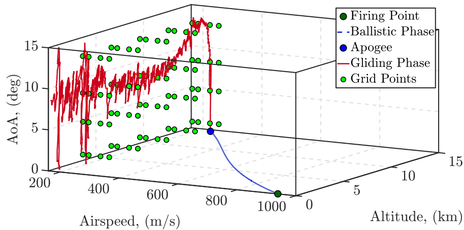
Figure 4.33: Grid-based perturbed simulation: 3D scheduling variables trajectory.
