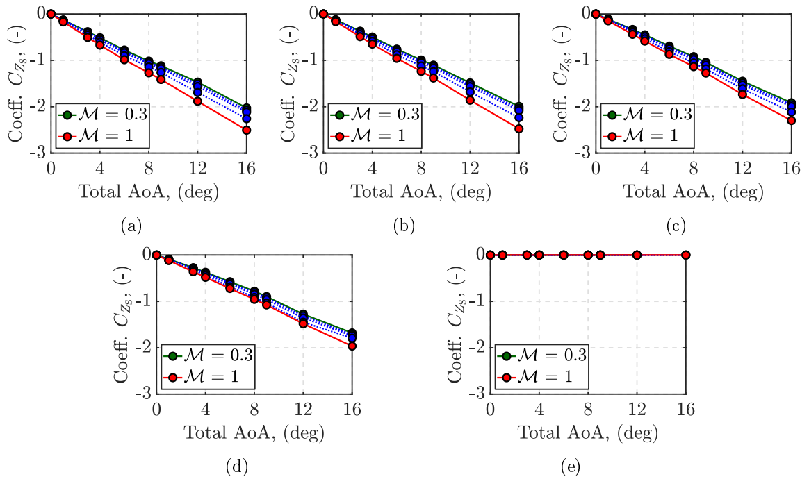
Figure A.3: CFD static vertical coefficient dataset, C_{Z_S} : (a) \phi' = 0 deg; (b) \phi' = 15 deg; (c) \phi' = 30 deg; (d) \phi' = 45 deg; (e) \phi' = 90 deg.
