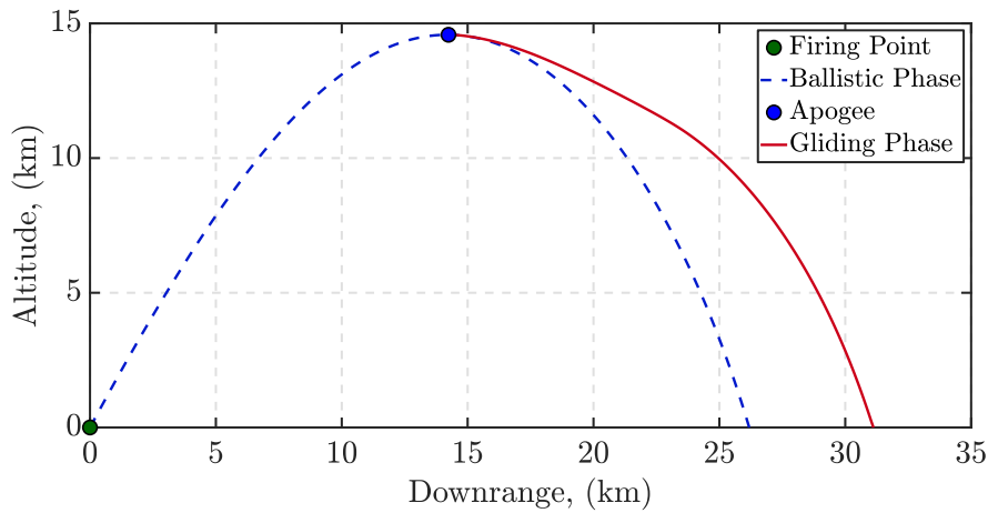
Figure 1.26: Ballistic simulations: trajectory performance comparison.
