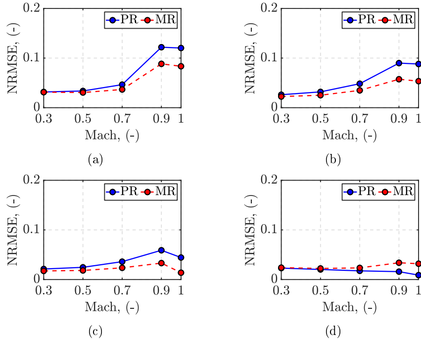
Figure A.8: C_{Y_S} interpolation NRMSE comparison at different flight conditions: (a) \phi' = 15^\circ ; (b) \phi' = 30^\circ ; (c) \phi' = 45^\circ ; (d) \phi' = 90^\circ .
