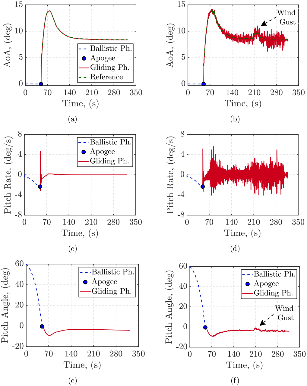
Figure 4.23: Polytopic simulations: (a)-(b) AoA nominal and perturbed trajectories, respectively; (c)-(d) pitch rate nominal and perturbed trajectories, respectively; (e)-(f) pitch angle nominal and perturbed trajectories, respectively.
