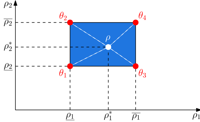
Figure 2.2: 2D polytope representation.
