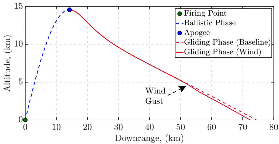
Figure 4.28: Grid-based simulations: trajectory performance.
