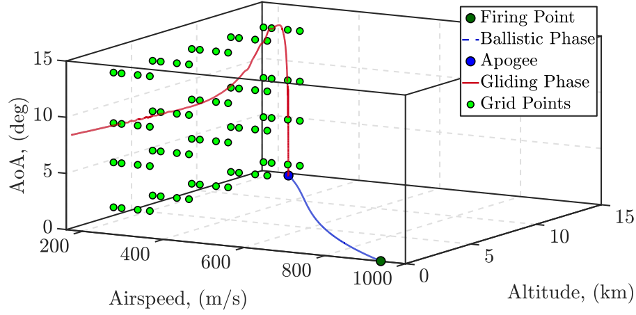
Figure 4.32: Grid-based nominal simulation: 3D scheduling variables trajectory.
