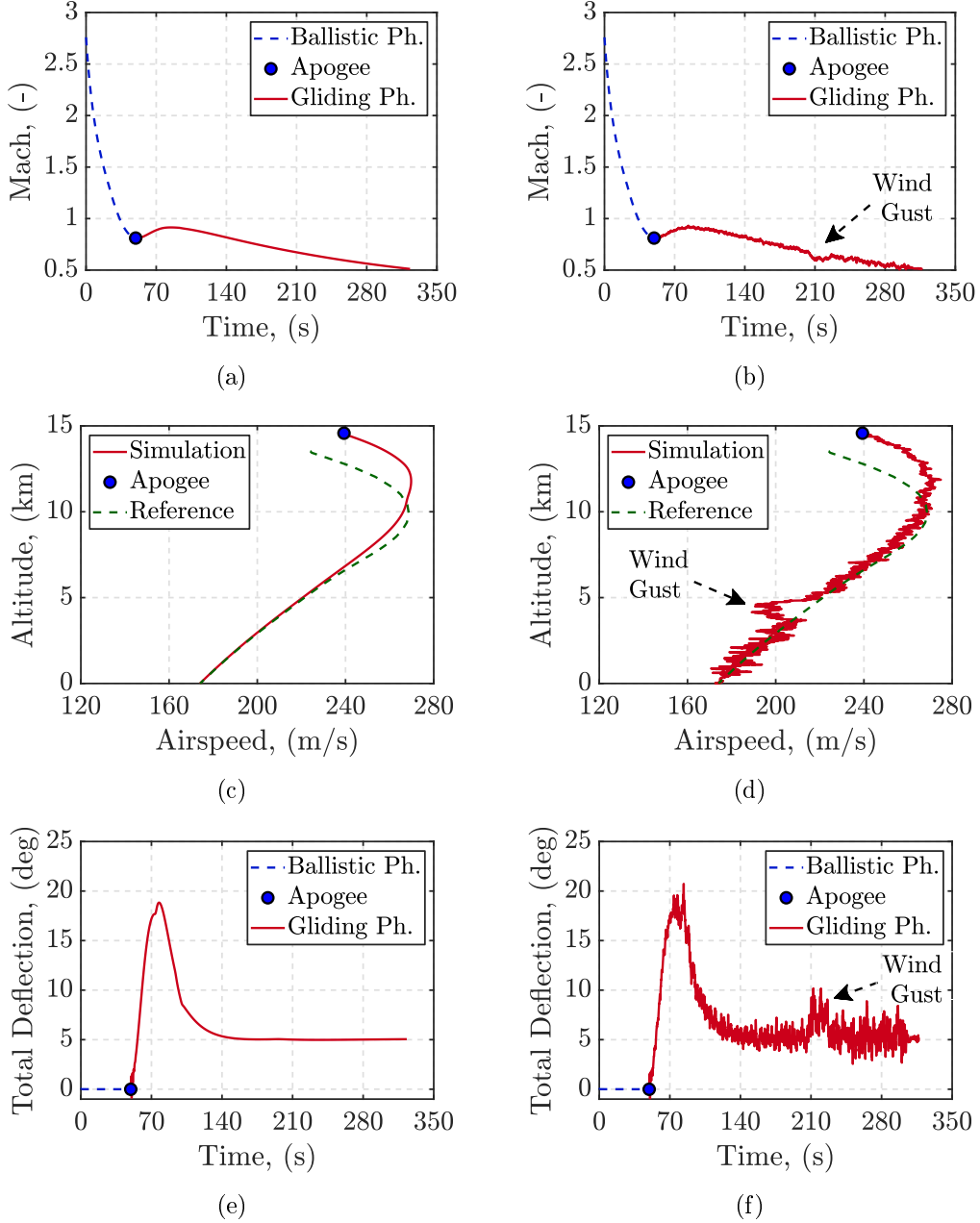
Figure 4.24: Polytopic simulations: (a)-(b) Mach nominal and perturbed trajectories, respectively; (c)-(d) V - h relation nominal and perturbed trajectories, respectively; (e)-(f) canards total pitch deflection nominal and perturbed trajectories, respectively.
