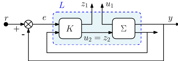
Figure 4.4: Loop-at-a-time disk margins computation scheme.
