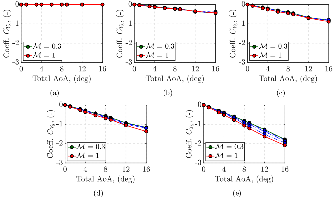
Figure A.2: CFD static lateral coefficient dataset, C_{Y_S} : (a) \phi' = 0 deg; (b) \phi' = 15 deg; (c) \phi' = 30 deg; (d) \phi' = 45 deg; (e) \phi' = 90 deg.
