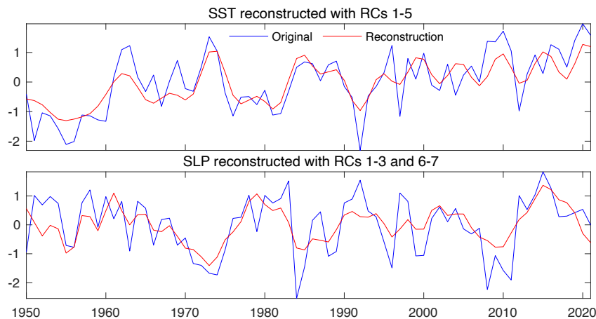
Figure 4.3: Example of original time series and reconstructed timeseries from 5 reconstructed components (trend, decadal and interannual modes explained in the text) for a random grid point for SST (above) and SLP (below).
