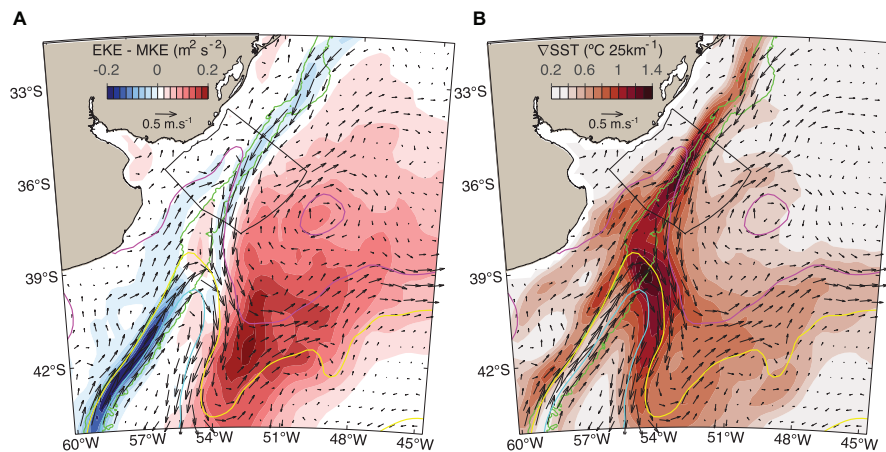
FIGURE 1 | Long-term mean conditions in the Southwestern Atlantic Ocean derived from satellite observations. Both panels show the mean surface geostrophic currents displayed as black arrows, the green lines show the 500 and 2,500 m isobaths, and the 0 m (cyan), 0.25 m (yellow), and 0.5 m (magenta) Absolute Dynamic Topography contours which indicate the retroflection of the main core of the Malvinas Current, the mean confluence position and the separation of the Brazil Current from the shelf-break, respectively. The black polygon delimits the Uruguayan Exclusive Economic Zone (EEZ). Background colors show the long-term daily mean of (A) eddy kinetic energy (EKE) minus mean kinetic energy (MKE) and (B) SST gradient.
