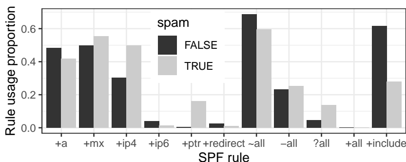
Figure 4.3: Usage proportion of SPF rules for benign and spamming domains
