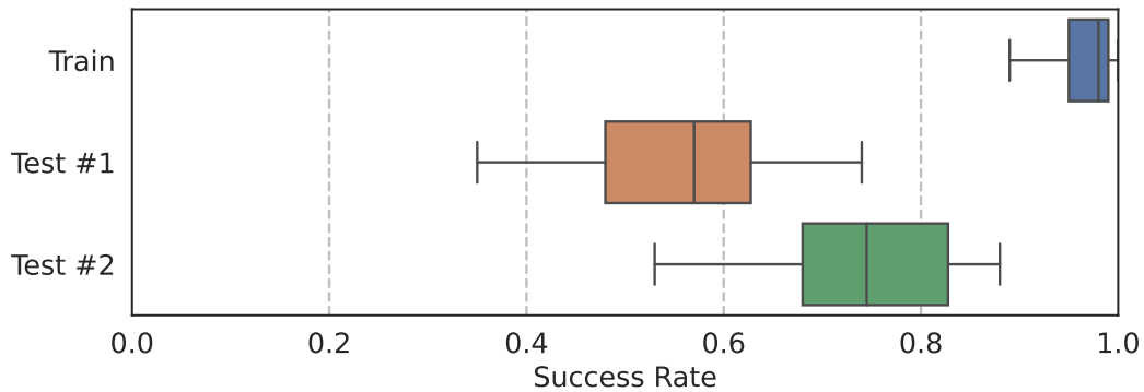
Figure 5.1 – Distribution of the success rate of a population of 100 trained policies. At the end of the training, we rollout trajectories with each policy on 3 different environments: Train (Ant, the one used for training), Test #1 (Ant with a Torso 20% bigger), Test #2 (Ant with legs 30% smaller). Success rate is averaged on 100 rollouts. The task remains the same for all environments (navigating from point A to B)
