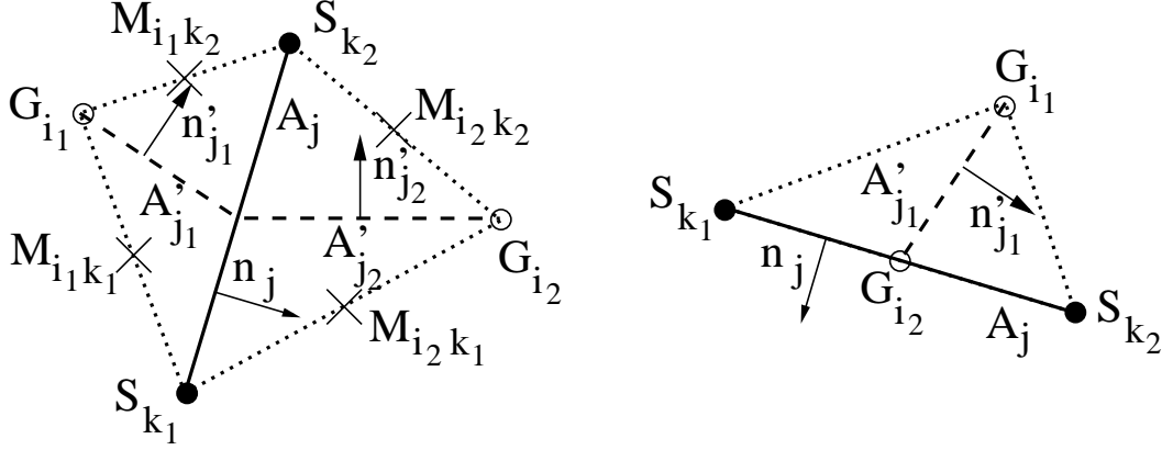
Figure 1.2: Notations for the inner diamond-cell (left) and a boundary diamond mesh (right).
