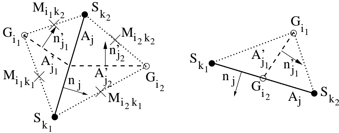
Figure 2.2: Notations for the inner diamond-cell (left) and a boundary diamond mesh (right).
