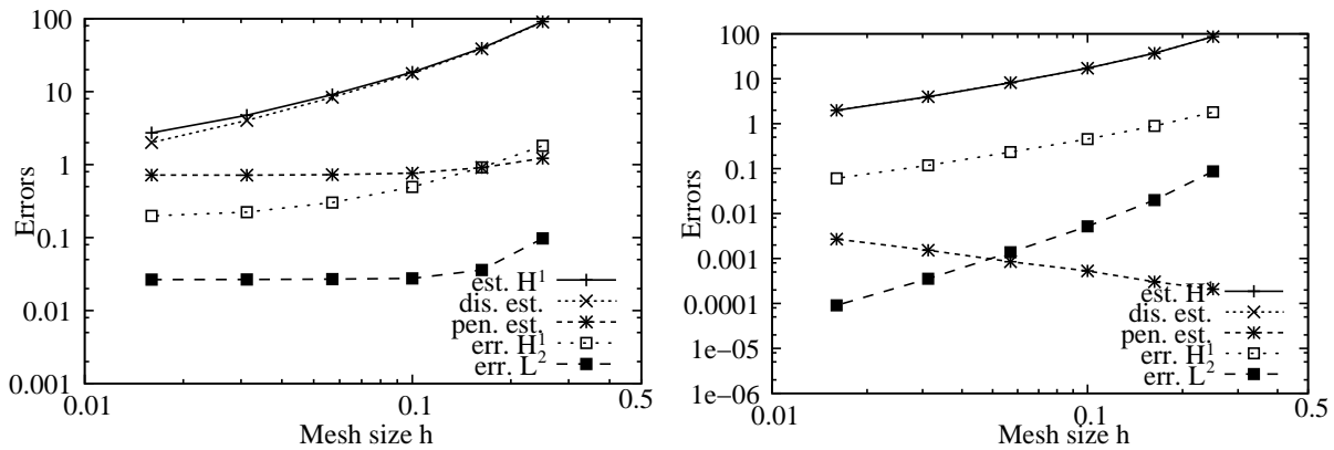
Figure 1.8: Actual errors in H^1(\Omega) and L^2(\Omega) norms, total estimator, discretization estimator and penalization estimator for the velocity. Left: \varepsilon = 10^{-3} , right: \varepsilon = 10^{-7} .
