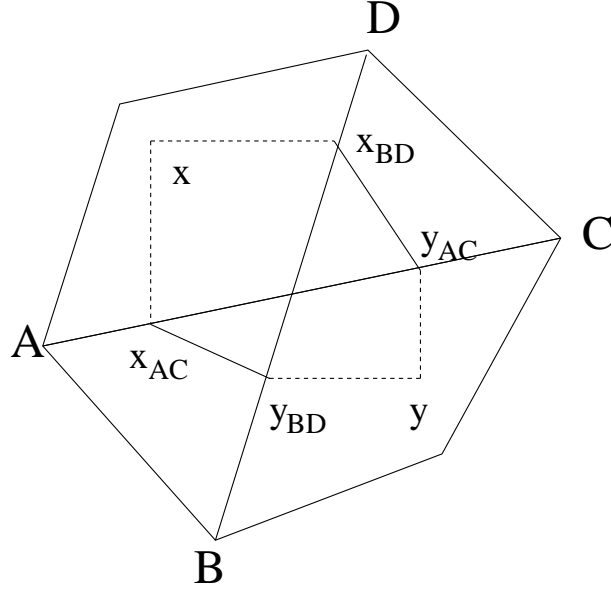
Figure 4.6: Notation for points A, B, C, D and points x_{AC}, x_{BD}, y_{AC}, y_{BD} .
