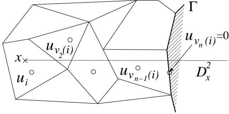
Figure 4.3: Straight line \mathcal{D}_x^2 intersecting primal cells from point x to the boundary.
