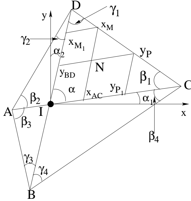
Figure 4.9: x_{AC}x_Mx_{M_1} intersects y_{BD}y_Py_{P_1} before it intersects DC .
