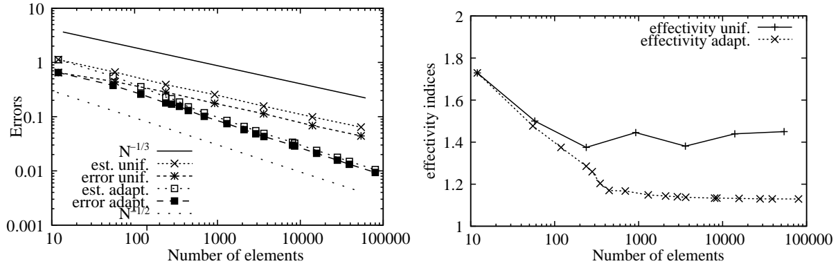
Figure 2.4: Estimated and actual errors for uniform and adaptive refinements (left) and effectivity indices for uniform and adaptive refinements (right) for H(x) = 1 + 1/(1 + x^2) .
