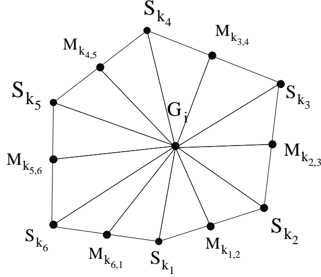
Figure 1.6: Notations of Prop. 1.32.
