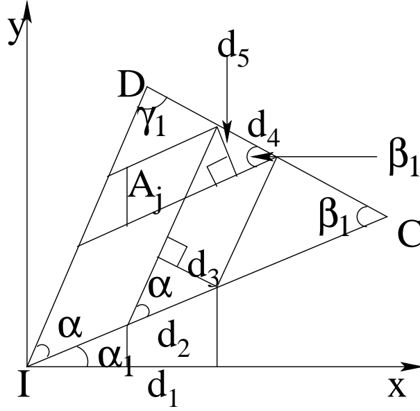
Figure 4.11: How to estimate the term \int_{x_I}^{x_C} \chi_j(x_M, x_{M_1}) dx_1 .
