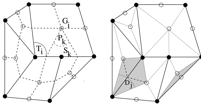
Figure 4.1: A nonconforming primal mesh and its associated dual mesh (left) and diamond-mesh (right).
