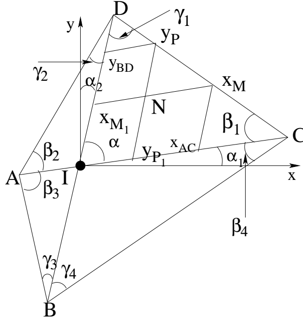
Figure 4.8: x_{AC}x_Mx_{M_1} intersects DC before it intersects y_{BD}y_Py_{P_1} .
