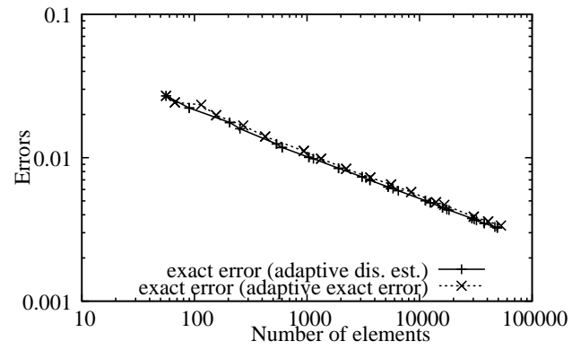
Figure 1.12: Exact errors in the adaptive process using the discretization estimator and exact error.
