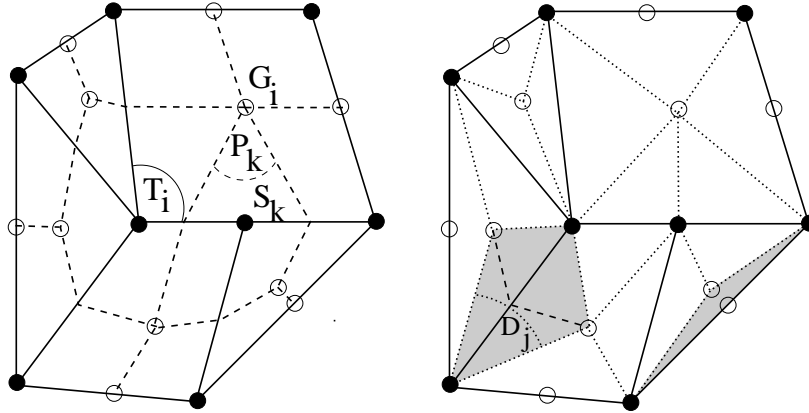
Figure 1.1: A nonconforming primal mesh and its associated dual mesh (left) and diamond mesh (right).
