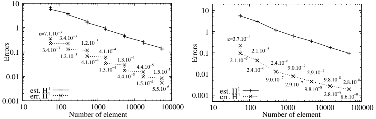
Figure 1.10: Actual errors in H^1(\Omega) and total estimator for the velocity. Left: \gamma = 1/10 , right: \gamma = 1/500 .
