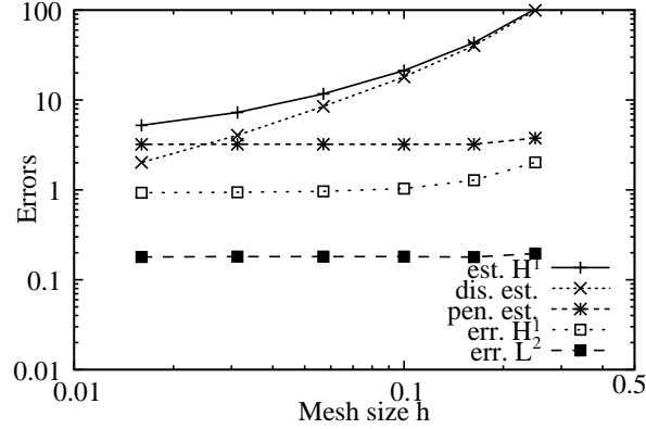
Figure 1.9: Actual errors in H^1(\Omega) and L^2(\Omega) norms, total estimator, discretization estimator and penalization estimator for the velocity for \varepsilon = 10^{-2} .
