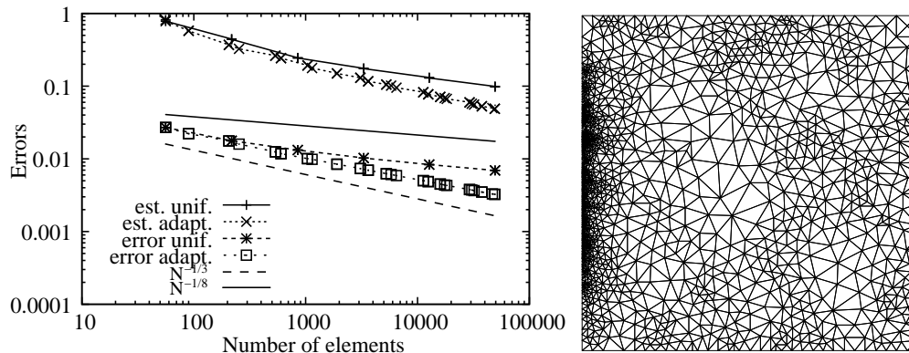
Figure 1.11: Estimated and exact errors in uniform/adaptive refinement (left) and an adaptive mesh (right).
