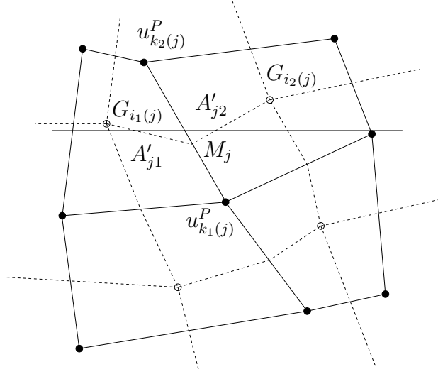
Figure 4.4: The straight line \mathcal{D}_x^2 intersects twice the boundary A'_{j1} \cup A'_{j2} of a non convex dual.
