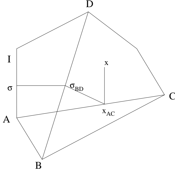
Figure 4.7: Notation for points A, B, C, D and points x_{AC} , \sigma_{BD} .
