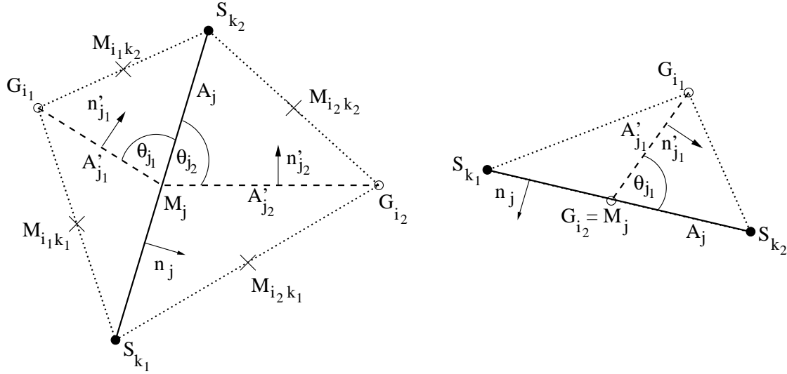
Figure 4.2: Notations for the inner diamond-cell (left) and a boundary diamond mesh (right).
