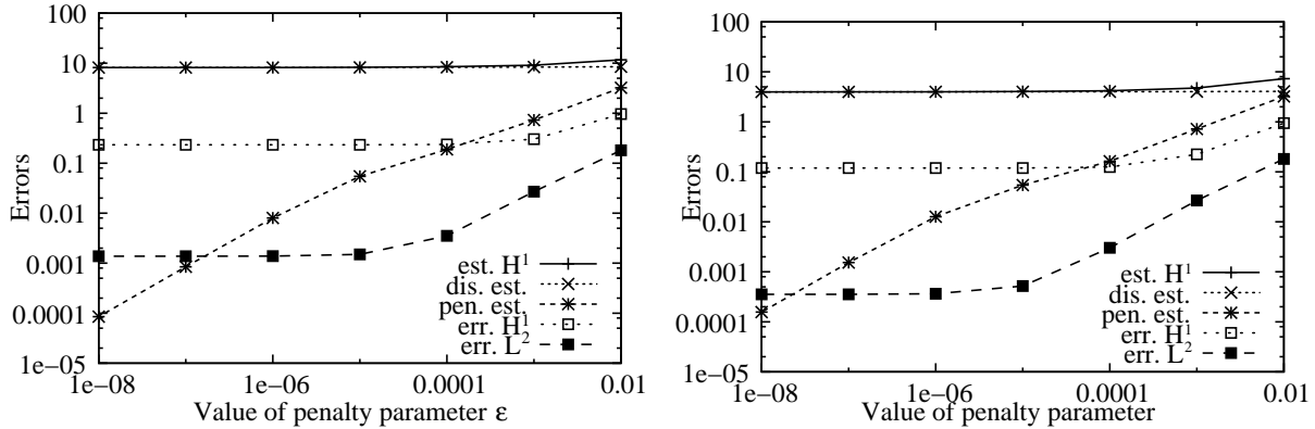
Figure 1.7: Actual errors in H^1(\Omega) and L^2(\Omega) norms, total estimator, discretization estimator and penalization estimator for the velocity. Left: h = 5.69 \times 10^{-2} , right: h = 3.125 \times 10^{-2} .
