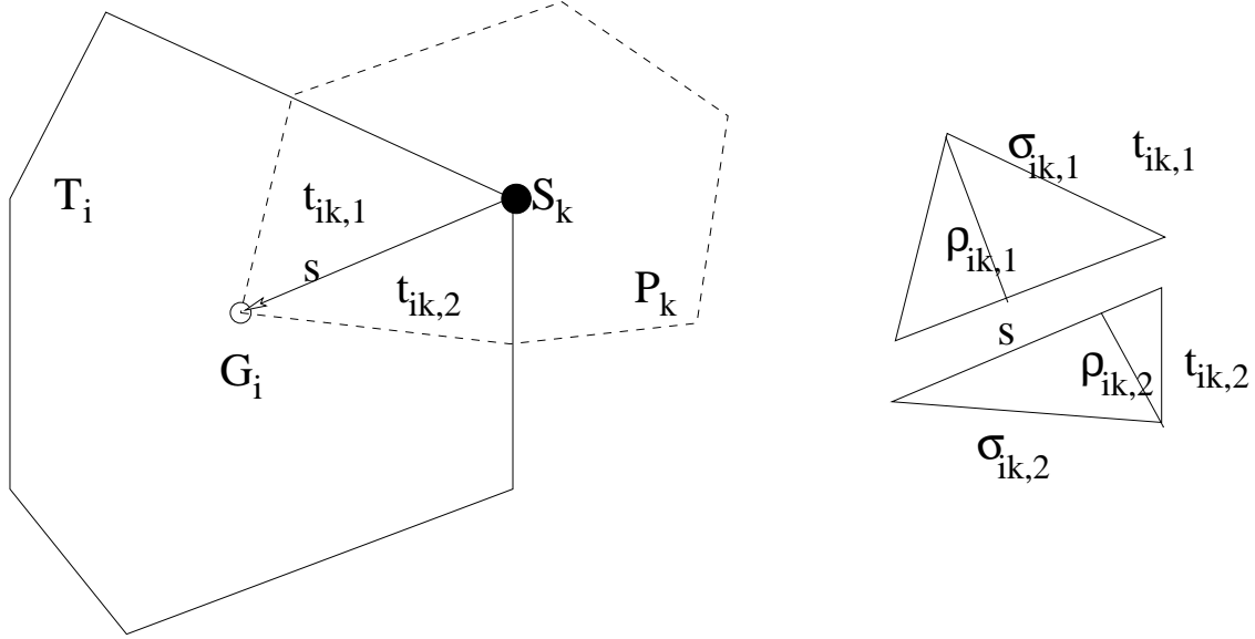
Figure 1.4: For each cell T_i and each vertex S_k of T_i , T_i \cap P_k is split in two triangles t_{ik,1} and t_{ik,2} .
