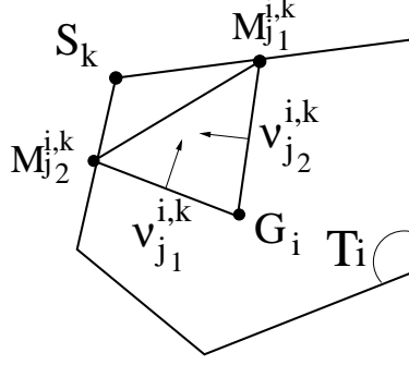
Figure 2.3: Notations for the triangle G_i M_{j_1}^{i,k} M_{j_2}^{i,k} .
