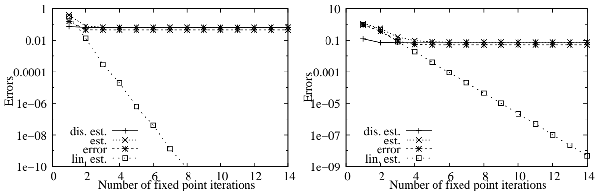
Figure 2.5: Total error, total estimator, discretization and linearization estimators as a function of the fixed point iteration. Left: H(x) = 1 + 1/(1 + x^2) and right: H(x) = 2 + \sin(10x) .
