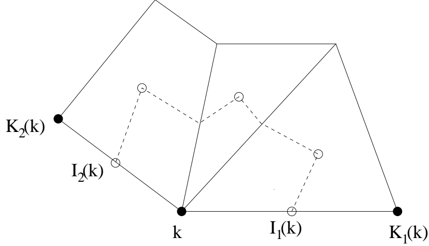
Figure 1.3: Notation for a boundary dual cell in formula (1.22).
