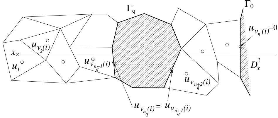
Figure 4.5: Straight line D_x^2 intersecting primal cells from point x to the boundary through internal boundary \Gamma_q .
