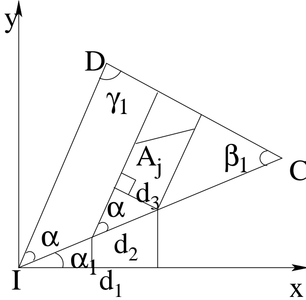
Figure 4.10: How to estimate the term \int_{x_I}^{x_C} \chi_j(x_{AC}, x_M) dx_1 .
