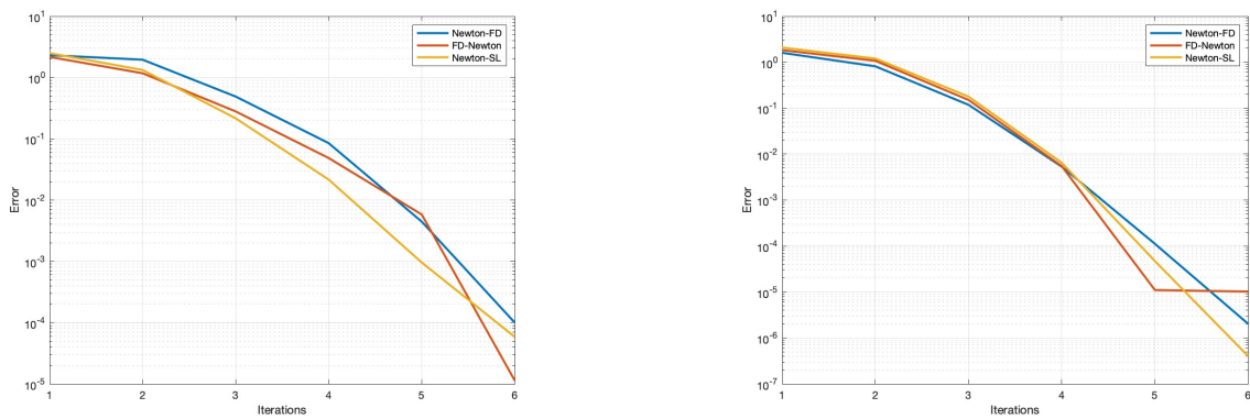
(a) \|m^{n+1} - m^n\|_\infty
