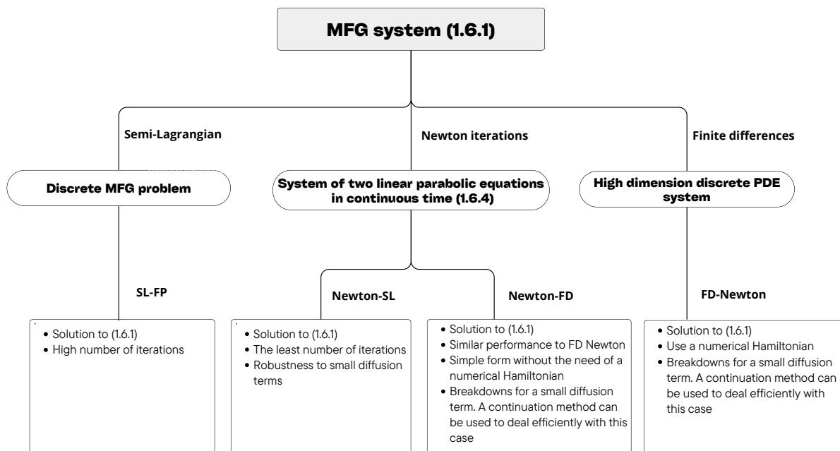
Figure 1.4: Solving the MFG system (1.6.1).
