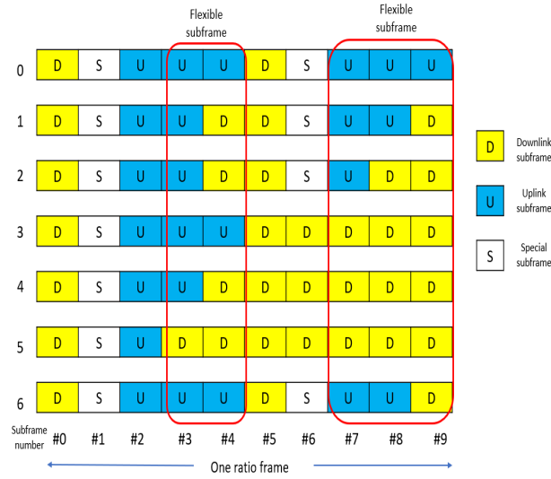
Figure 1.1: Dynamic TDD DL/UL configurations
